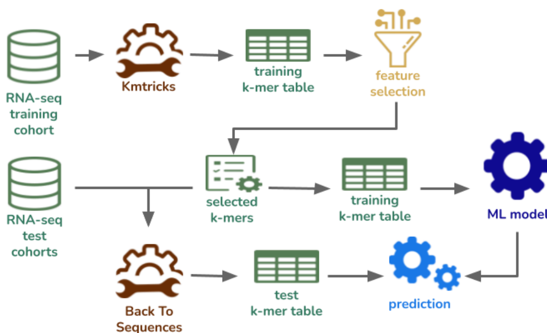
Figure A11. Pipeline to training and prediction for RNA-seq data.
