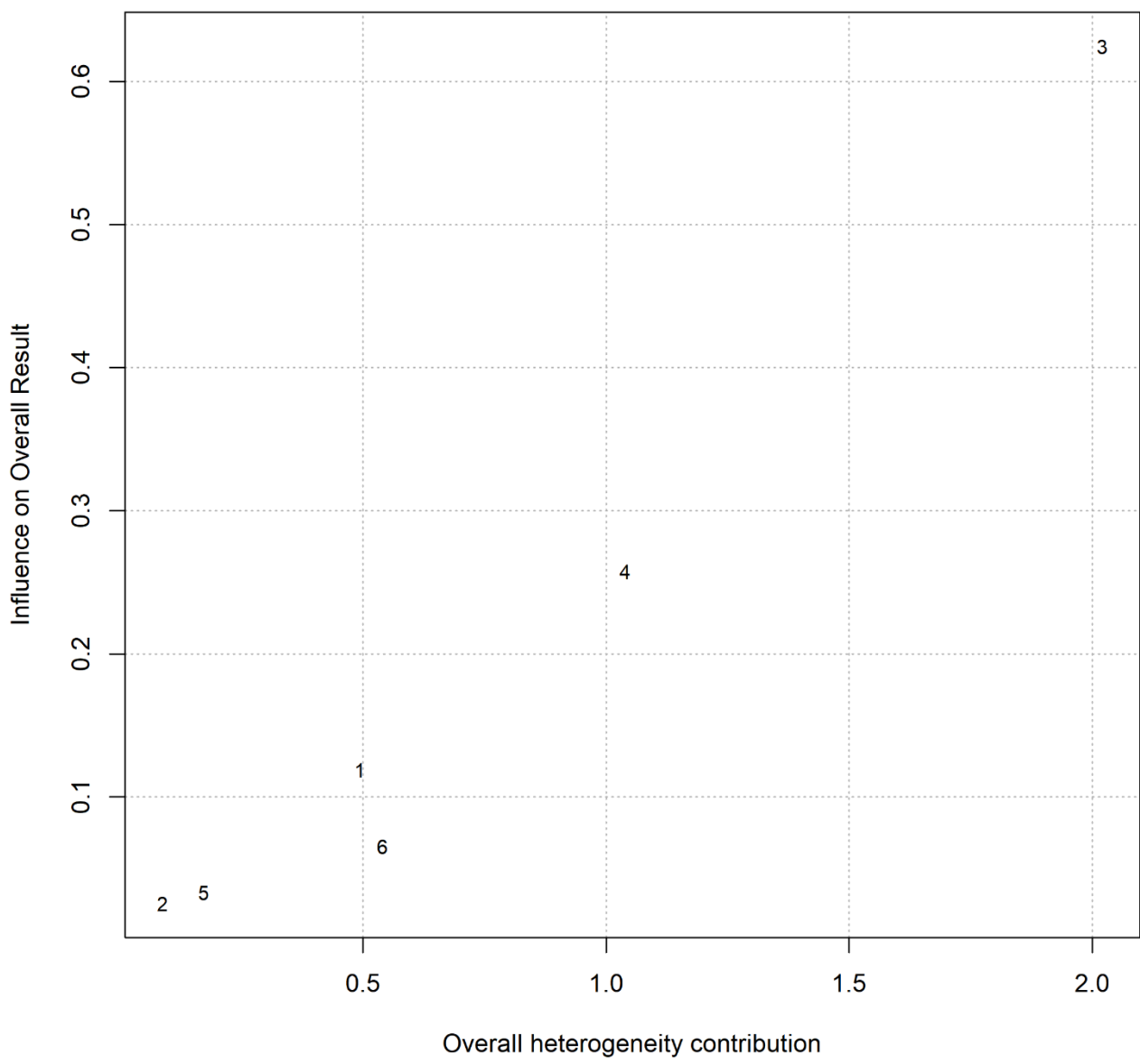
Figure S2. The Baujat plot summarizes the contribution of each study on the meta-analysis heterogeneity considering pre to follow-up craving scores as the outcome measure. On the x-axis, the overall heterogeneity as measured by Cochran’s QQ is displayed, whereas on the y-axis, the influence on the pooled effect size is represented.
