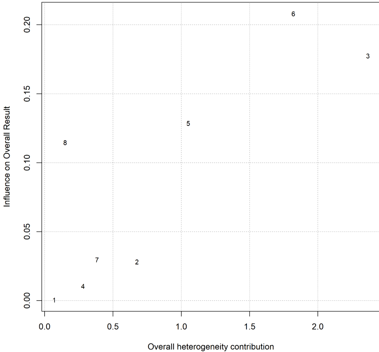
Figure 5. The Baujat plot summarizes the contribution of each study on the meta-analysis heterogeneity, considering pre- to post-craving scores as the outcome measure in a subgroup of studies including a sham/control condition. On the x-axis, the overall heterogeneity as measured by Cochran's QQ is displayed, whereas on the y-axis, the influence on the pooled effect size is represented.
