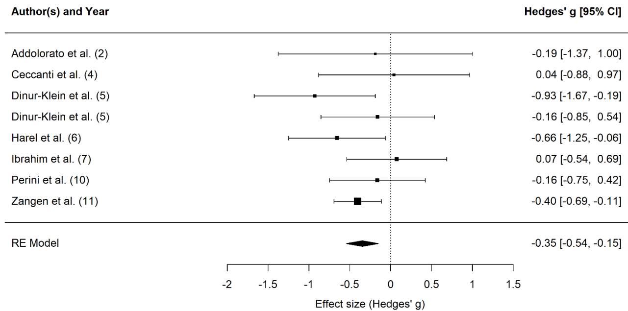
Figure 4. The forest plot summarizes the effect sizes of the dTMS on craving scores in a subgroup of studies including a sham condition. CI = confidence interval.
