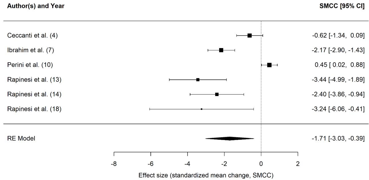
Figure S1. The forest plot summarizes the effect sizes of the dTMS intervention on craving scores at follow-up. CI = confidence interval.
