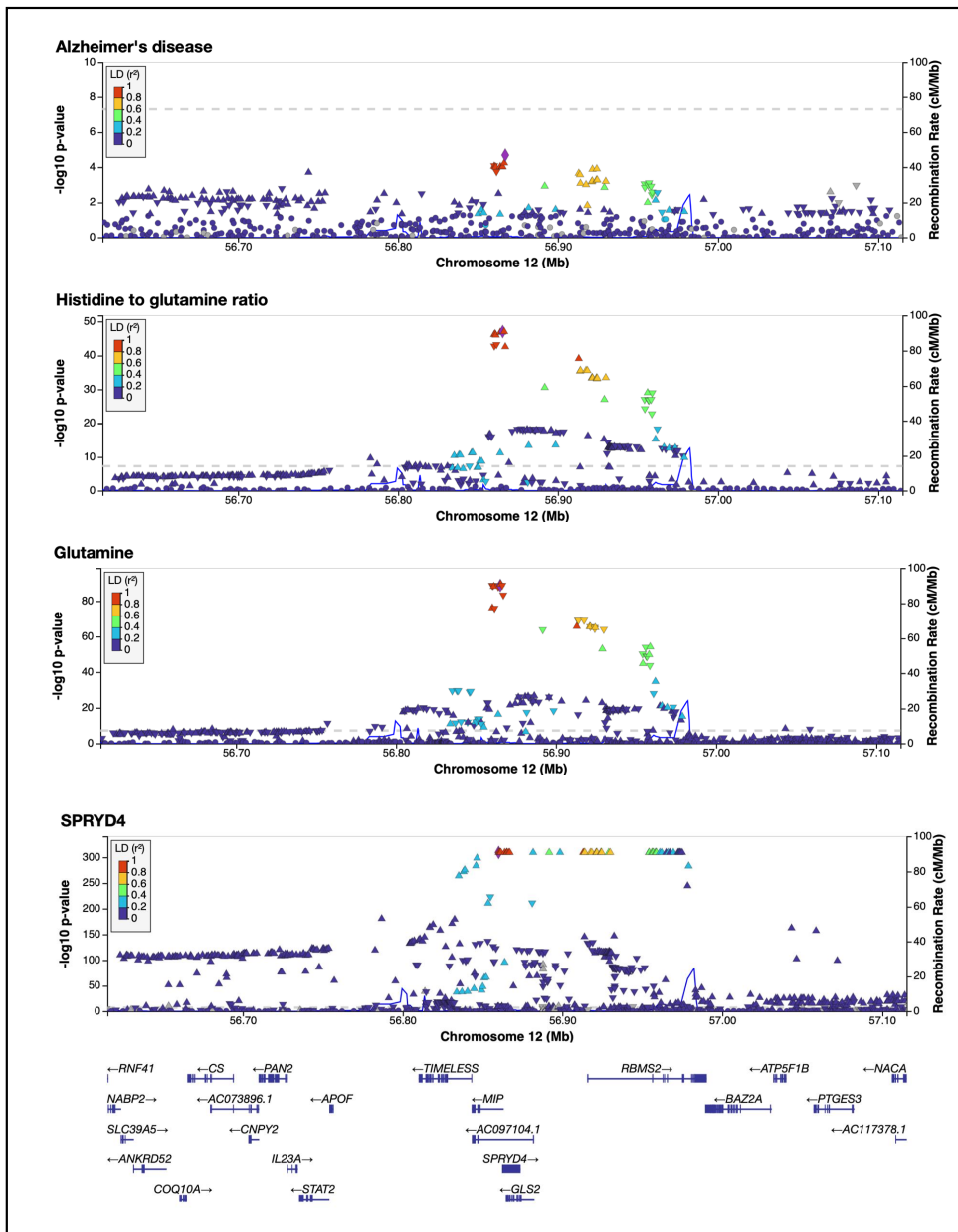
574 Figure 4: LocusZoom plots of the colocalising region ( PPH_4 \geq 0.8 ) chr12: 56615338-57115338 for 575 Alzheimer's disease, the ratio of histidine to glutamine, glutamine, and SPRYD4 expression.
