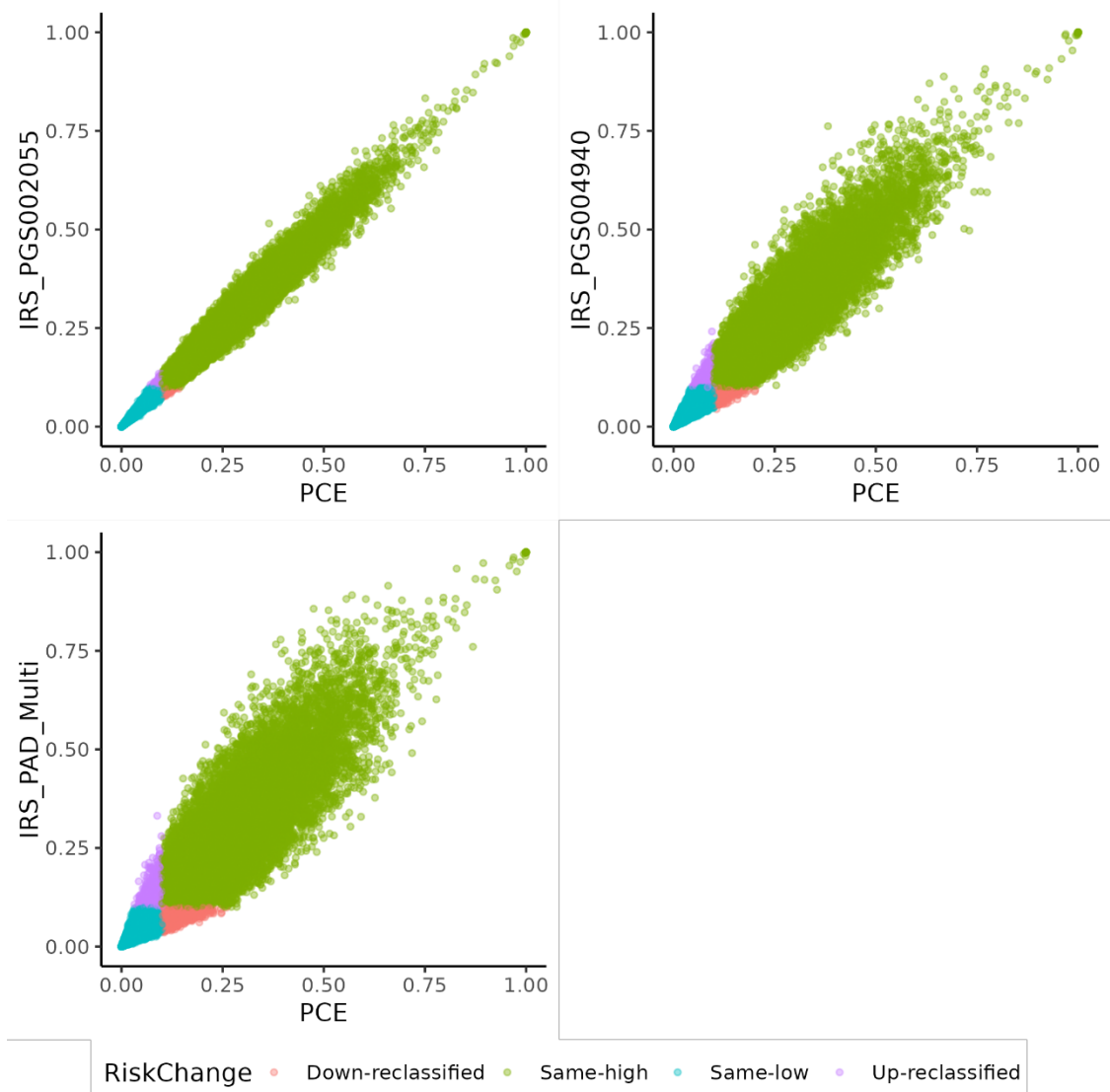
53 Figure S11. Net reclassification plots for each IRS based on each PRS for PAD and integration with the clinical PCE for 10-year clinical risk estimates with a threshold of > 10% 54 representing high risk. Blue represents same category low risk, purple represents up-reclassified risk, pink represents down-reclassified risk, and green represents same category 55 high risk.
