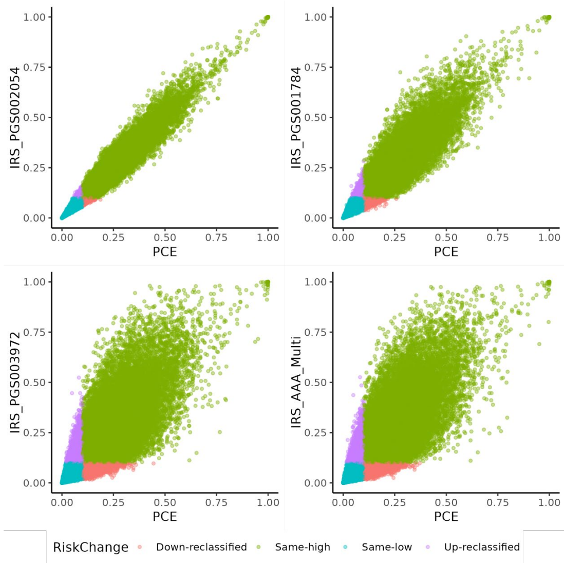
45 Figure S9. Net reclassification plots for each IRS based on each PRS for AAA and integration with the clinical PCE for 10-year clinical risk estimates with a threshold of > 10% 46 representing high risk. Blue represents same category low risk, purple represents up-reclassified risk, pink represents down-reclassified risk, and green represents same category 47 high risk.
