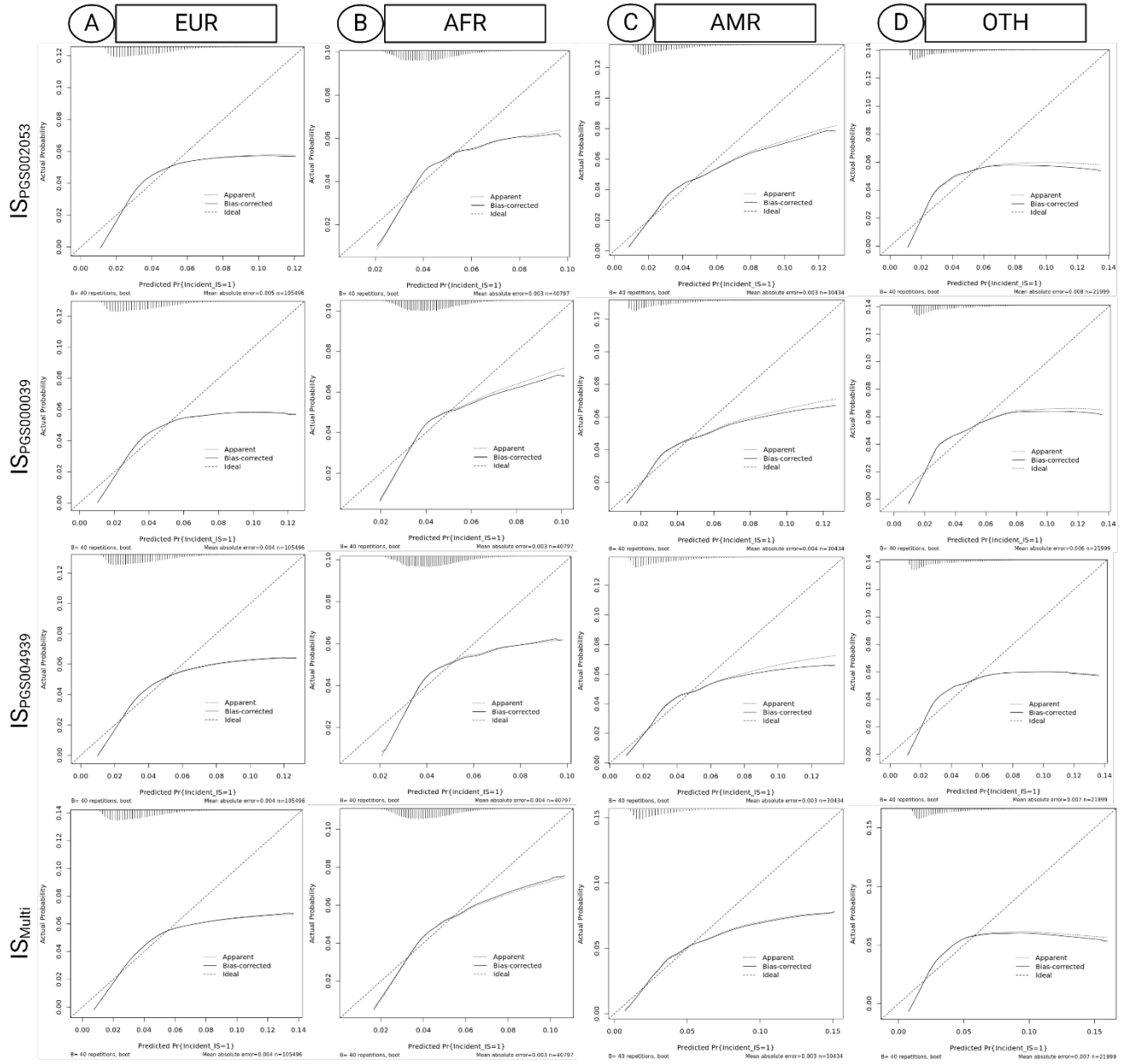
29 Figure S5. Calibration of PRS for IS adjusted for age and sex with predicted probability on the x-axis and actual probability on the 30 y-axis for European (EUR), African (AFR), Admixed American (AMR), and Other (OTH) genetic ancestry groups. Distribution of the 31 cases is shown in the top left corner of each plot.
