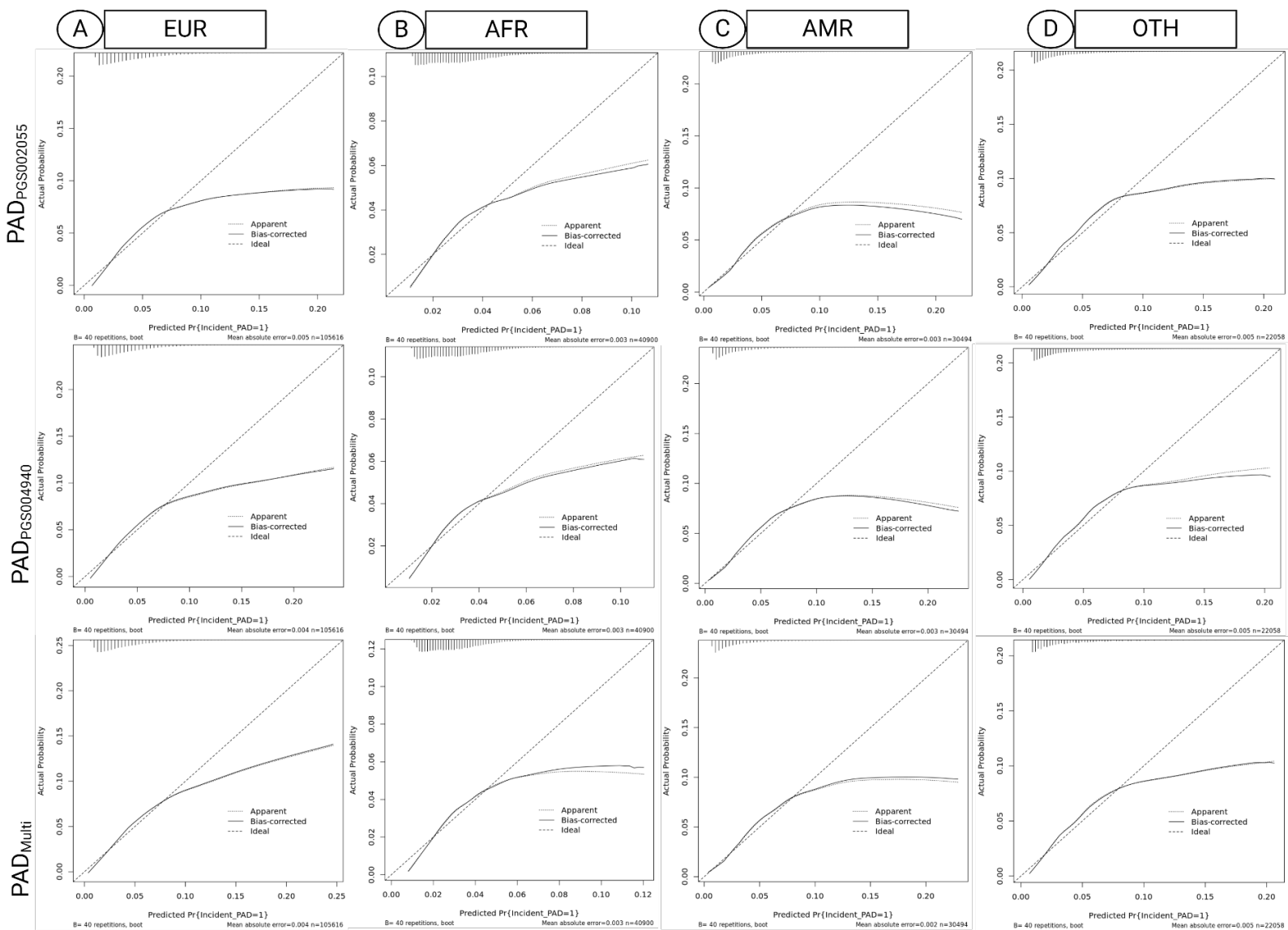
37 Figure S7. Calibration of PRS for PAD adjusted for age and sex with predicted probability on the x-axis and actual probability on the y-axis for European (EUR), African (AFR), 38 Admixed American (AMR), and Other (OTH) genetic ancestry groups. Distribution of the cases is shown in the top left corner of each plot.
