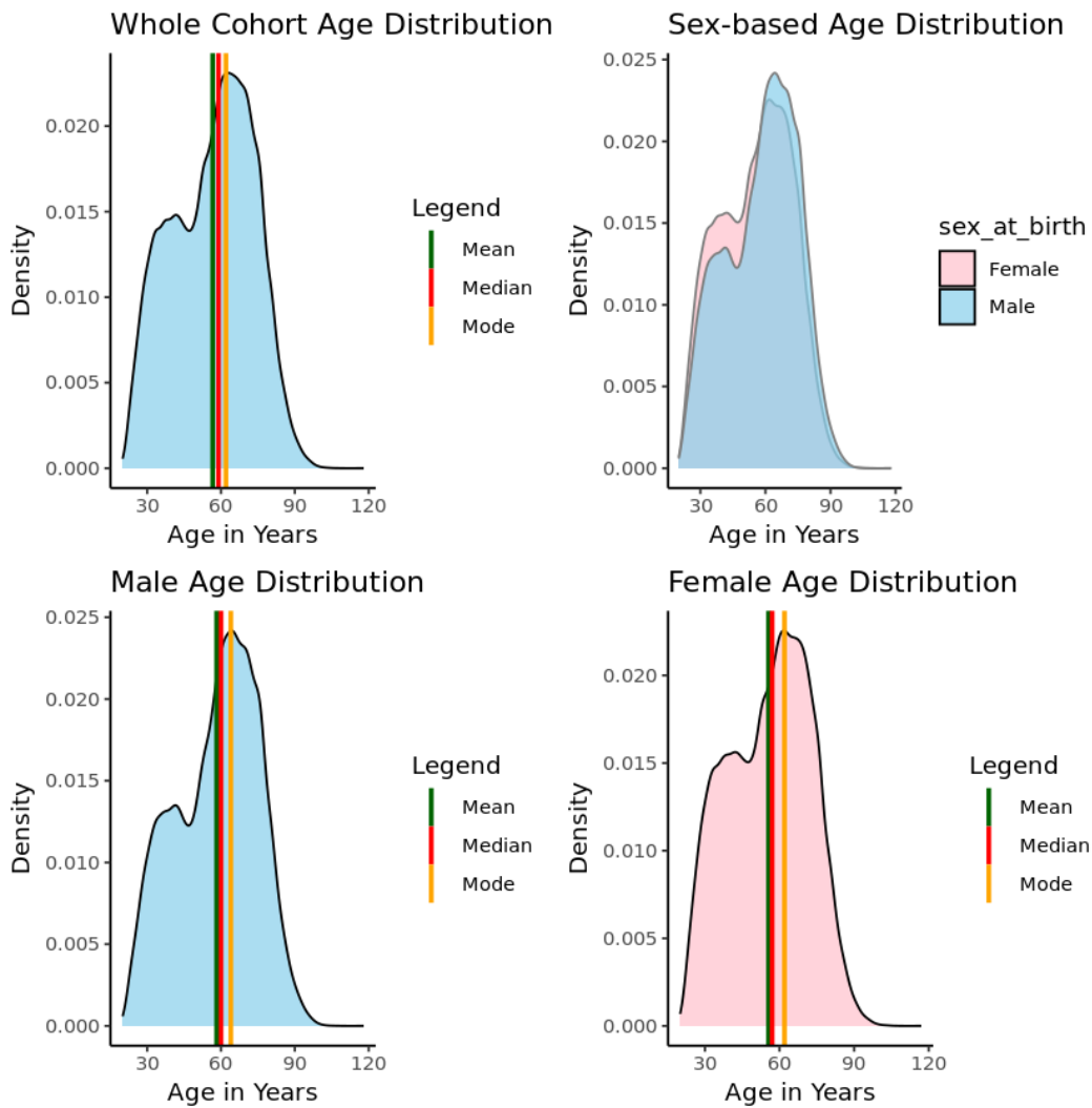
9 10 Figure S1. Age distribution a.) with mean, median, and mode across the whole ASCVD validation cohort, b.) comparing sex at 11 birth designations overlayed, and for c.) male and d.) female individuals in the cohort.
