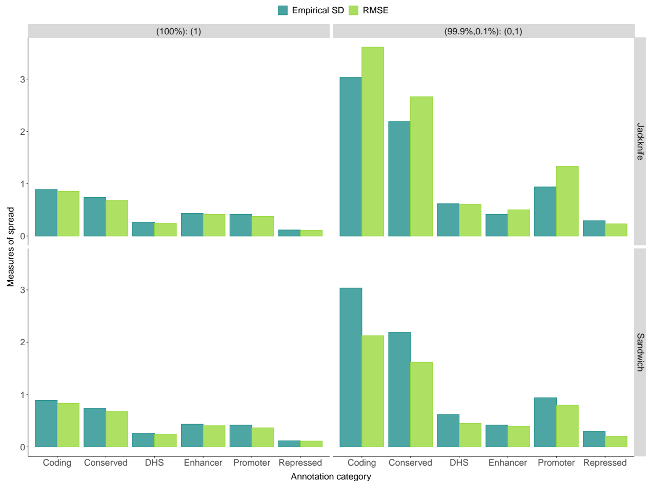
Supplementary Figure 8. Standard error calibration using the jackknife vs. the sandwich estimator. The column panel corresponds to different mixture components for generating the true causal effect sizes; the row panel corresponds to different SE estimators. Root mean square error (RMSE) is computed as the square root of the sum of the square SE divided by the number of experiments (100). Similarity between the empirical SD and the RMSE indicates good calibration.
