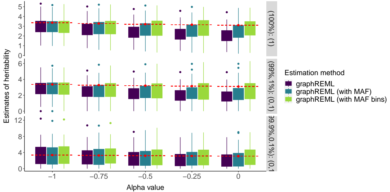
Supplementary Figure 6. Robustness of enrichment estimates under model mis-specifications: varying frequency-dependent architecture. Summary statistics are directly simulated based on the LDGM precision matrices on chromosome 1 from the Europeans in 1000 Genome ( p = 513,012, n = 100,000 ). Row panels represent different genetic architectures or mixture of causal effects, denoted as (component weights): (variance of the normal components). For example, (99%, 1%): (0,1) signifies that 99% of the SNPs are null and 1% of markers have their effect sizes drawn from N(0, 1) . X-axis correspond to different frequency-dependent architectures. The ALpha value determines the strength of the dependency 1 . For example, \alpha = -1 corresponds to the GCTA model and \alpha = -0.25 corresponds to the LDAK model. The red dashed lines represent the true heritability value of 0.1. graphREML: estimation without inclusion of any MAF-related annotations; graphREML (with MAF): estimation including MAF as a single continuous annotation; graphREML (with MAF bins): estimation that accounts MAF via 10 binary annotations for the 10 deciles.
