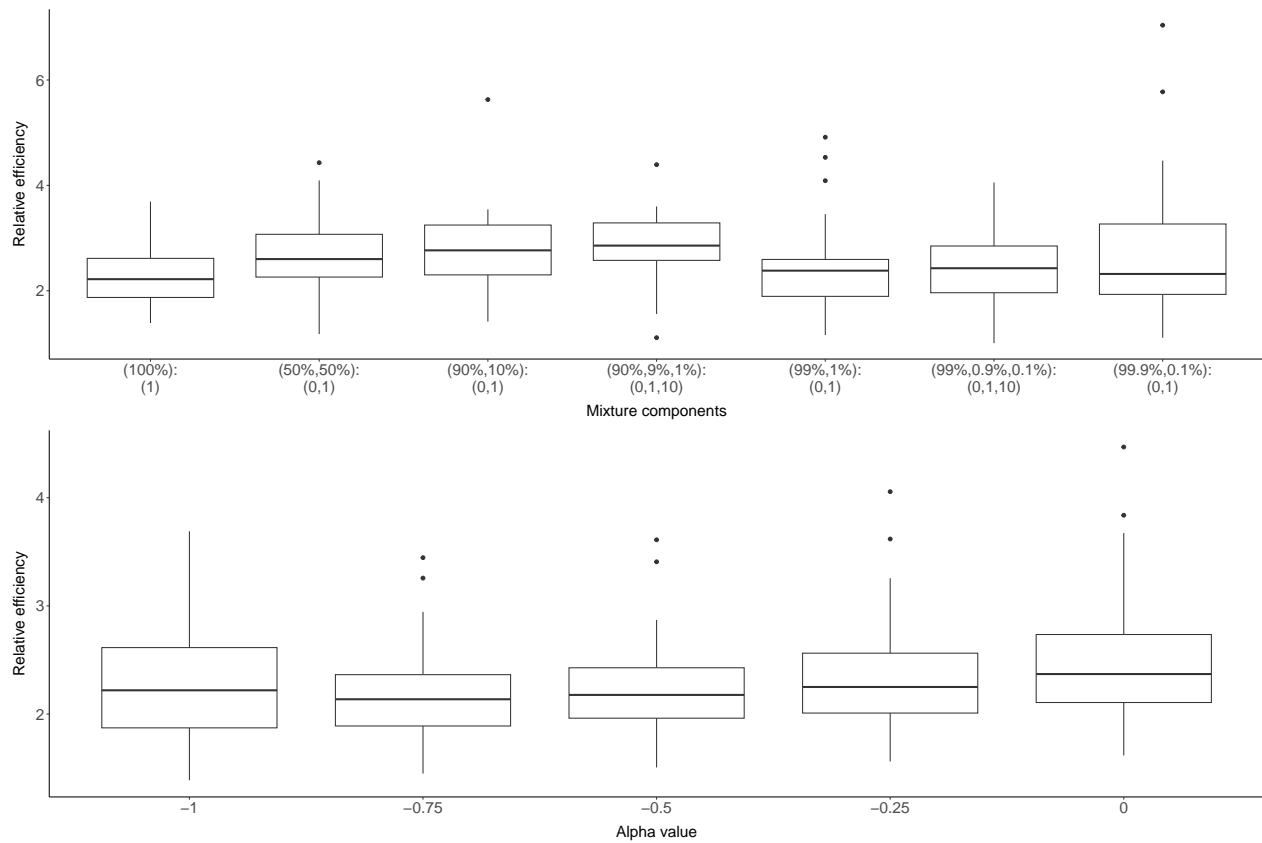
Supplementary Figure 7. Comparison of relative efficiency across different genetic architectures. The boxplots show the distributions of RE across parameters. The top panel corresponds to RE with varying mixture components; the bottom panel corresponds to RE with varying degrees of frequency-dependence. Numerical values of these results are provided in Supplementary Table 3 and 4 .
