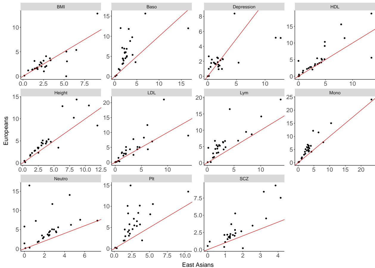
Supplementary Figure 23. Comparison of enrichment estimates between two ancestry groups. The difference to Supplementary Figure 19 is that plotted on the y-axis are the enrichment estimates based on GWAS summary statistics of European individuals (where UKB is not the major component of the sample). A summary of the summary statistics used in this comparison is provided in Supplementary Table 9-10 . The numerical values of the estimates are reported in Supplementary Table 12 .
