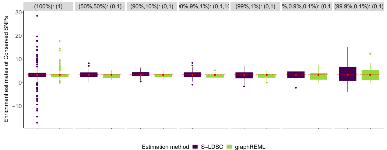
Supplementary Figure 4. Robustness of enrichment estimates under model mis-specifications: varying causal signal sparsity. Summary statistics are directly simulated based on the LDGM precision matrices on chromosome 1 from the Europeans in 1000 Genome ( p = 513,012, n = 100,000 ). The column panels represent different genetic architectures or mixture of causal effects, denoted as (component weights): (variance of the normal components). For example, (99%, 1%): (0,1) signifies that 99% of the SNPs are null and 1% of markers have their effect sizes drawn from N(0, 1) . The red dashed lines represent the true enrichment value.
