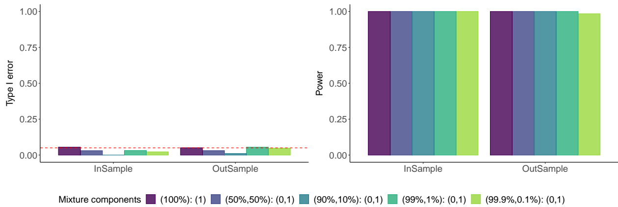
Supplementary Figure 20. The left panel is similar to Figure 1c in the main text; the right panel is similar to Supplementary Figure 17 . The difference is that the sandwich estimator of SE is used instead of the jackknife estimator ( Online Methods ).
