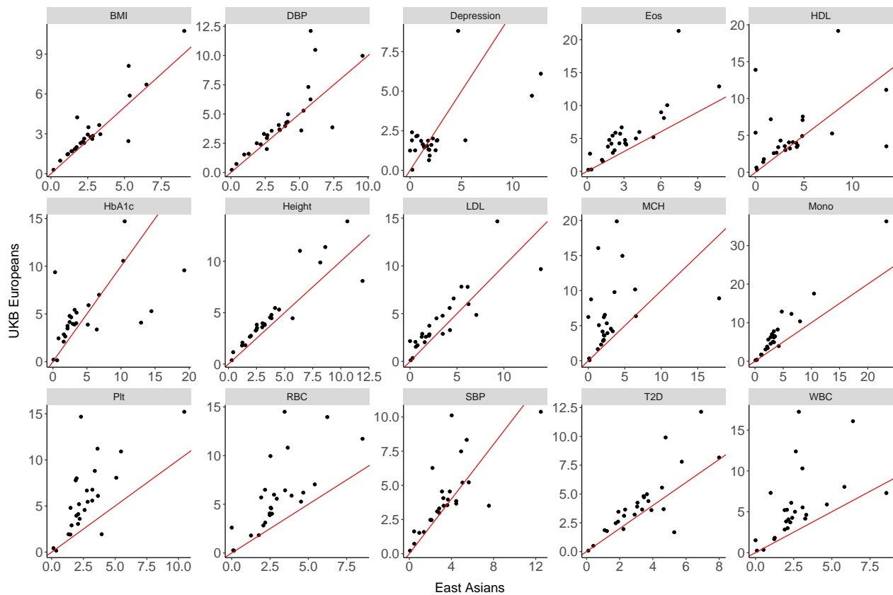
Supplementary Figure 22. Comparison of enrichment estimates between two ancestry groups. GWAS summary statistics and LDGM precision matrices inferred from matching ancestries are used to produce the enrichment estimates. LDGM precision matrices derived from the East Asian individuals in the 1000 Genome are used with the East Asian GWAS summary statistics. The red reference line is the 45 degree line. The numerical values of the estimates are reported in Supplementary Table 13 .
