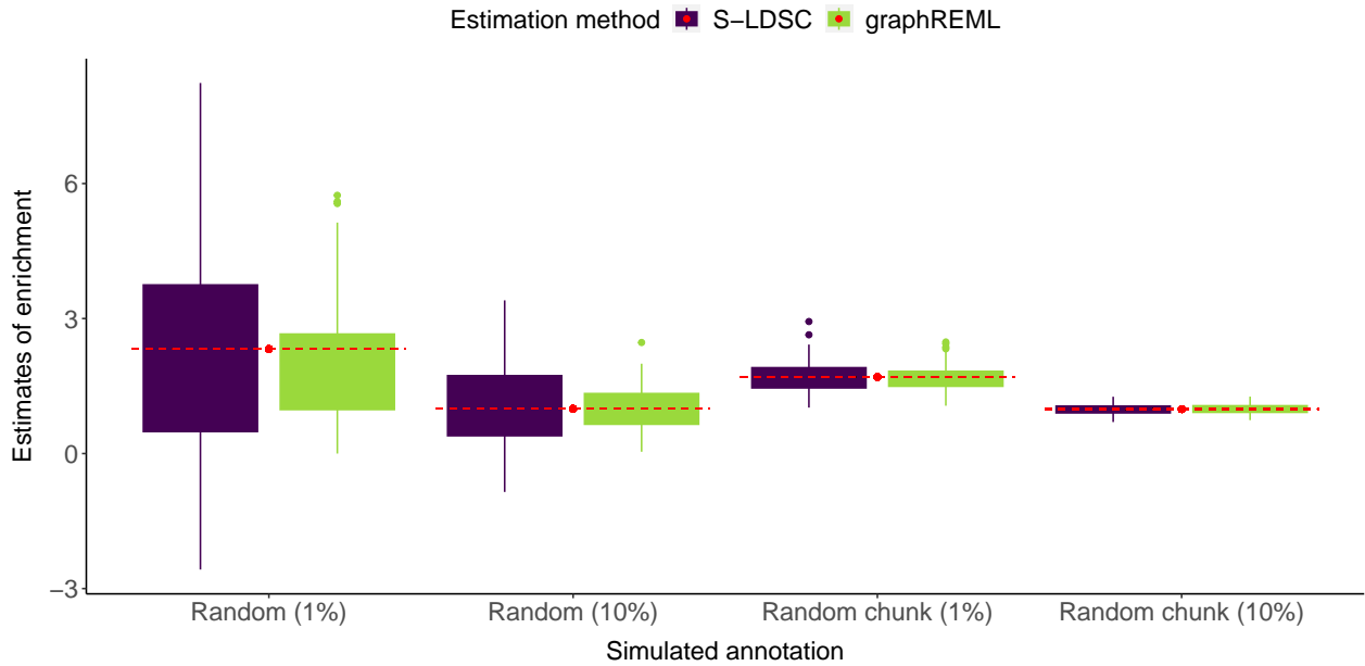
Supplementary Figure 3. Comparison of enrichment estimates for the random annotations. Summary statistics are directly simulated based on the LDGM precision matrices on chromosome 1 from the Europeans in 1000 Genome ( p = 513,012, n = 100,000 ). The boxplots show the empirical distributions of the enrichment estimates from S-LDSC or graphREML. "Random (1%)" corresponds to the annotation that randomly assigns 1 to 1% of the SNPs on the genome; "Random chunk (1%)" corresponds to an annotation where a random continuous region with the size of 1% of the genome is assigned 1. The red dashed lines represent the true values of heritability enrichment.
