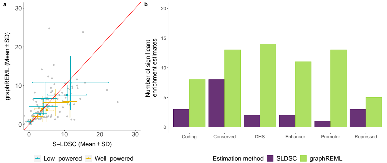
Supplementary Figure 16. Comparison of enrichment estimates from real trait analyses when both graphREML vs S-LDSC use out-of-sample LD. The association summary statistics are based on UK Biobank and the LDGMs are based on 1000 Genome.
