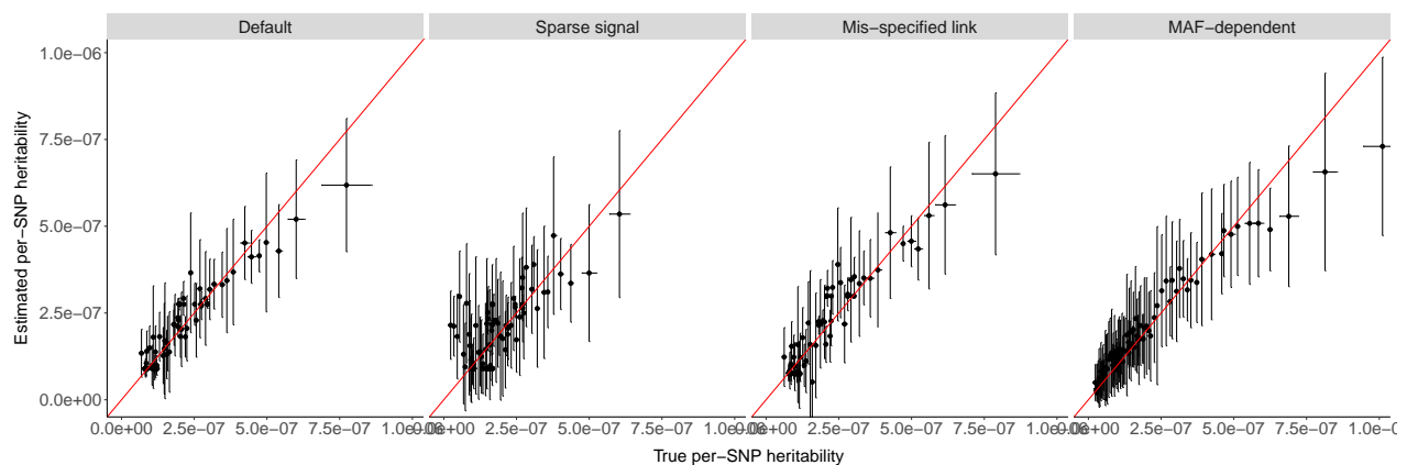
Supplementary Figure 9. Calibration of per-SNP heritability under different model mis-specifications. The points and the error bars on the x (y) axis correspond to the average and the SD of the true (estimated) per-SNP heritability. Colored in red is the 45 degree reference line. Alignment with the reference line indicates good calibration. The column panels represent different generative models or genetic architectures, same as those defined in Figure 1b of the main text.
