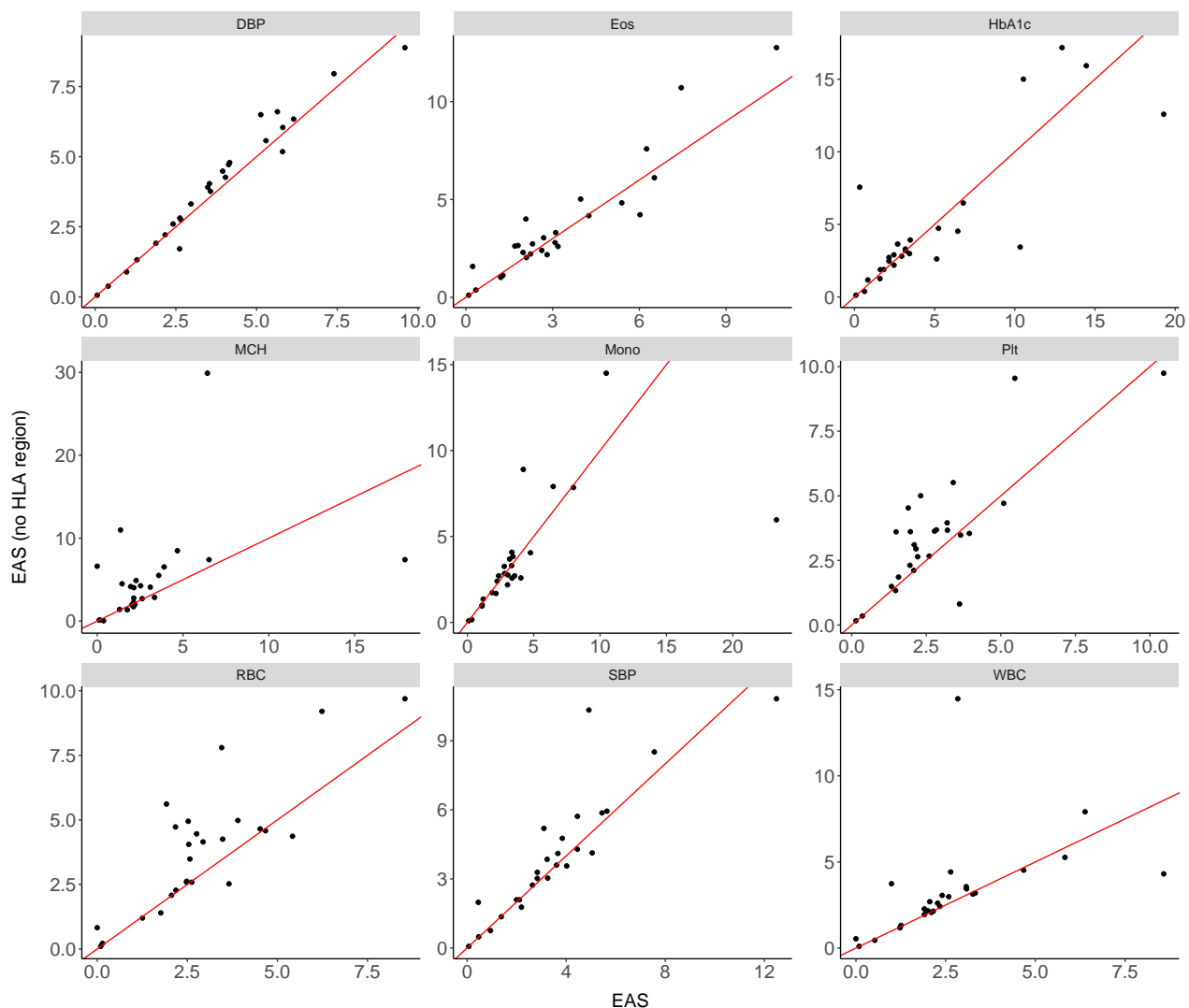
Supplementary Figure 24. Comparison of enrichment estimates with vs. without the variants in the HLA region included. The association statistics included in this analysis are blood or hematopoietic traits, for which we observed larger discrepancy in the enrichment estimates between Europeans and East Asians. LDGM precision matrices derived from the East Asian individuals in the 1000 Genome are used with the East Asian GWAS summary statistics. The red reference line is the 45 degree line.
