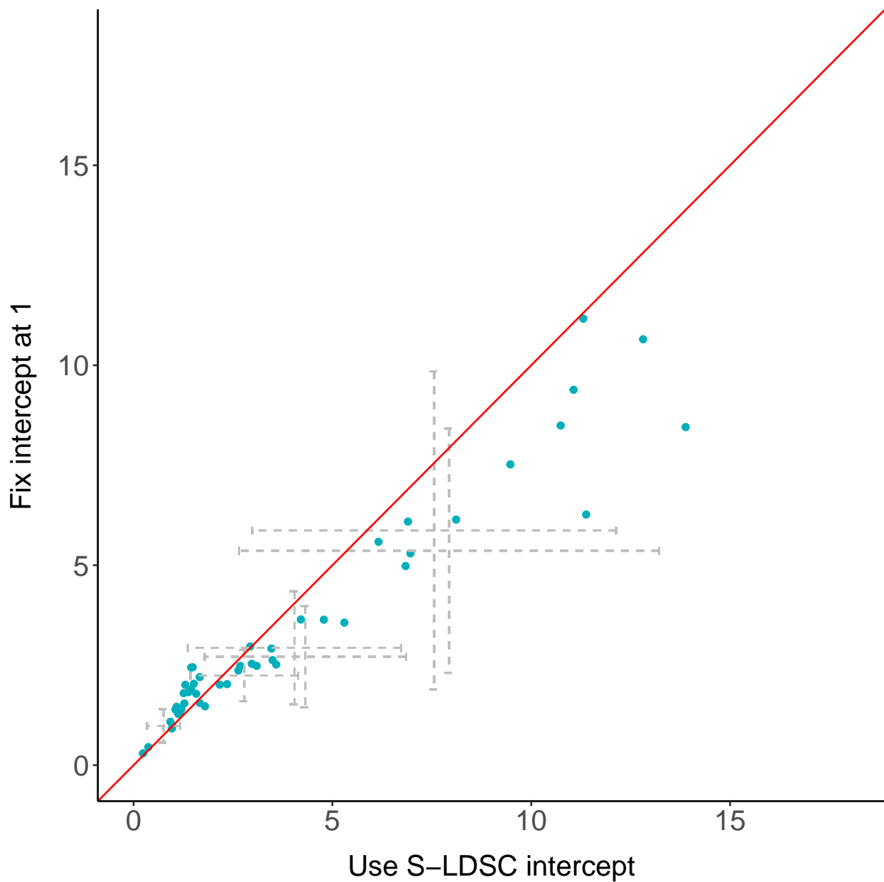
Supplementary Figure 26. Impact of controlling for population stratification through S-LDSC. Comparison of the graphREML results when we fix the intercept at 1 vs. at the S-LDSC estimated intercept. Blue dots are the enrichment estimates for the 18 validation traits (see descriptions of Figure 3 in the main analyses). Gray dotted lines are the meta-analyzed results for each annotation. Colored in red is the 45 degree reference line.
