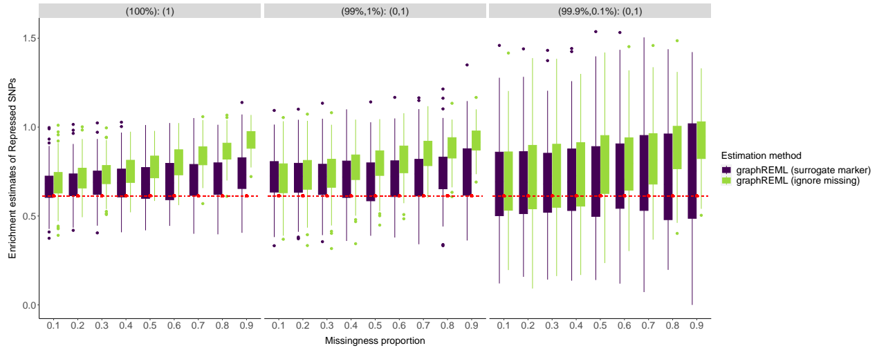
Supplementary Figure 12. Impact of missingness on enrichment (depletion) estimates. Summary statistics are directly simulated based on the LDGM precision matrices on chromosome 1 from the Europeans in 1000 Genome ( p = 513,012, n = 100,000 ). The x-axis represents the proportion of SNPs in the LDGM that are missing in the summary statistics. The column panels represent different genetic architectures or mixture of causal effects, denoted as (component weights): (variance of the normal components). For example, (99%, 1%): (0,1) signifies that 99% of the SNPs are null and 1% of markers have their effect sizes drawn from N(0, 1) . The red dashed line represents the true depletion value of the repressed SNPs in simulation.
