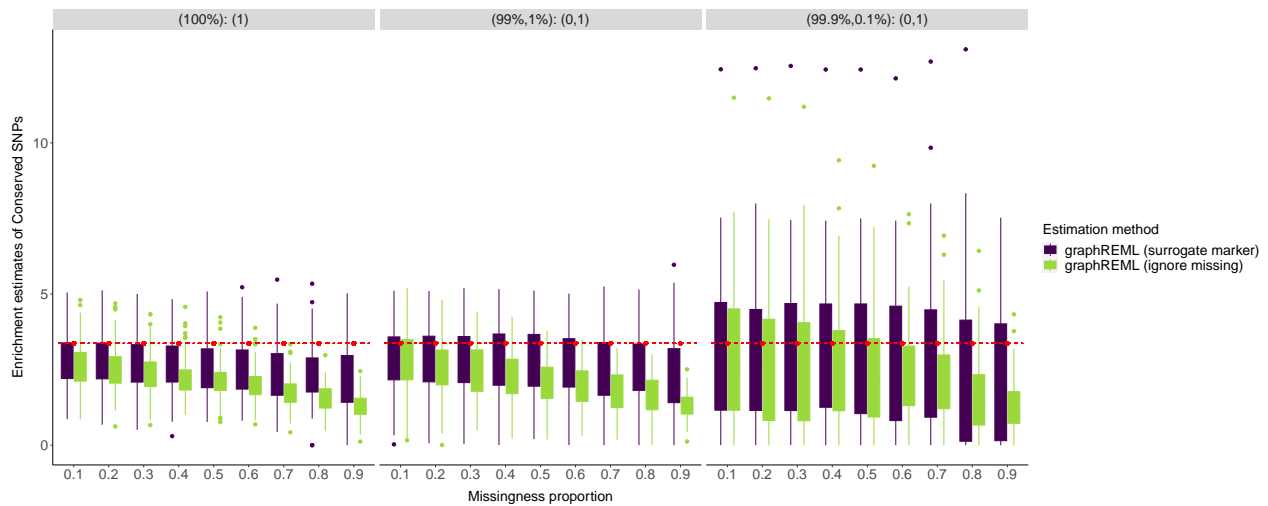
Supplementary Figure 13. Impact of missingness on enrichment (depletion) estimates. Summary statistics are directly simulated based on the LDGM precision matrices on chromosome 1 from the Europeans in 1000 Genome ( p = 513,012, n = 100,000 ). The x-axis represents the proportion of SNPs in the LDGM that are missing in the summary statistics. The column panels represent different genetic architectures or mixture of causal effects, denoted as (component weights): (variance of the normal components). For example, (99%, 1%): (0,1) signifies that 99% of the SNPs are null and 1% of markers have their effect sizes drawn from N(0, 1) . The red dashed line represents the true enrichment value of the conserved SNPs in simulation.
