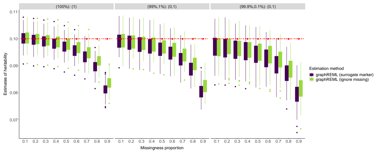
Supplementary Figure 14. Impact of missingness on heritability estimates. Summary statistics are directly simulated based on the LDGM precision matrices on chromosome 1 from the Europeans in 1000 Genome ( p = 513,012, n = 100,000 ). The x-axis represents the proportion of SNPs in the LDGM that are missing in the summary statistics. The column panels represent different genetic architectures or mixture of causal effects, denoted as (component weights): (variance of the normal components). For example, (99%, 1%): (0,1) signifies that 99% of the SNPs are null and 1% of markers have their effect sizes drawn from N(0, 1) . The red dashed line represents the true heritability in simulation.
