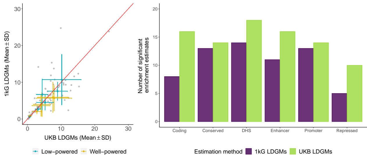
Supplementary Figure 17. Comparison of enrichment estimates from real trait analyses using in-sample (UKB) vs. out-of-sample (1kG) LDGMs. The set of phenotypes is the same as those used for method comparisons in Figure 3 of the main text. All estimates are based on graphREML.
