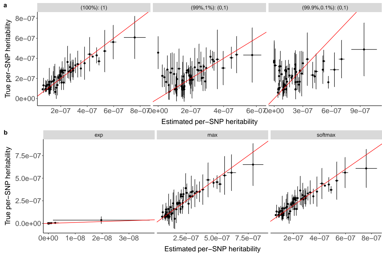
Supplementary Figure 11. Calibration of per-SNP heritability estimates from graphREML with different GWAS sample sizes. Summary statistics are directly simulated based on the LDGM precision matrices on chromosome 1 from the Europeans in 1000 Genome ( p = 513,012, n = 100,000 ). SNPs are first ordered by the true (estimated) per-SNP genetic variances and then assigned to 100 equal-sized bins, based on the percentile values in the top (bottom) row. Panel names represent the GWAS sample size. Each point represents the average true (or estimated) SNP-heritability on the X-axis (or Y-axis), respectively. The error bars correspond to the SD of the true or estimated SNP-heritability within the bin. The red reference is the 45 degree line, y = x .
