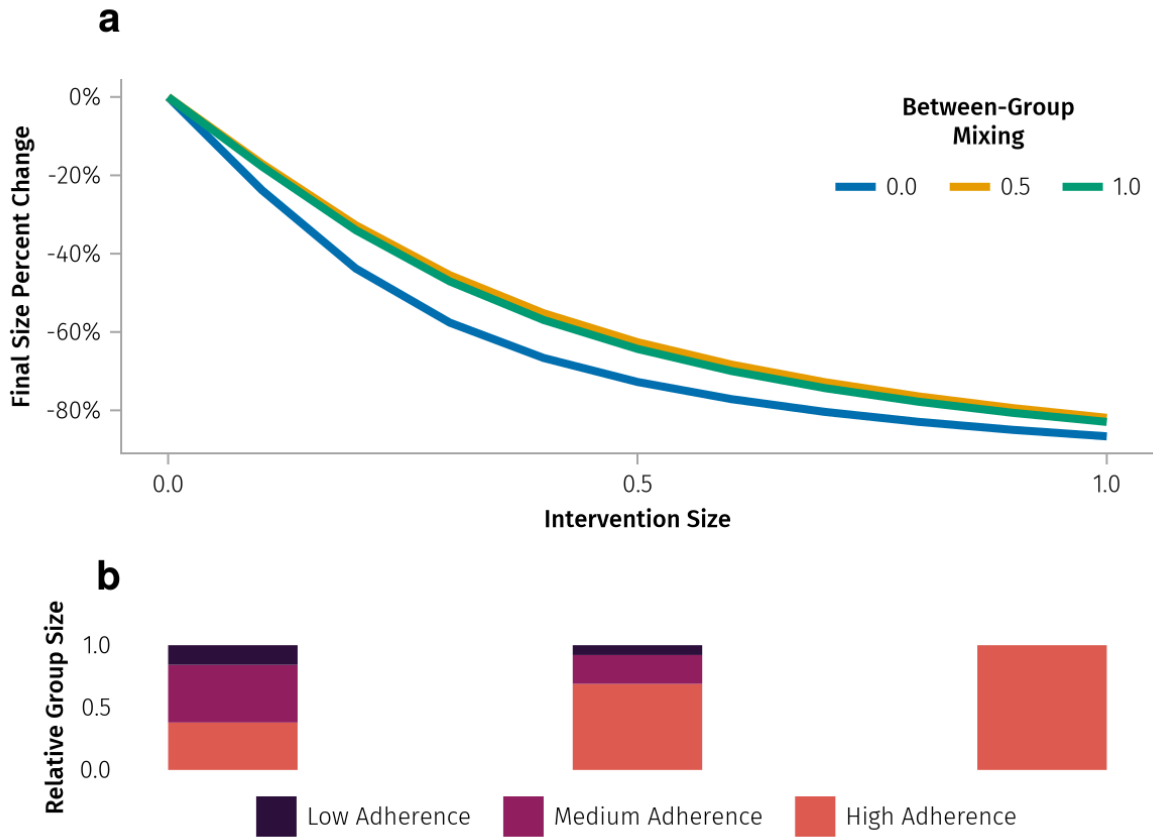
Figure 2: PHMs confer protection to the practitioner. A) The reduction in final infection size across a range of intervention effectiveness (1.0 is a fully effective intervention), accounting for a range of assortativity. Between-group mixing of 1.0 equates to between-group mixing as likely as within-group mixing; B) The relative distribution of group sizes at three levels of intervention effectiveness (0.0, 0.5, 1.0)
