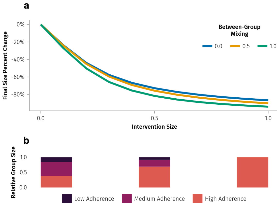
Figure 4: Identical off-diagonal values. A) The reduction in final infection size across a range of intervention effectiveness (1.0 is a fully effective intervention), accounting for a range of assortativity. Between-group mixing of 1.0 equates to between-group mixing as likely as within-group mixing; B) The relative distribution of group sizes at three levels of intervention effectiveness (0.0, 0.5, 1.0)
