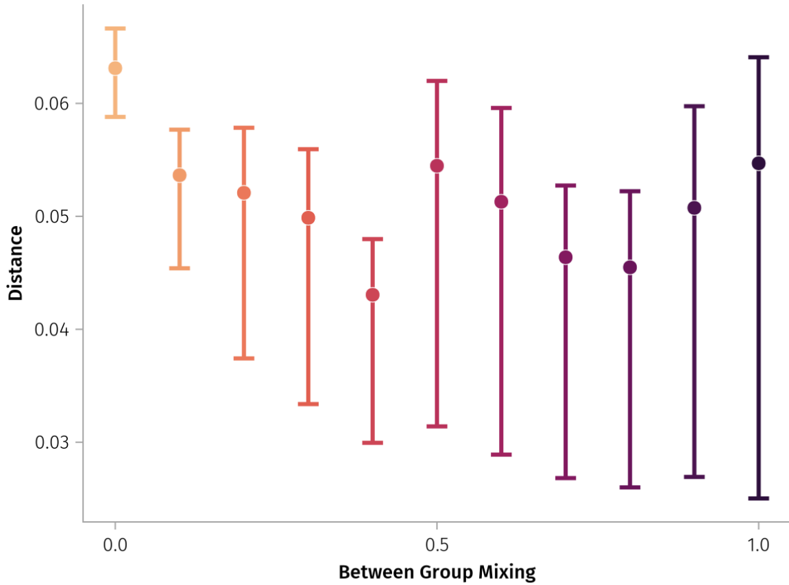
Figure 1: PHMs confer protection to the practitioner. Distribution of the distance from the ABC fits, with the minimum and maximum distances illustrated by the whiskers, and the median distance by the point. Between-group mixing of 1.0 equates to between-group mixing as likely as within-group mixing
