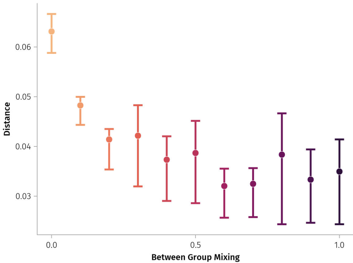
Figure 3: Identical off-diagonal values. Distribution of the distance from the ABC fits, with the minimum and maximum distances illustrated by the whiskers, and the median distance by the point. Between-group mixing of 1.0 equates to between-group mixing as likely as within-group mixing
