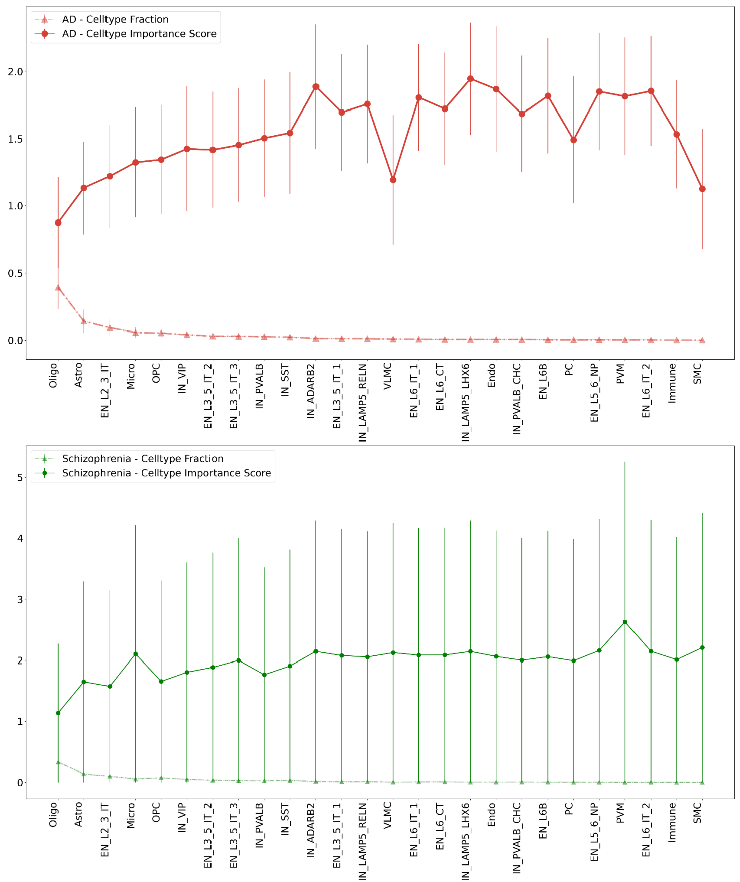
Supplementary Figure 8: Cell type importance scores for AD (top) and SCZ (bottom) samples. Circles indicate importance scores, and triangles represent cell fractions.
