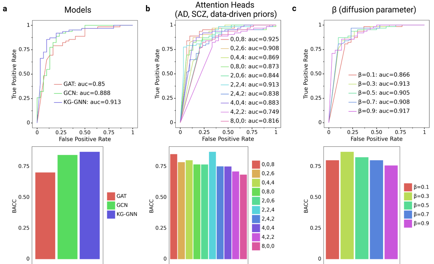
Supplementary Figure 4: Benchmarking KG-GNN model performance for AD vs. Control classification a , ROC curves and BACC comparing KG-GNN with state-of-art graph learning models: graph convolution networks (GCN), graph attention networks (GAT). b , ROC curves and BACC comparing different combinations of attention heads in the following order: AD, SCZ, Data-Driven. c , ROC curves and BACC comparing values for diffusion parameter \beta . (see Supplementary Note 4 )
