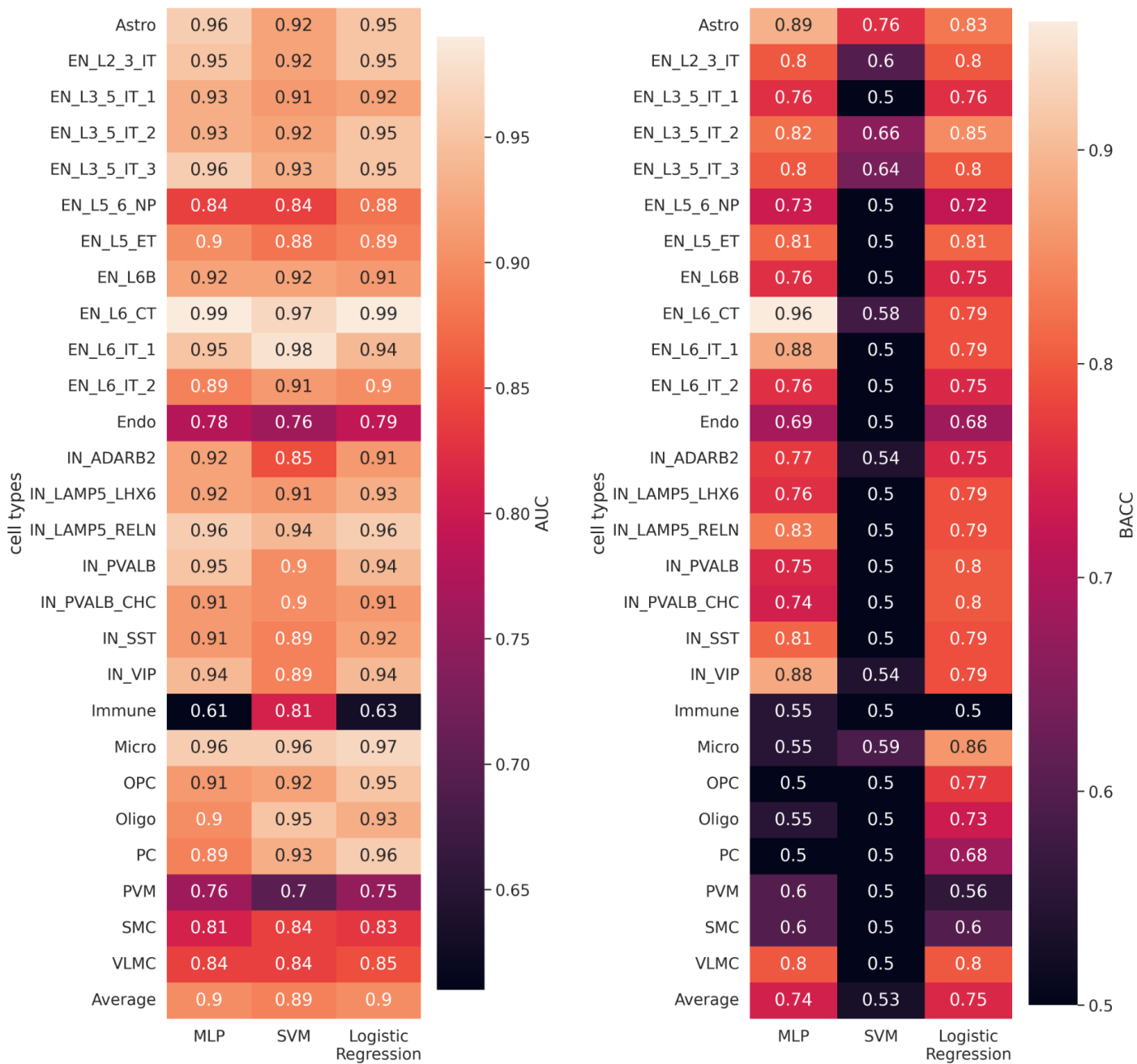
Supplementary Figure 5: Benchmarking classification performance of donors with AD vs. Controls for three machine learning models: Multi-linear Perceptron (MLP), Support Vector Machines (SVM), and Logistic Regression (LR). Here we classify each donor's average cell type gene expression into AD or Control groups using the three models across all cell types reporting metrics area-under-the-curve (AUC) and balanced accuracy (BACC) (see Supplementary Note 5 ).
