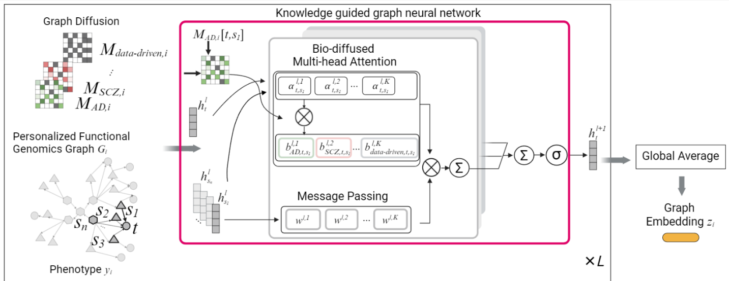
Supplementary Figure 2: Architecture of knowledge-guided graph neural network (KG-GNN) Given a PFG G_i , the inputs to the KG-GNN model include its bio-diffused PFG ( M_{AD,i} , M_{SCZ,i} , ..., M_{data-driven,i} ) and node features h . The KG-GNN uses a self-attention mechanism to calculate attention scores between a node t and its neighbors s_j and incorporates prior biological knowledge through edges using our bio-diffused PFGs M_{AD,i} , M_{SCZ,i} to get bio-diffused attention scores or priors b_{AD,t,s_j} , b_{SCZ,t,s_j} , ..., b_{data-driven,t,s_j} . These are normalized across node t 's neighborhood and are used to compute a linear combination of the node features corresponding to them using a softmax function to further update the t 's node features. (see Supplementary Note 2 )
