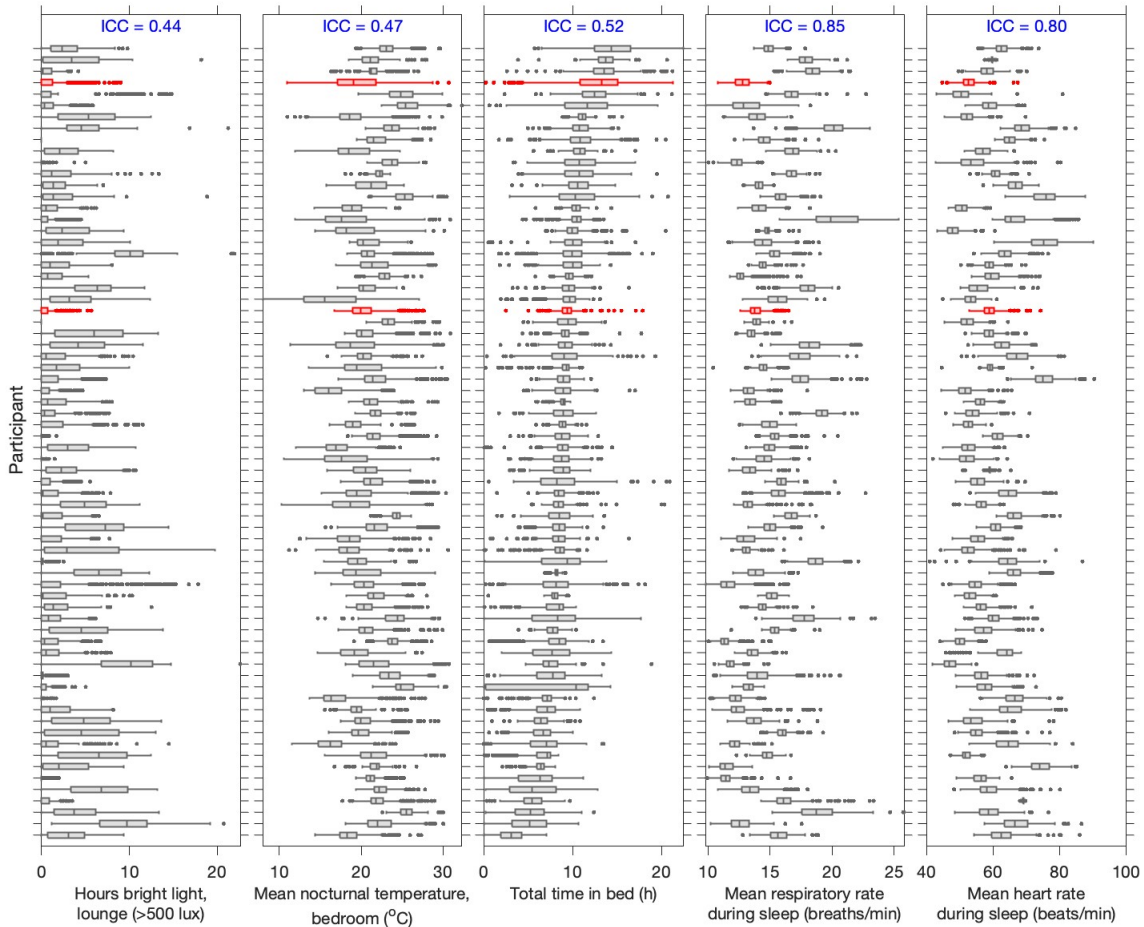
Figure S2: Between and within participant variation in indoor light and temperature environment, bed occupancy, respiratory rate and heart rate. Box plots for each participant showing the between and within participant variation in a few example metrics that quantify aspects of the indoor daytime light environment, the nighttime temperature environment, time in bed, respiratory rate and heart rate.
