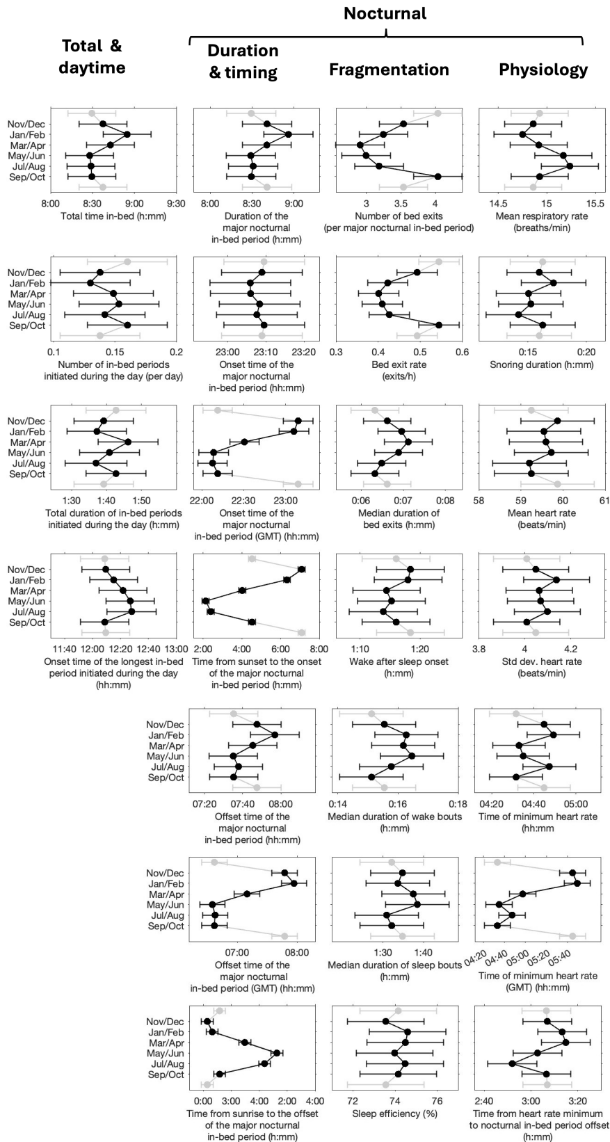
Figure S3: Seasonal variation of in-bed duration, timing and fragmentation, physiology. The data shown are the Least Squares (LS) means from a linear mixed effect model which considers the seasonal variation for each measure controlling for gender, age and diagnosis with participant as a random effect (see Supplementary Table S5). Eight of the 25 measures are also shown in the Fig. 3 of the main text. All measures are included here for ease of visual comparison.
