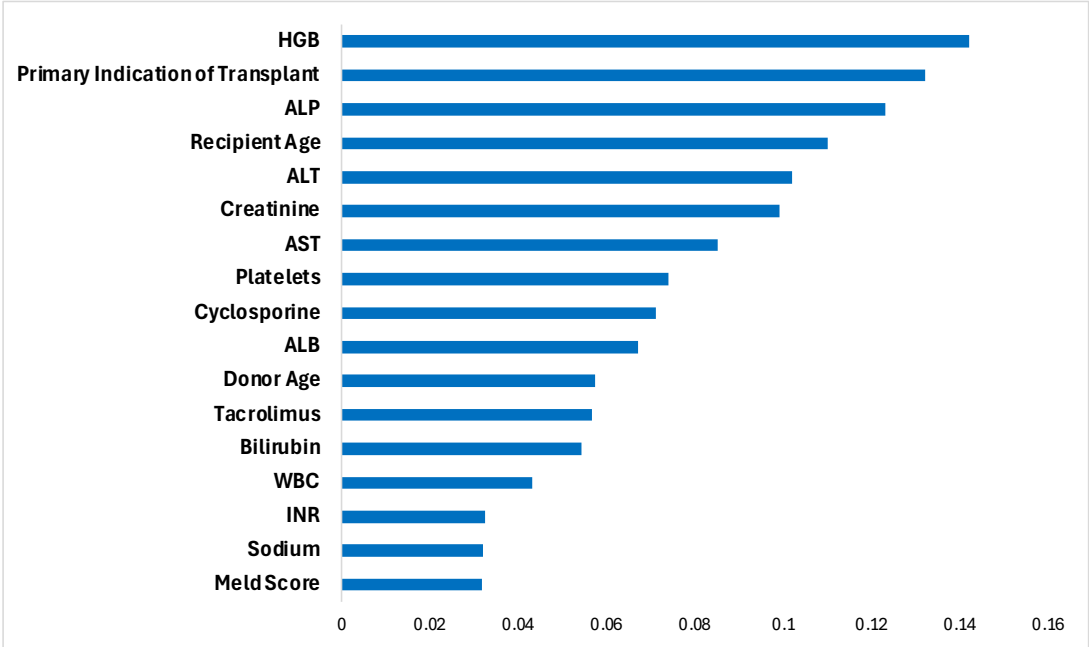
Gradient obtained using Neural Network
