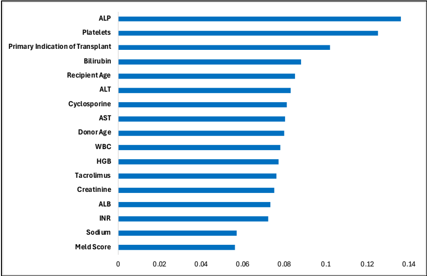
Gradient obtained using Neural Network
