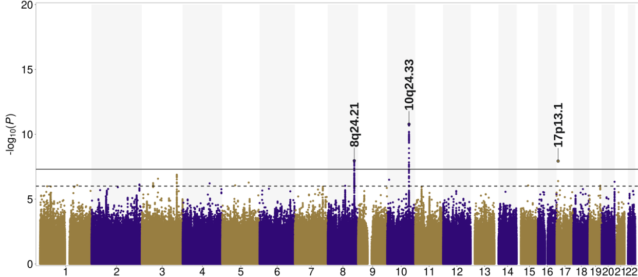
Supplementary Figure 2: Manhattan plot highlighting the lead chromosomal regions ( P < 5 \times 10^{-8} ) from the genome-wide association study of multiple invasive cancers ( n = 8,673 ) versus cancer-free controls ( n = 420,944 ). The solid black line signifies the genome-wide significance threshold ( P < 5 \times 10^{-8} ), whereas the dashed black line represents a suggestive significance threshold of P < 1 \times 10^{-6} .
