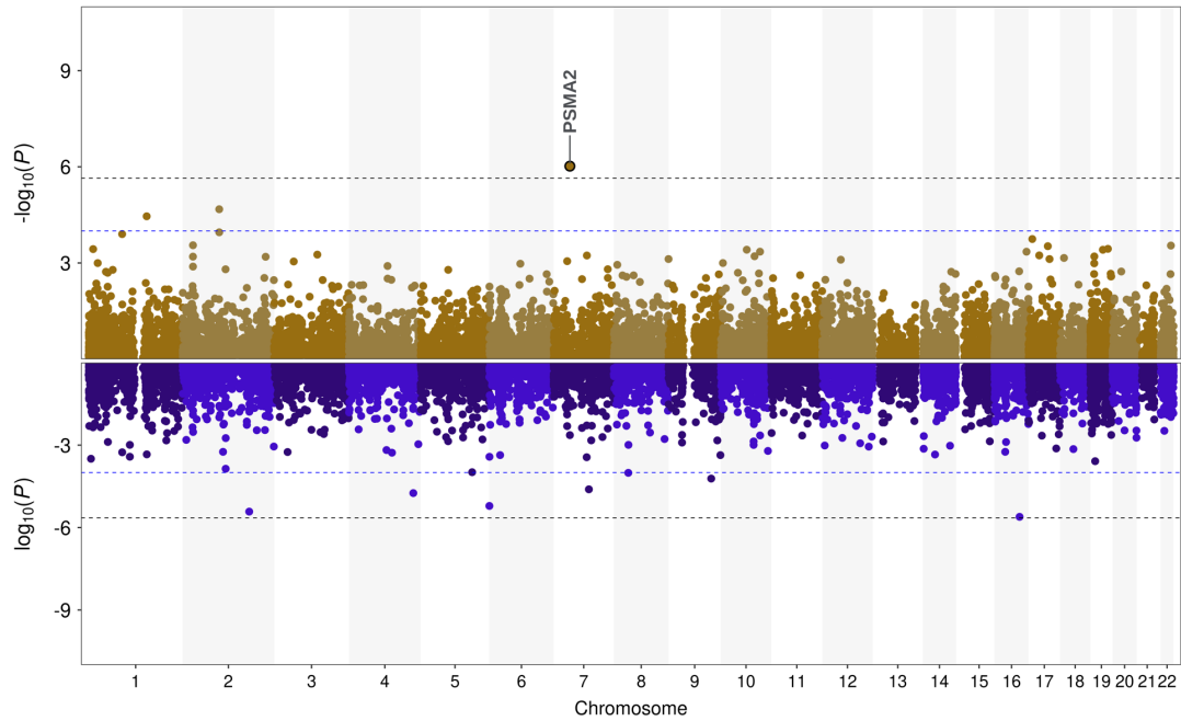
(B) TWAS of multiple invasive cancers (8,673 cases and 72,686 single invasive cancer cases as controls)
