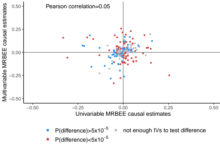
Fig. 13 These results display the bivariate association between univariable MR and multivariable MR causal estimates and indications of the significance in testing H_0 : I_3 = 0 from the text above. Red and blue points respectively represent genes for which this null hypothesis was rejected and not rejected at P < 5 \times 10^{-5} . Grey points correspond to genes for which the test could not be reliably performed because of imprecise variance estimation in \hat{I}_3 . For these genes, we could not estimate a positive \hat{\sigma}_\Theta^2 (see Equation 21) because of very small valid IV counts in univariable MR. ‘Pearson correlation’ corresponds to the linear correlation between univariable and multivariable MR causal estimates. This value will be 1 if there is no omitted variable (OV) bias (due either to CHP or mediation effects) and will approach 0 as OV bias becomes stronger.
