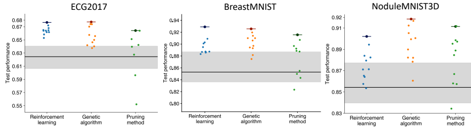
Fig. 4: Performance of ensemble prediction (larger dot with a dash) and optimized architectures (dot) compared with benchmark results (gray area). The horizontal line is the median, and the gray area is the upper to lower quartile region, for the performance of 150 benchmark architectures, respectively.
