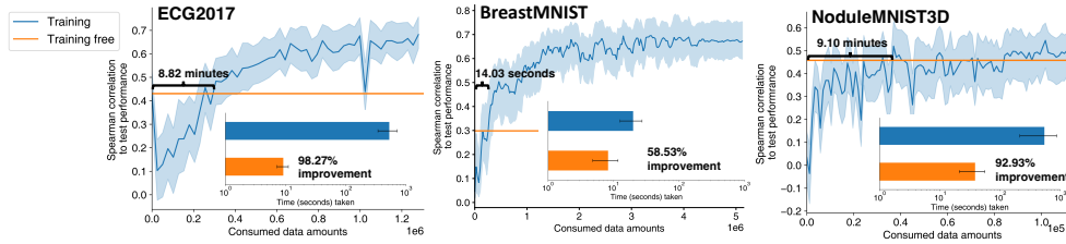
Fig. 3: Comparison of computation time costs between partial training and the TEACUP metric when they achieve equal Spearman correlations with the final trained DNN performance. For “Training”, the Spearman correlation across the 150 benchmark architectures (y-axis) is calculated between the testing and the validation accuracy after trained for a certain amount of data (x-axis). Orange horizontal lines correspond to values of \rho in the left column of Fig. 2.
