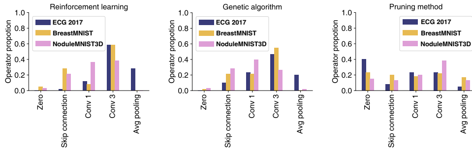
Fig. 5: Distributions of optimized architectures by reinforcement-learning, genetic-algorithm, and pruning-method on three datasets.
