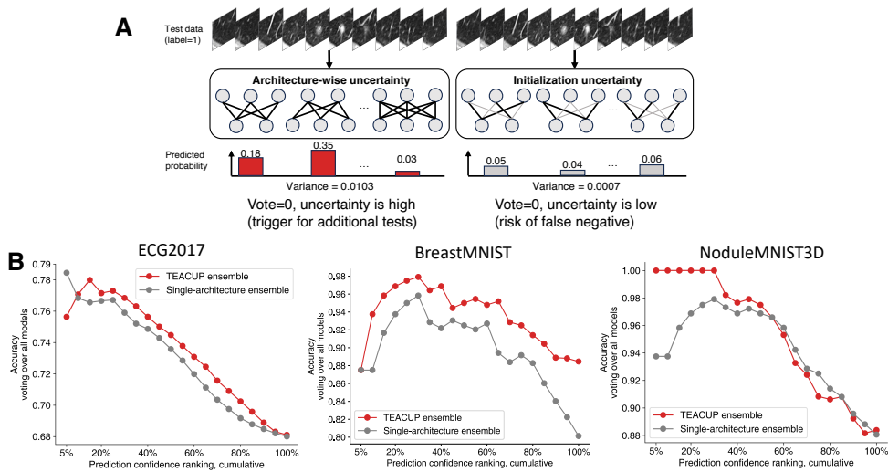
Fig. 6: (A) Comparison of a false negative test case over two uncertainty quantification methods: different architectures vs. single architecture trained from different weight initialization. Despite both methods yielding incorrect predictions, the larger architecture-wise uncertainty suggests the need for additional tests. (B) Across testing samples of different confidence, the ensemble of TEACUP-optimized models (search method: RL for ECG2017, pruning for BreastMNIST, Genetic for NoduleMNIST3D) outperforms the ensemble of a single architecture trained from random initialization.
