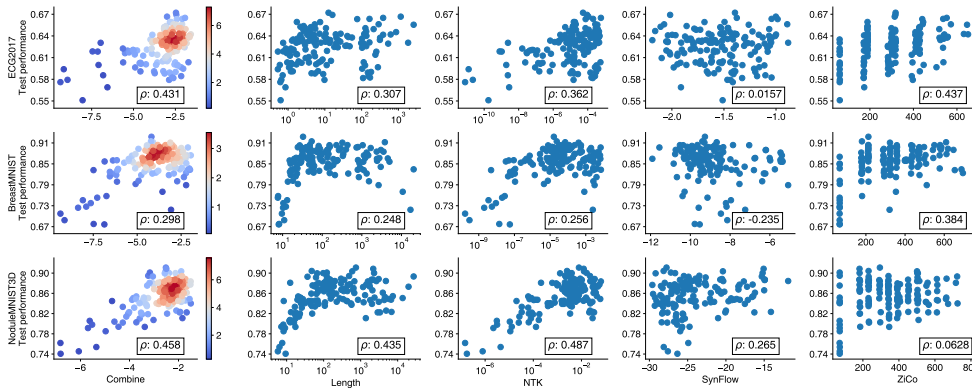
Fig. 2: Spearman correlation between the test reward and training-free metrics. A composite TEACUP metric (left) is derived by combining all four metrics: Length, NTK, SynFlow, ZiCo.
