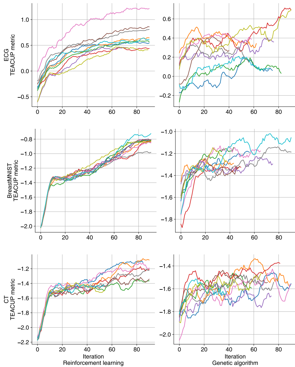
Supplementary Figure 3: Change of TEACUP metrics as iteration increases in reinforcement learning and genetic algorithm. Different colors represent different, independent search runs.
