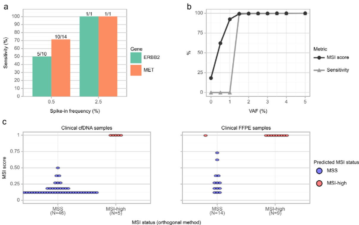
Fig. 2: Analytical performance for CNV detection and MSI status determination. a. Analytical sensitivity for the detection of MET and ERBB2 CNVs in reference standards at 0.5% and 2.5% spike-in frequency. b. MSI score reported by Hedera Prime and MSI status determination sensitivity on in-silico dilutions of reference standards. c. Estimated MSI score and predicted MSI status by HP2 versus predicted MSI status by orthogonal assays on clinical cfDNA samples and clinical FFPE samples.
