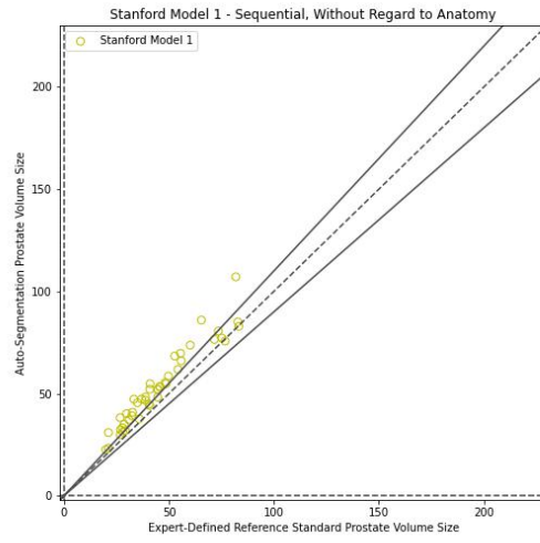
Stanford Model 1
