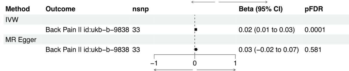
Fig. 4. A) Exposures potentially causal for LSS, and B) outcomes that LSS was potentially found to be causal for. The analysis was performed using the TwoSampleMR R library and data from the present study and MRC-IEU database. The inverse variance weighted (IVW) model was our primary analysis, for which statistical significance was considered at false discovery rate corrected p-value (pFDR < 0.05). We also performed a sensitivity analysis using MR Egger. nsnp, number of SNPs; OR (95% CI), odds ratio and its 95% confidence interval; Beta (95% CI), beta estimate and its 95% confidence interval; pFDR, false discovery rate-corrected p-value.
