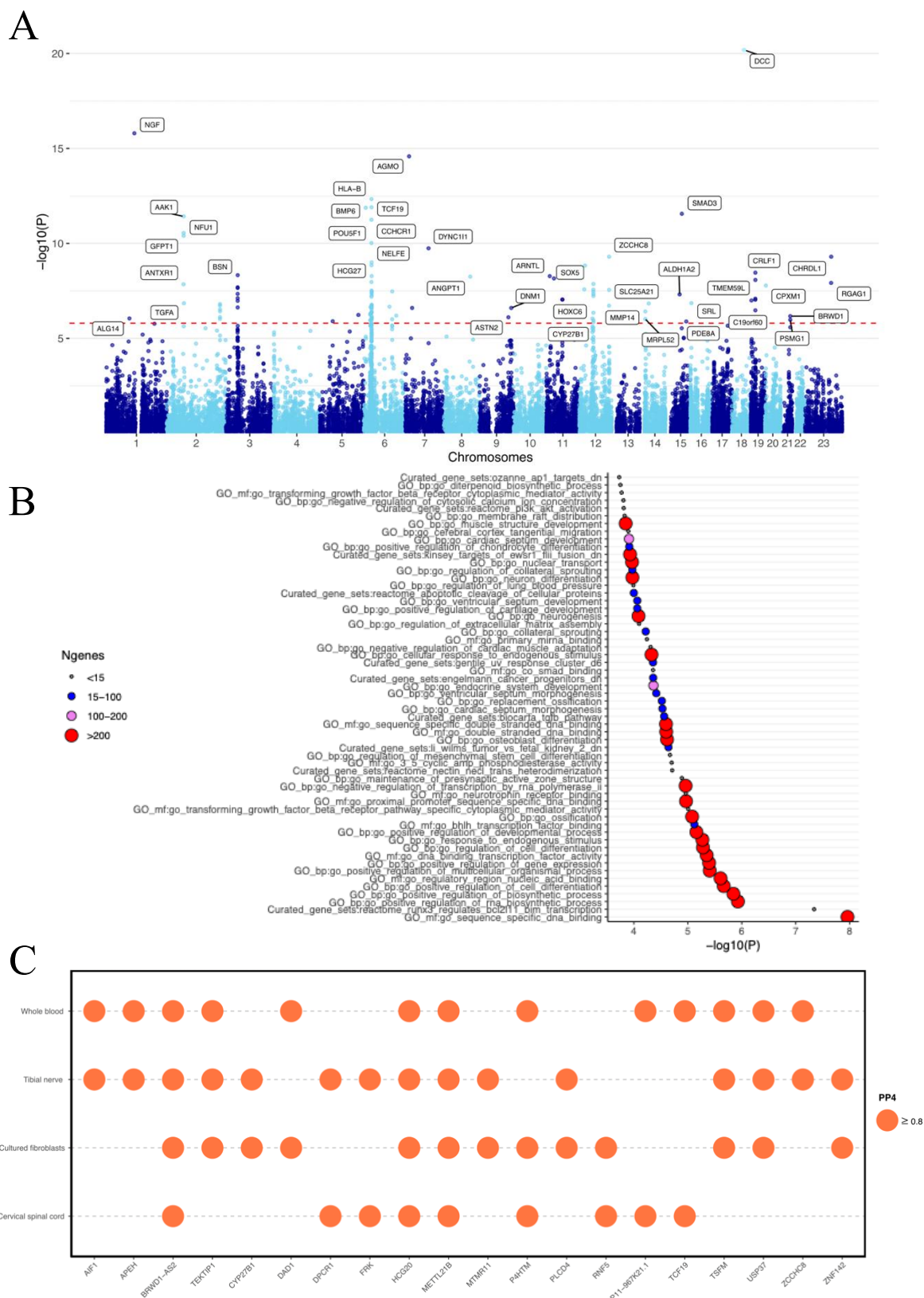
Fig. 2. A) Results of the MAGMA 26 gene-based test in a Manhattan plot. X-axis chromosomes, y-axis -\log_{10}(p\text{-value}) . B) MAGMA gene-set enrichment analysis. The plot shows significantly enriched pathways ( p\text{FDR} < 0.05 ), curated gene sets, and GO-annotations ranked by significance ( -\log_{10}(P\text{-value}) ). The circle size refers to the size of the gene set. Small gray <15 , blue 15\text{--}100 , violet 100\text{--}200 , and red >200 genes. The analysis was done using FUMA 27 , and the gene sets and GO annotations included in the analysis are from MSigDB 28 . C) Colocalizations between LSS GWAS and eQTL signals were estimated with approximate Bayesian factor analyses, implemented with the ‘coloc.abf’ function available in the ‘coloc’ R-library (Table S7). The ‘biomaRt’ R-library was used to extract genes from Ensembl archives 29 within a 1 MB ( \pm 500000 bases) window surrounding each lead variant. Colocalizations were investigated for 754 genes that were available in GTEx. Variant-gene expression associations for selected tissues (whole blood, cultured fibroblasts, tibial nerve, and cervical spinal cord) were downloaded from GTEx v8. Colocalizations with posterior probabilities \geq 0.8 for the variant were considered significant 30 . Only genes with at least two significant colocalizations are shown in the plot; all significant colocalizations are listed in Table S7.
