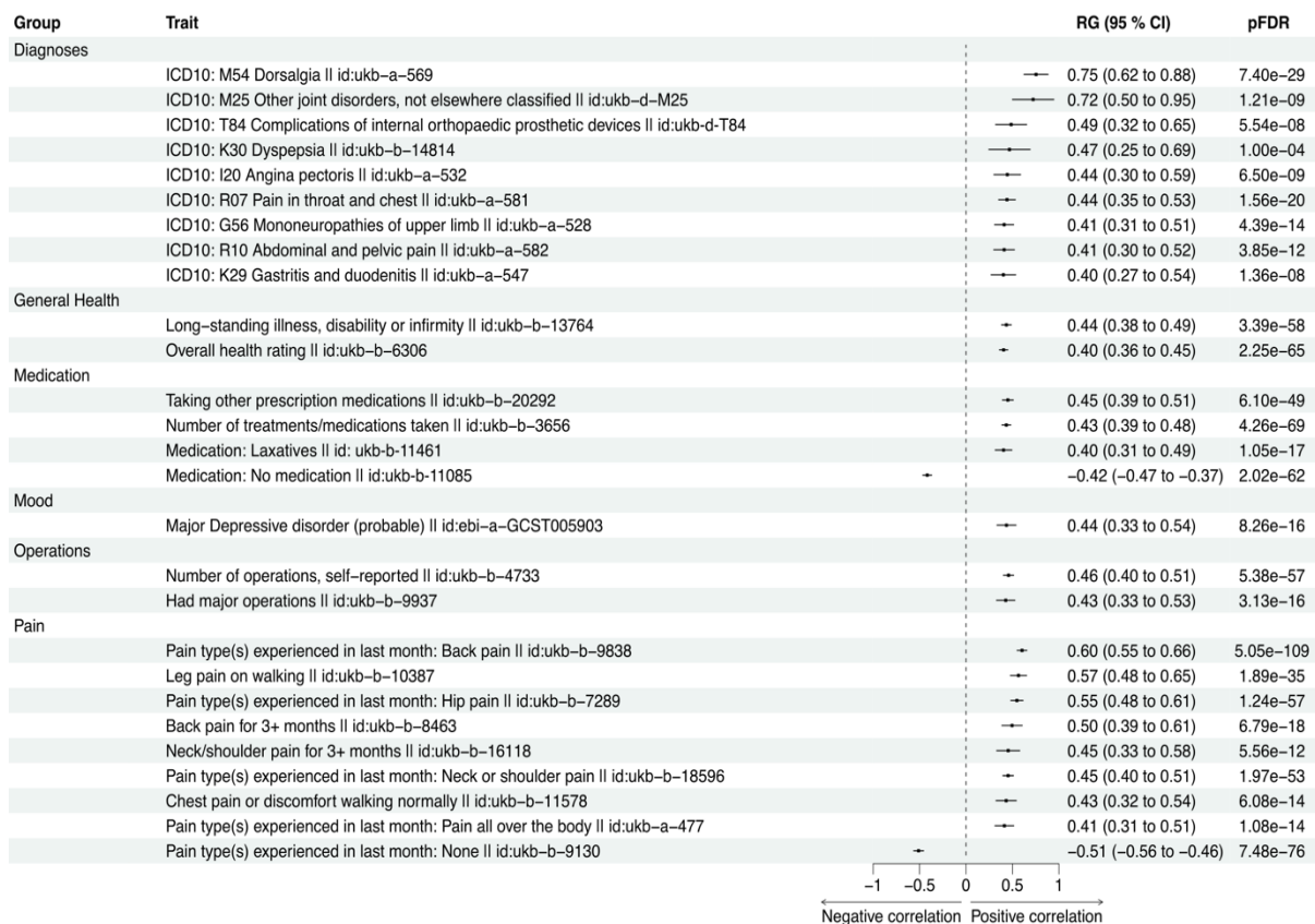
Fig. 3. Genetic correlations were calculated using LDSC-software 8,31 . All traits were extracted from the GWAS database provided by the MRC Integrative Epidemiology Unit (IEU). Only the strongest observed ( rg < -0.4 & rg > 0.4 ) correlations with a significant false discovery corrected p-value ( p_{FDR} < 0.05 ) are shown in the figure. RG, genetic correlation coefficient value; pFDR, false discovery rate-corrected p-value. Genetic correlations for all 517 phenotypes can be seen in Table S9.
