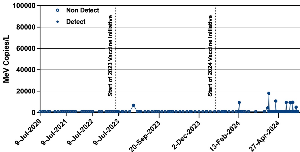
Figure 1: Genome copies of MeV per litre of wastewater sample from July 2020 to May 31, 2024. The open circles indicate non detects and closed circles indicate detects. The dashed lines indicate the approximate start of increased vaccination efforts by Ottawa Public Health in 2023 and in 2024.
