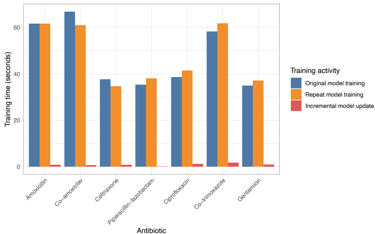
Figure S14. Model training, retraining and model updating times. All times are from training using a single Apple M3 Max core. Original and repeat training include hyperparameter optimisation, incremental updates are based on previously obtained hyperparameters from initial training.
