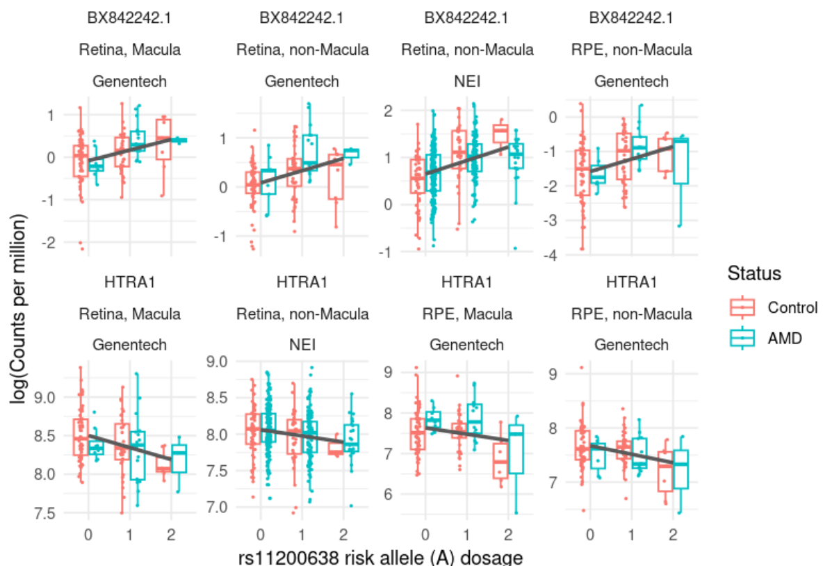
Fig. 4: Increased RPD genetic risk is associated with increased expression of BX842242.1 retinal RNA, and decreased expression of HTRA1 . Only significant eQTL results are displayed. BX842242.1 : long
