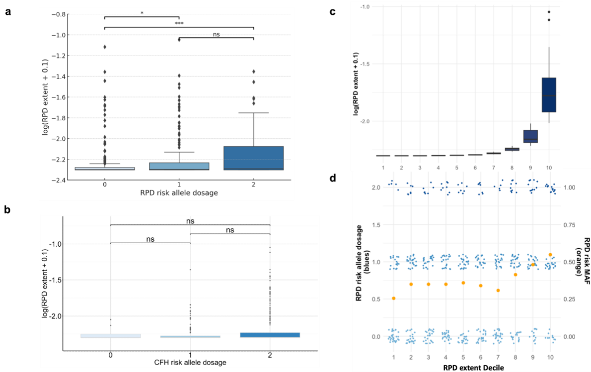
Fig. 3. Reticular pseudodrusen (RPD) extent is significantly associated with heightened RPD genetic risk. a Box plot showing the RPD extent in N=526 individuals relative to the RPD-risk lead SNP (rs11200638) dosage (x-axis) and b Box plot showing RPD extent in N=526 individuals relative to the CFH top risk SNP (rs10922109) based on Fritsche et al (7) dosage (x-axis) while adjusting for age and sex as covariates. The y-axis represents the log-transformed RPD extent based on a percentage of the entire scan with RPD (the mean RPD extent of the left and right eyes were used) adding a constant of 0.1 to avoid log (0) of N=181 individuals who showed a mean extent RPD value of zero. A linear regression test was conducted to examine the differences in the RPD extent across the genotype groups controlling for age and sex. We performed pairwise Wilcoxon tests with Bonferroni correction to directly compare the p-values among groups. Significant differences between groups are indicated by asterisks (p > 0.05: 'ns', p < 0.05: '*', p < 0.01: '**', p < 0.001: '***'); c RPD extent as defined in panel a (y-axis), binned into deciles (x-axis) for analysis of RPD risk. d RPD risk allele frequency (left y-axis) relative to RPD extent deciles (x-axis); In d, blue points represent individual study participants' genetic risk, colored by risk allele dosage. Orange points represent risk allele frequency per decile (right y-axis). The plot illustrates how the RPD-risk lead SNP genotypes vary across different levels of RPD extent, providing insights into the genetic association between RPD risk and the severity of RPD.
