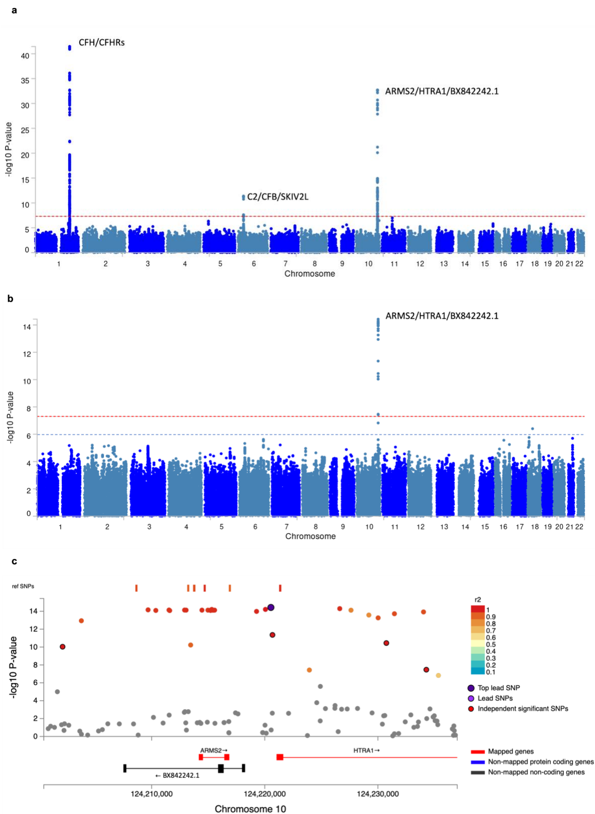
Fig. 2: Results of Genome-wide association studies (GWAS). a Manhattan plot of overall AMD-GWAS meta-analysis showing -\log_{10}(P\text{-value}) values across the genome comparing AMD+ (RPD+/-) participants (N= 3,959) vs. AMD- controls (N= 1,946). The red horizontal line represents the genome-wide significance level ( P\text{-value} = 5 \times 10^{-8} ). Nearby genes to the two main associated loci with AMD risk on chromosomes 1, 6 and 10 are labelled; b Manhattan plot of the meta-analysis of AMD+/RPD+
