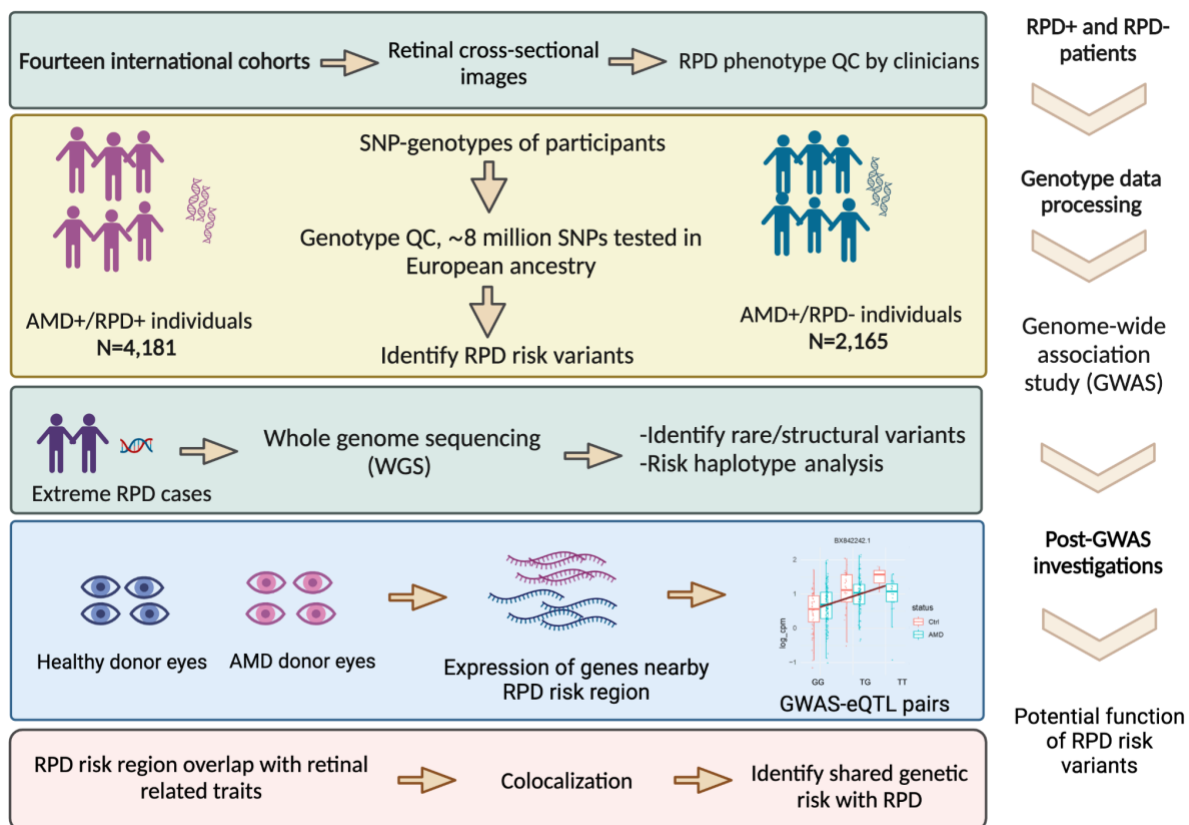
Fig. 1: Overall study design in multiple stepwise strategies from cohort collection, GWAS to subsequent post-GWAS analyses.
