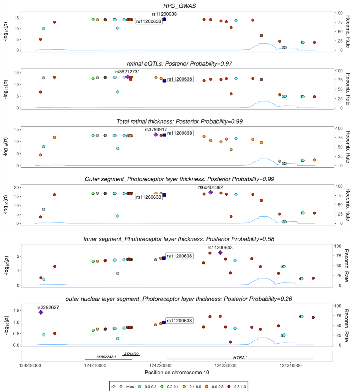
Fig. 5. Genome-wide multi-trait colocalization analysis of RPD and candidate traits that show ARMS2/HTRA1 locus as a significant risk-associated region. Stacked association plots of traits with > 95% shared variants with RPD. Colocalization analysis with Coloc implicates the RPD risk lead variant rs11200638 as being the shared causal variant between RPD risk and eQTLs, photoreceptor cell outer segment (OS) thickness and total retinal thickness. In contrast, the thickness of photoreceptor cell layers including the inner segment (IS) and photoreceptor cell outer nuclear layer (ONL) did not show a high overlap with the RPD risk region. Each plot includes a recombination rate track (blue line) and a linkage disequilibrium (LD) color scale indicating the r^2 values of SNPs in relation to RPD-risk lead SNP (rs11200638). The x-axis represents the position on chromosome 10, and the y-axis represents the -\log_{10}(P\text{-value}) of association. The blue bars on the x-axis label the genes. IncRNA BX842242.1 was added manually. The purple diamond represents the most significant SNP in the region for each trait and the dark blue square represents the RPD-risk lead SNP (rs11200638) in each trait.
