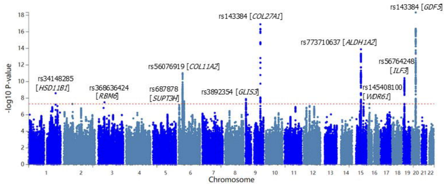
Primary GWAS
