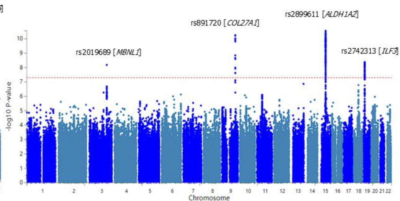
Male-specific GWAS
