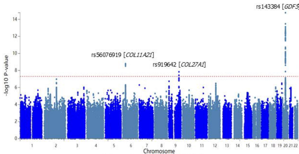
Female-specific GWAS
