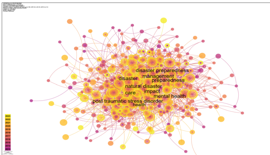
Fig 6. Map of keywords
