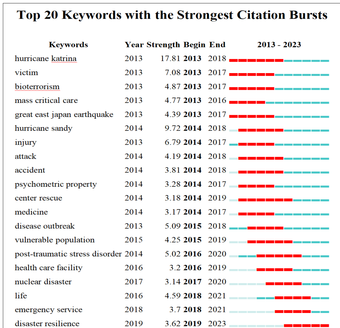
Fig 9. Top 20 keywords with the strongest citation bursts
