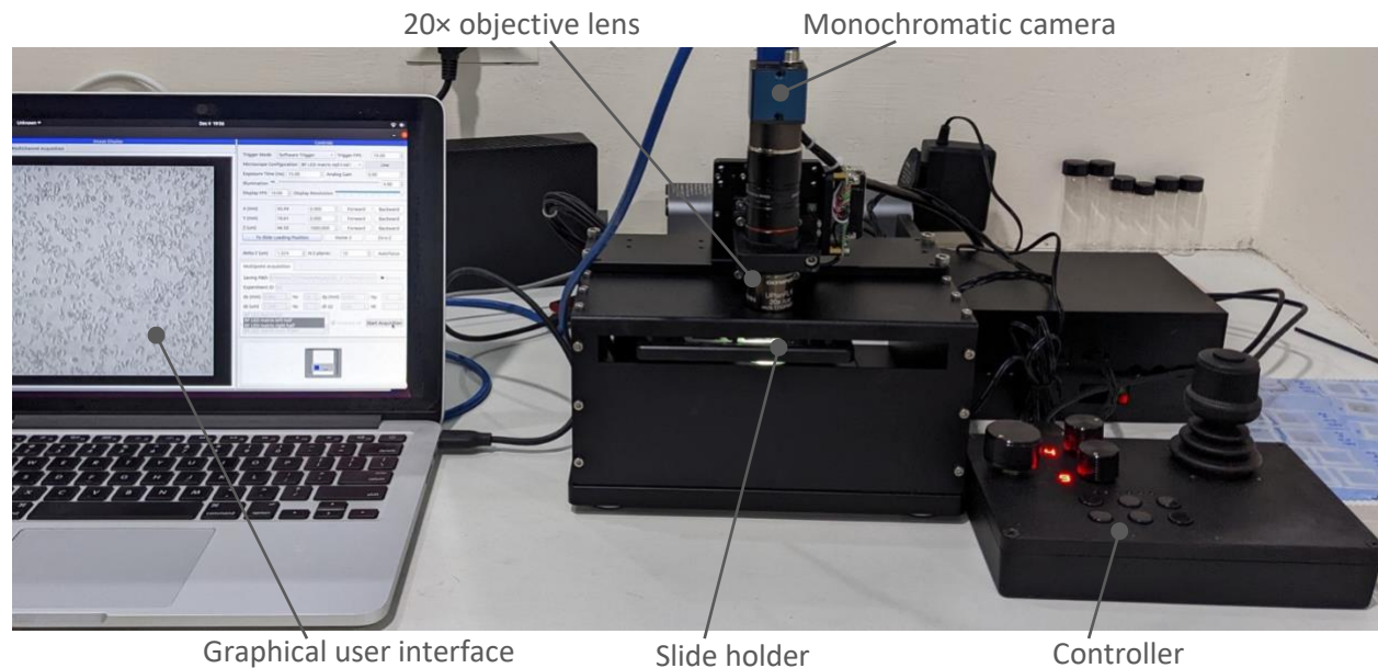
Fig. S1: Picture of the automated microscope, Octopi, during imaging of 225 images/coverslip at the study site in Nepal.
