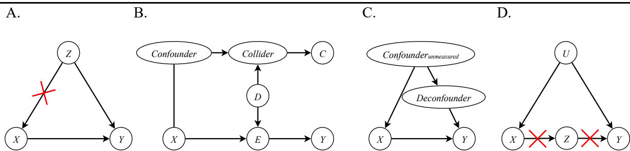
Fig. B4.1 Different positions of a confounder in the DAG structure require different confounder adjustment strategies.
