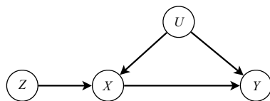
Fig. B4.2 DAG of instrumental variable Z
