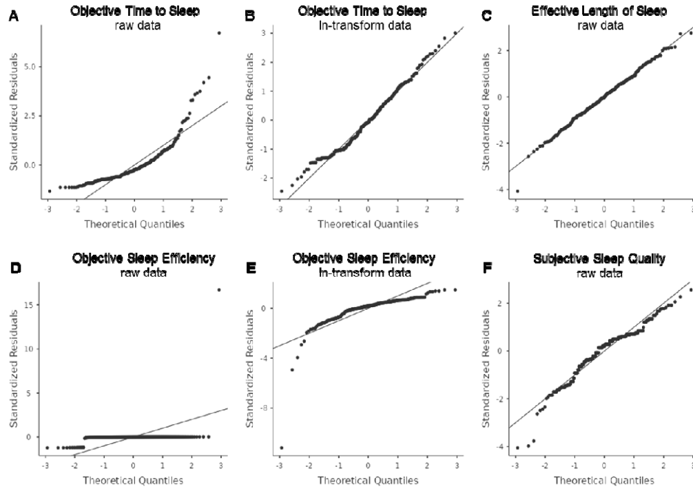
Figure 1. Q-Q plots of normality of observed data.
