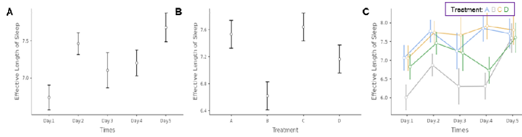
Figure 3. Comparison of subgroups of estimated marginal means of effective sleep duration.
