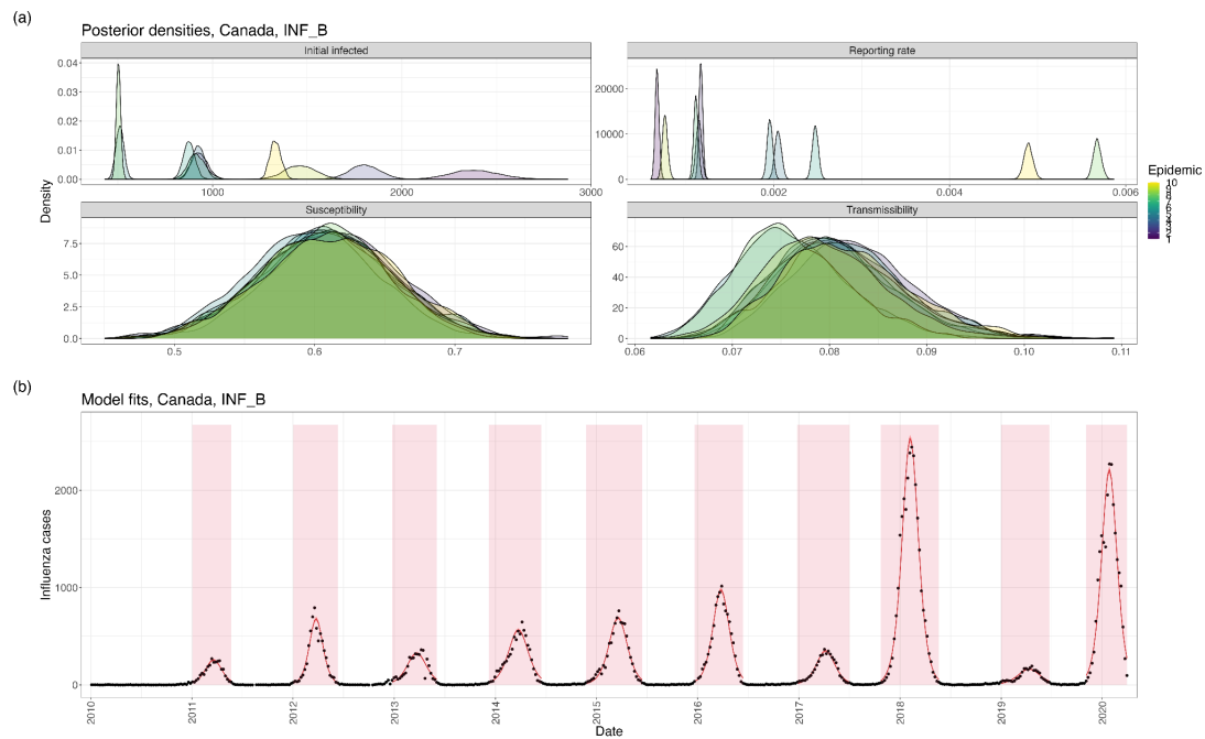
Figure S10: (a) Posterior distributions of the initial number of infections, reporting rate, population-level susceptibility, and influenza transmissibility in each epidemic used for inference (Canada, Influenza B). (b) Model fits using parameter posteriors.
