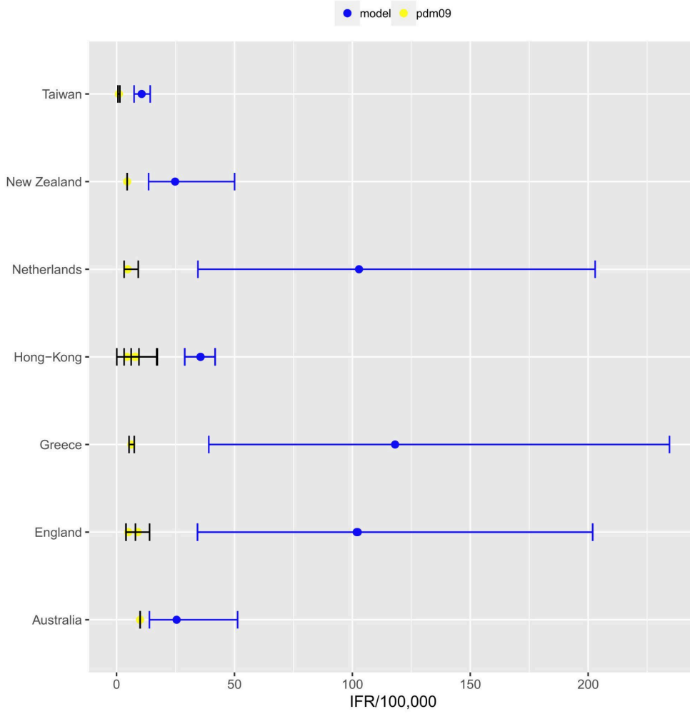
Figure S51: Forest plot of A(H1N1) 2009 pandemic influenza IFR estimates from empirical studies and from the seasonal influenza model.
