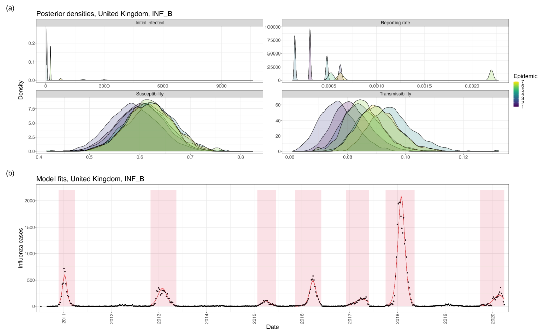
Figure S18: (a) Posterior distributions of the initial number of infections, reporting rate, population-level susceptibility, and influenza transmissibility in each epidemic used for inference (United Kingdom, Influenza B). (b) Model fits using parameter posteriors.
