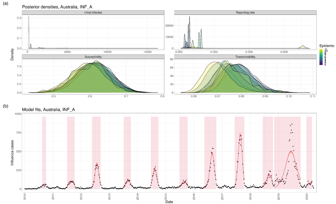
Figure S7: (a) Posterior distributions of the initial number of infections, reporting rate, population-level susceptibility, and influenza transmissibility in each epidemic used for inference (Australia, Influenza A). (b) Model fits using parameter posteriors.
