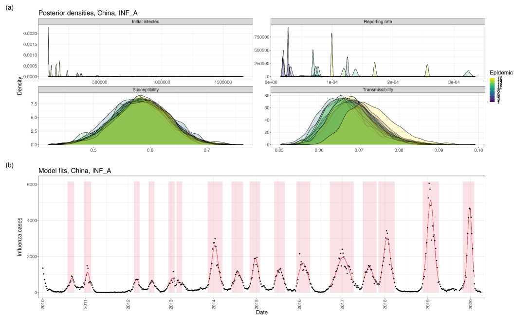
Figure S11: (a) Posterior distributions of the initial number of infections, reporting rate, population-level susceptibility, and influenza transmissibility in each epidemic used for inference (China, Influenza A). (b) Model fits using parameter posteriors.
