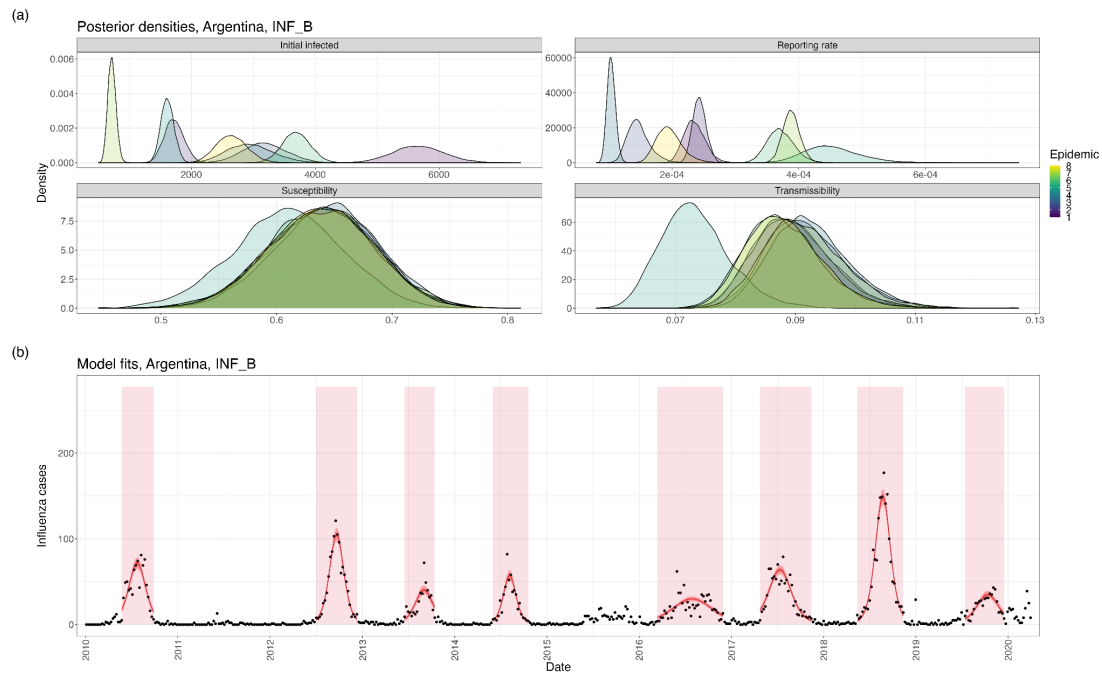
Figure S6: (a) Posterior distributions of the initial number of infections, reporting rate, population-level susceptibility, and influenza transmissibility in each epidemic used for inference (Argentina, Influenza B). (b) Model fits using parameter posteriors.
