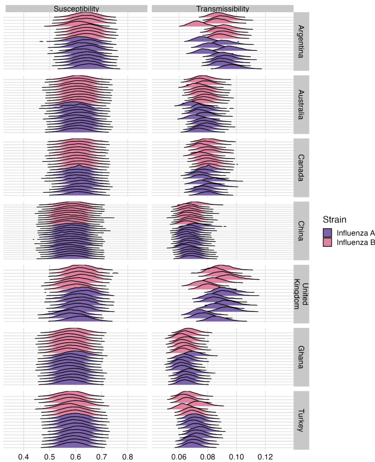
Figure S4: Posterior distributions of population-level susceptibility and influenza transmissibility in each epidemic used for inference.
