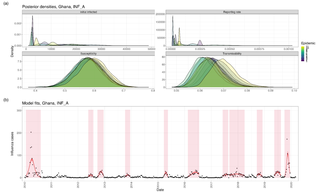
Figure S13: (a) Posterior distributions of the initial number of infections, reporting rate, population-level susceptibility, and influenza transmissibility in each epidemic used for inference (Ghana, Influenza A). (b) Model fits using parameter posteriors.
