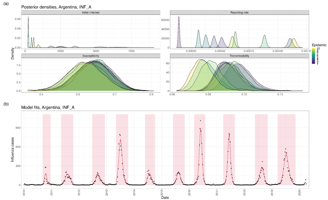
Figure S5: (a) Posterior distributions of the initial number of infections, reporting rate, population-level susceptibility, and influenza transmissibility in each epidemic used for inference (Argentina, Influenza A). (b) Model fits using parameter posteriors.
