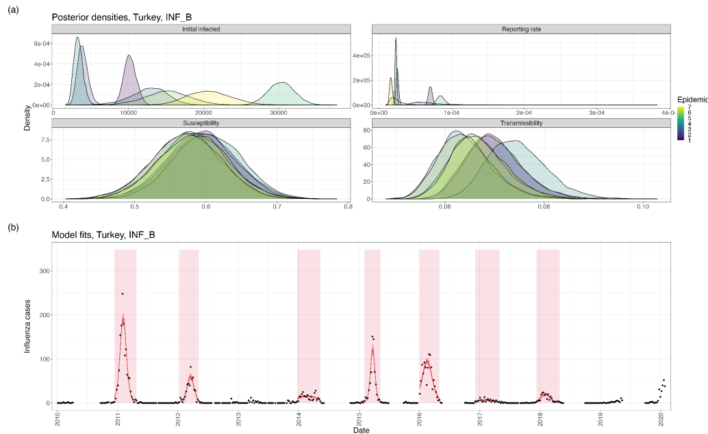
Figure S16: (a) Posterior distributions of the initial number of infections, reporting rate, population-level susceptibility, and influenza transmissibility in each epidemic used for inference (Turkey, Influenza B). (b) Model fits using parameter posteriors.
