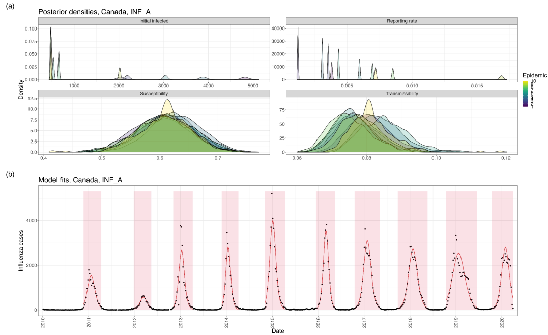
Figure S9: (a) Posterior distributions of the initial number of infections, reporting rate, population-level susceptibility, and influenza transmissibility in each epidemic used for inference (Canada, Influenza A). (b) Model fits using parameter posteriors.
