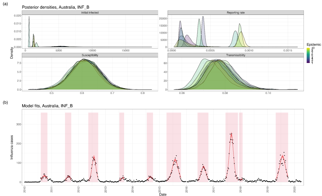
Figure S8: (a) Posterior distributions of the initial number of infections, reporting rate, population-level susceptibility, and influenza transmissibility in each epidemic used for inference (Australia, Influenza B). (b) Model fits using parameter posteriors.
