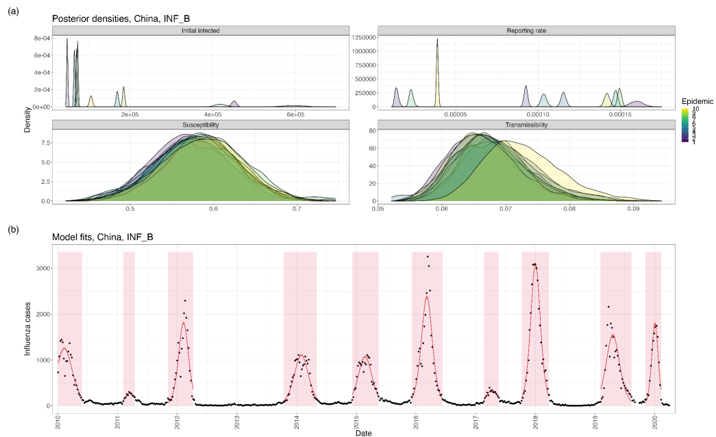
Figure S12: (a) Posterior distributions of the initial number of infections, reporting rate, population-level susceptibility, and influenza transmissibility in each epidemic used for inference (China, Influenza B). (b) Model fits using parameter posteriors.
