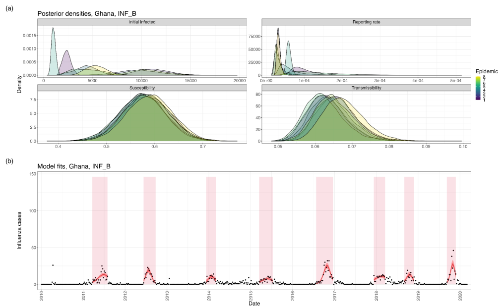
Figure S14: (a) Posterior distributions of the initial number of infections, reporting rate, population-level susceptibility, and influenza transmissibility in each epidemic used for inference (Ghana, Influenza B). (b) Model fits using parameter posteriors.
