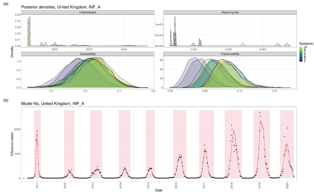
Figure S17: (a) Posterior distributions of the initial number of infections, reporting rate, population-level susceptibility, and influenza transmissibility in each epidemic used for inference (United Kingdom, Influenza A). (b) Model fits using parameter posteriors.
