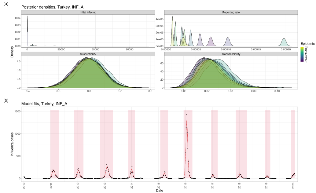
Figure S15: (a) Posterior distributions of the initial number of infections, reporting rate, population-level susceptibility, and influenza transmissibility in each epidemic used for inference (Turkey, Influenza A). (b) Model fits using parameter posteriors.
