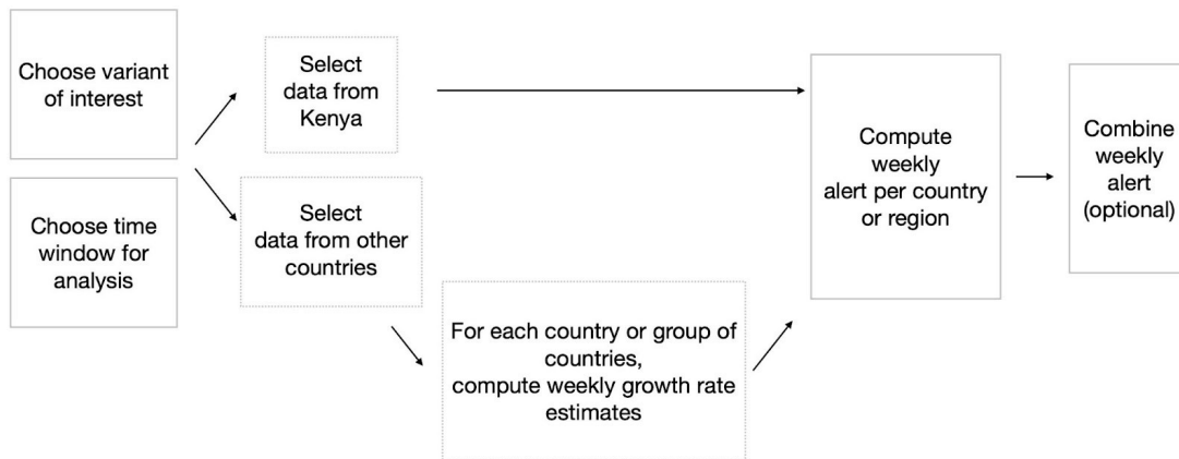
Figure 1. The process to estimate the growth of a variant in different countries or regions to produce a weekly warning signal.
