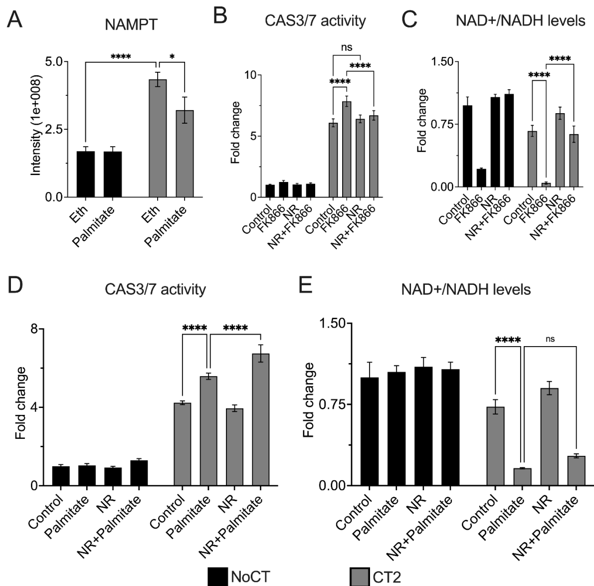
633 634 Figure 4 – Regulation of NAD metabolism in cytokine-mediated apoptosis by palmitate. MIN6 635 cells were treated with cytokine cocktail (CT2: 100 ng/mL IFN- \gamma , 10 ng/mL TNF- \alpha , and 5 ng/mL 636 IL-1 \beta ) in combination with 400 \mu M palmitate. (A) Levels of NAMPT measured by proteomics 637 analysis. Levels of apoptosis (measured by caspase 3/7 activity) (B) and NAD (C) in cells 638 treated with CT2 in combination with 10 \mu M NAMPT inhibitor FK866 and 100 \mu M nicotinamide 639 ribose (NR). Levels of apoptosis (measured by caspase 3/7 activity) (D) and NAD (E) in cells 640 treated with CT2 + 400 \mu M palmitate in combination with 100 \mu M NR. Additional abbreviations: 641 NoCT – no cytokine treatment control, Eth – ethanol vehicle control. 2-way ANOVA, Šídák's 642 multiple comparisons test: * p \leq 0.05 , ** p \leq 0.01 , *** p \leq 0.001 , **** p \leq 0.0001 .
