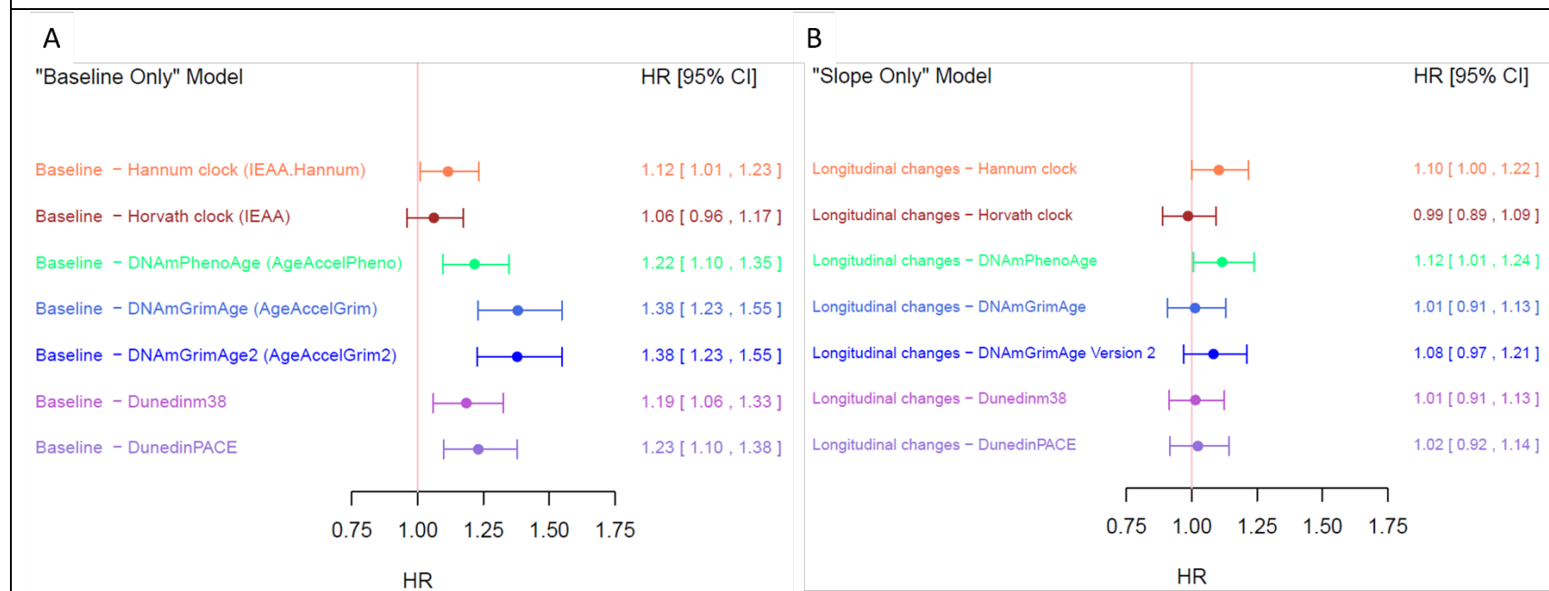
Figure 2. Forest Plot for the Adjusted Hazard Ratios of Mortality
