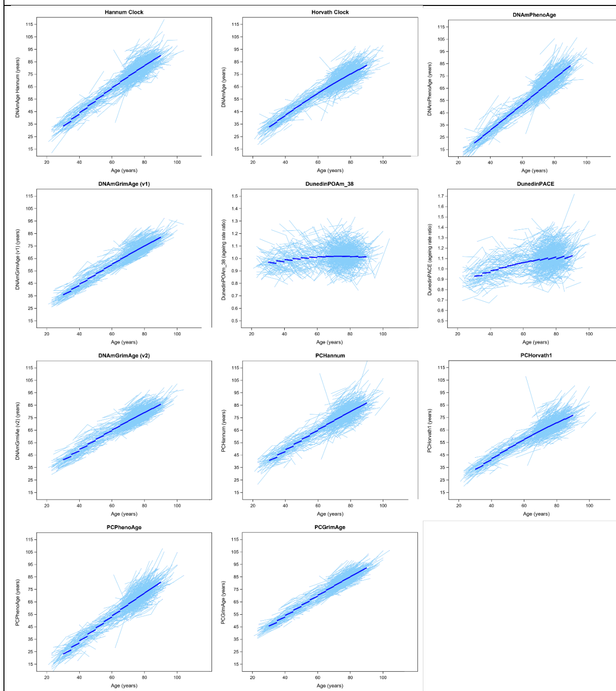
Figure 1. Longitudinal trajectories of epigenetic clocks
