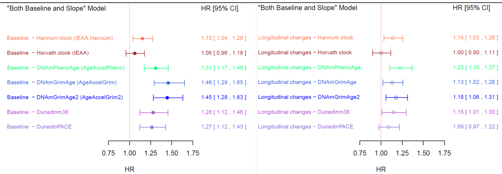
Figure 3. Forest Plot for the Adjusted Hazard Ratios of Mortality when both Baseline and Longitudinal Changes are included in the model
