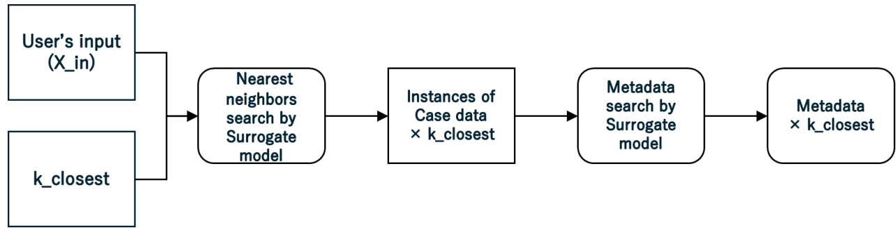
225 Fig 5 Activity diagram of explanation
