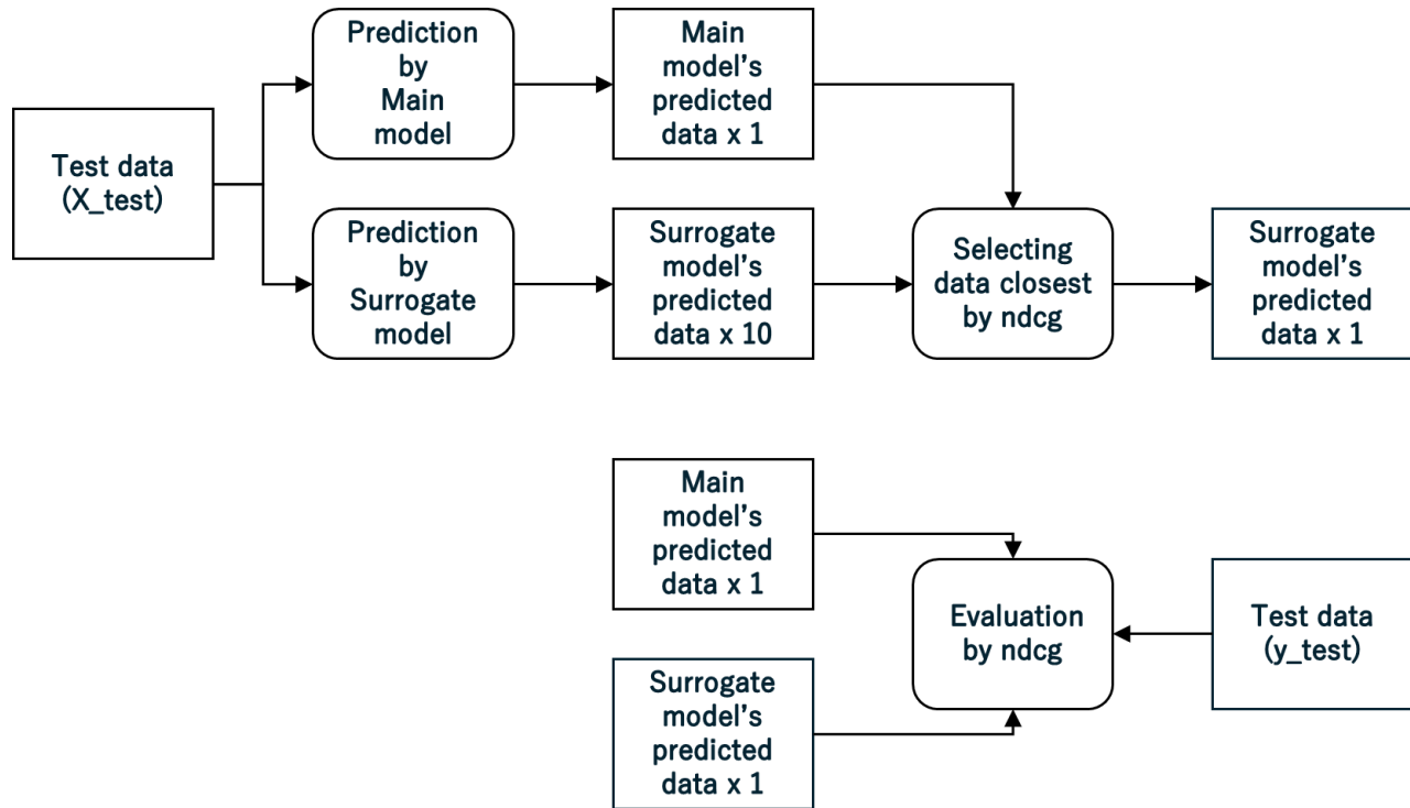
233 Fig 6 Activity diagram of evaluation
