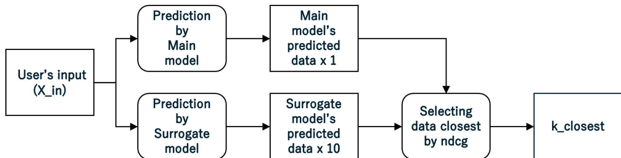
221 Fig 4 Activity diagram of prediction
