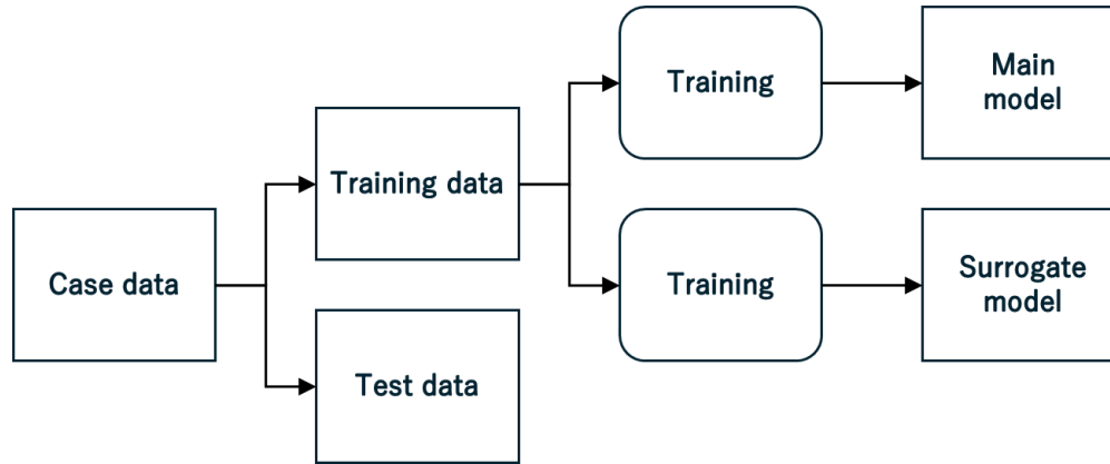
214 Fig 3 Activity diagram of training
