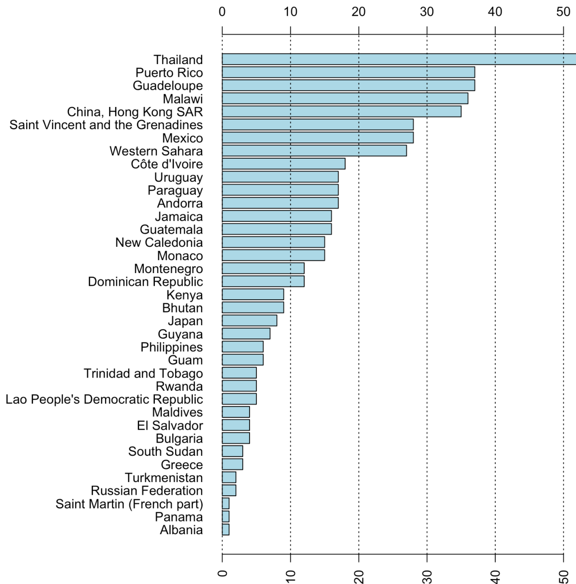
Figure S2. Incidence of top 10 rankings for centenarian attainment across 1970-2021. Despite the seemingly highly random composition of countries that attain the most remarkable late-life survival across the globe, rankings across consecutive cohorts are highly consistent. This is evident in the frequency with which several countries have retained top 10 rankings for late-life survival across the 51 years of available UN data. Thailand occupies a top 10 spot every year, closely followed by Puerto Rico, Guadeloupe, and Malawi with over 30 appearances each. Some countries, such as the Russian Federation, fell out of the rankings when they cease to exist, while others like South Sudan are recently created states. This ranking consistency rules out stochastic or sampling processes as a cause of these rankings, as age 100+ populations undergo complete replacement every 5-10 years.
