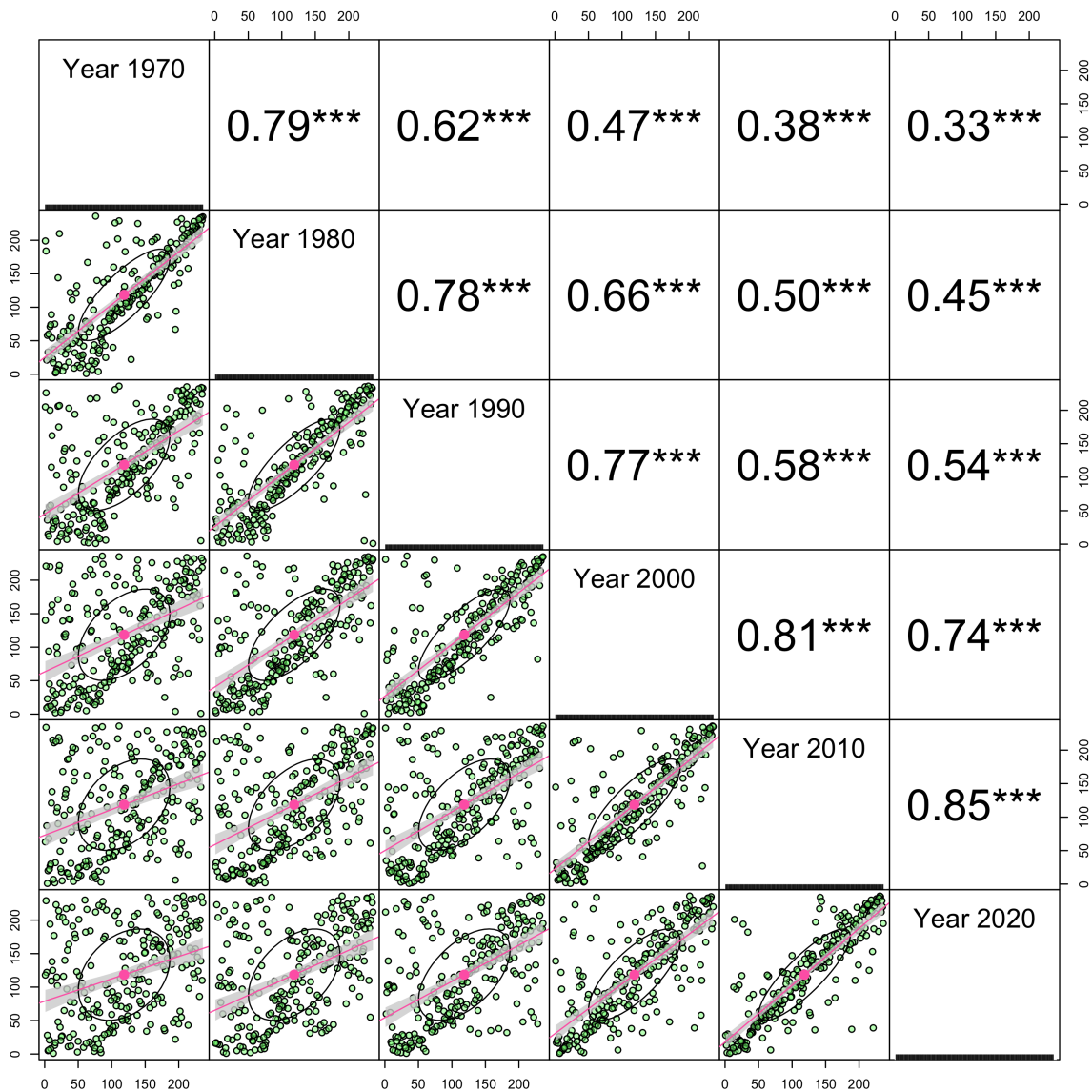
630 Figure 3. Rank concordance across non-overlapping cohorts of the oldest old. The ranks for centenarian attainment – survival rates from age 80 to ages 100+ – remain consistent across sizeable gaps and degrade slowly over time, despite the complete replacement of cohorts. Shown here are rank concordance (below the diagonal; pink lines show linear least squares regressions; ranks shown on axis labels) and correlation coefficients for rank concordance (above the diagonal) across 10-year gaps. These data all but rule out sampling effects as the dominant driver of late-life mortality rankings: virtually every 100+ year old dies and is replaced each decade, yet there is persistent long-term concordance in late-life survival over a decade or more. This concordance is typically around R^2 = 0.8 across a one-decade gap and around half of the variance in late-life mortality remains after 30 years. This slow decay in concordance likely 635 640
