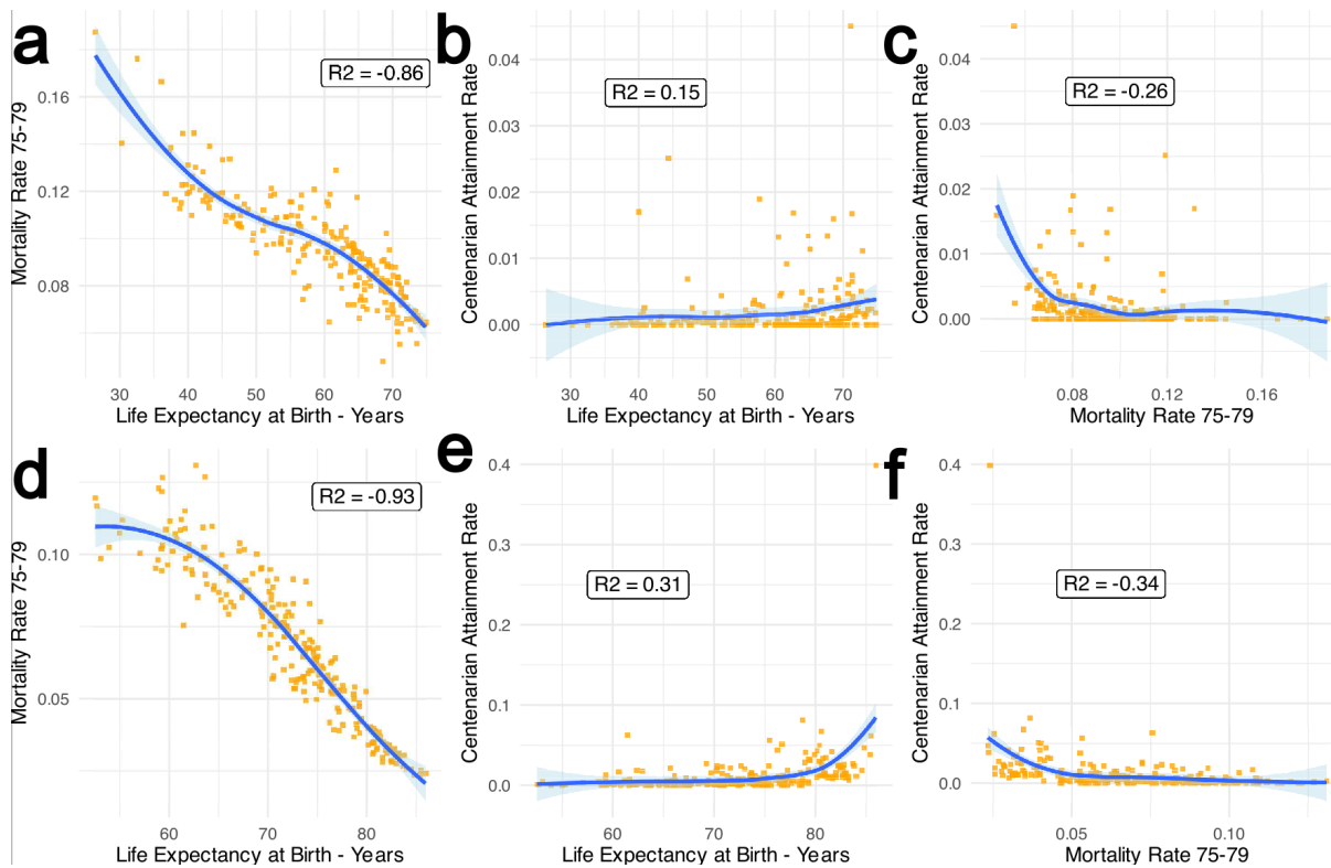
670 Figure S3. Consistently weak relationships between late-life survival or centenarian attainment rates and earlier-life survival over time. World Population Prospects data reveal the persistently weak relationship between early-life survival and centenarian attainment rates from the earliest (a-c) to the latest (2021 data, d-f) available mortality data. As expected, life expectancy at birth is strongly negatively 675 correlated with age-specific mortality rates until age 75-79 (a,d). Life expectancy at birth calculations include survival rates from ages 80-100+ and should, therefore, be highly negatively correlated. However, life expectancy at birth then has a persistently weak relationship with late-life survival and centenarian attainment rates from 1970 (b) to 2021 (e) despite orders-of-magnitude growth in the size of older populations. 680 Even mortality rates at age 75-79, immediately before ages 80-100+, display persistently weak correspondence with centenarian attainment rates (c,f). Such correlations between early- and late-life survival appear to be largely driven by a few low-mortality countries at the margin of the survival distribution (Supplementary Code; blue lines show locally weighted smoothed splines).
