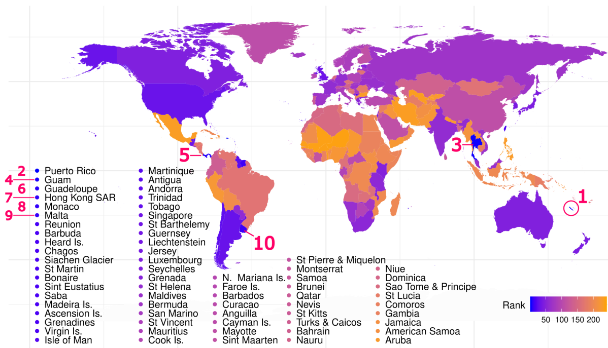
Figure S1. Patterns of UN-estimated life expectancy at age 100. World rankings of life expectancy at age 100, in years, derived from the 2021 UN World Population Prospects data 27 . Rankings for the ten longest-lived populations at age 100 are numbered.
