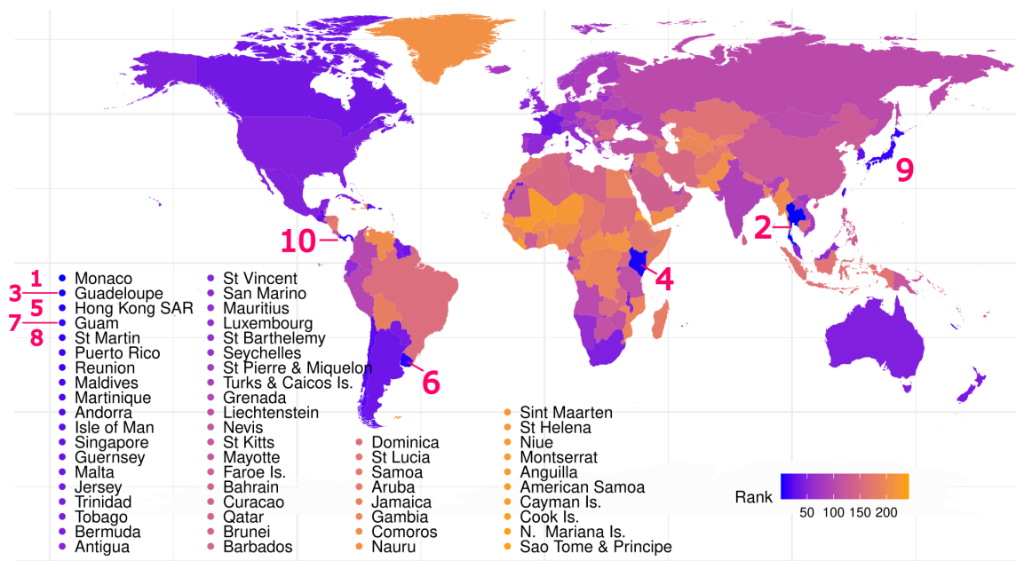
Figure 1. Centenarian attainment rates in 2021 United Nations data. Regions achieving the highest rate of cohort survival from ages 80 to 100+ years old – the centenarian attainment rate– are a highly irregular mix of states. For example, the top ten states globally for centenarian attainment (numbered) include both Monaco, with the highest life expectancy at birth in the world, and Kenya which is ranked 213 th in the world for life expectancy at birth. These rankings resemble unadjusted quinquennial UN figures for late-life survival – while being less model-dependent and less prone to sampling noise (Fig S1) – but have almost no resemblance to mortality or survival rates at any other age.
