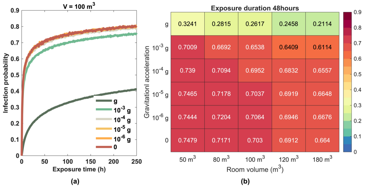
Fig S1: Infection probability under microgravity conditions. (a) Infection probability across various gravity levels as a function of exposure time. (b) Infection probability across different gravity levels and room volumes after 48 hours of exposure.
