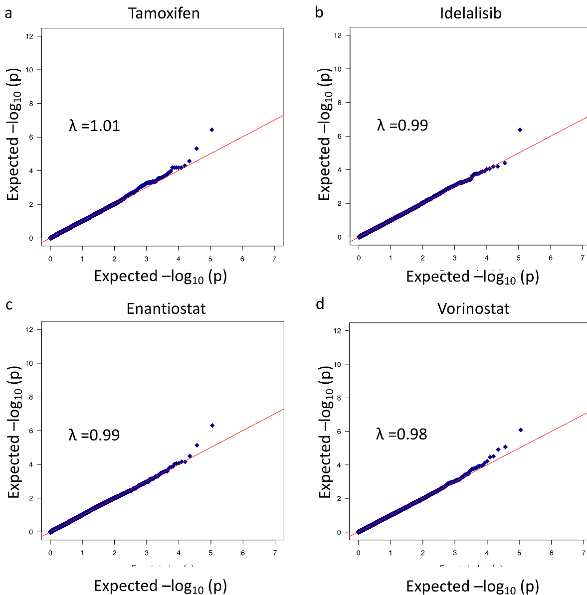
Supplementary Figure 2: QQ plot for the univariate GWAS associations
