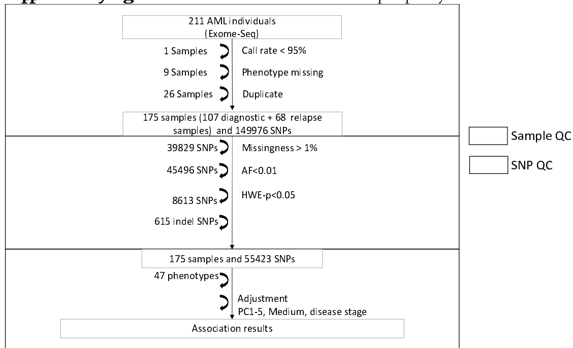
Supplementary Figure 1: Flow-chart for the SNP and sample quality control
