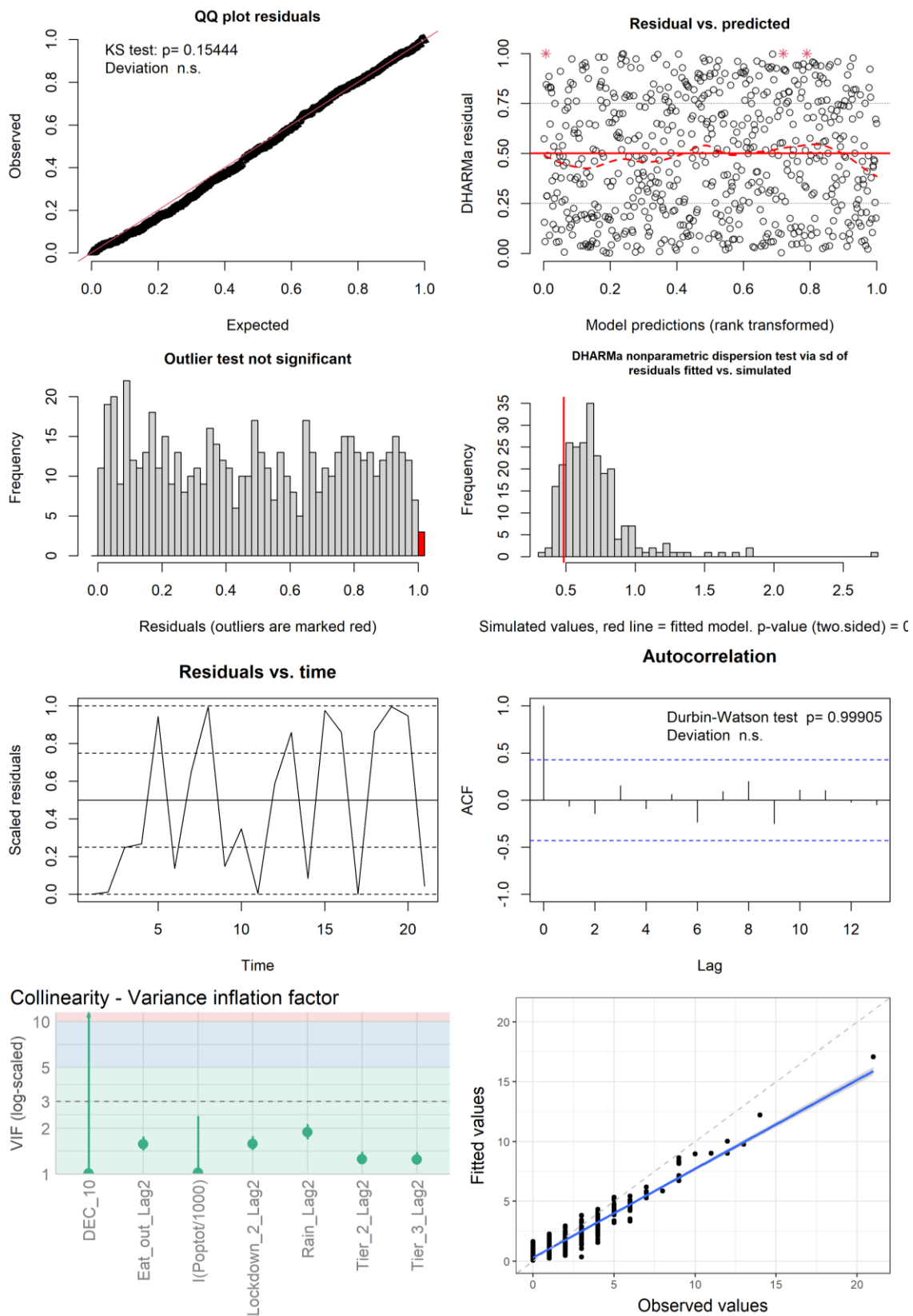
Figure S34: Figures used to assess model fit for the lineage B.1.177 GLMM with an AR1 term for week grouped by postcode. Temperature was dropped from this final model due to collinearity. First row: QQ plot, residuals vs predicted. Second row: outlier check, dispersion check. Third row: residuals vs time, ACF. Bottom row: VIF, observed values vs fitted values from the model.
