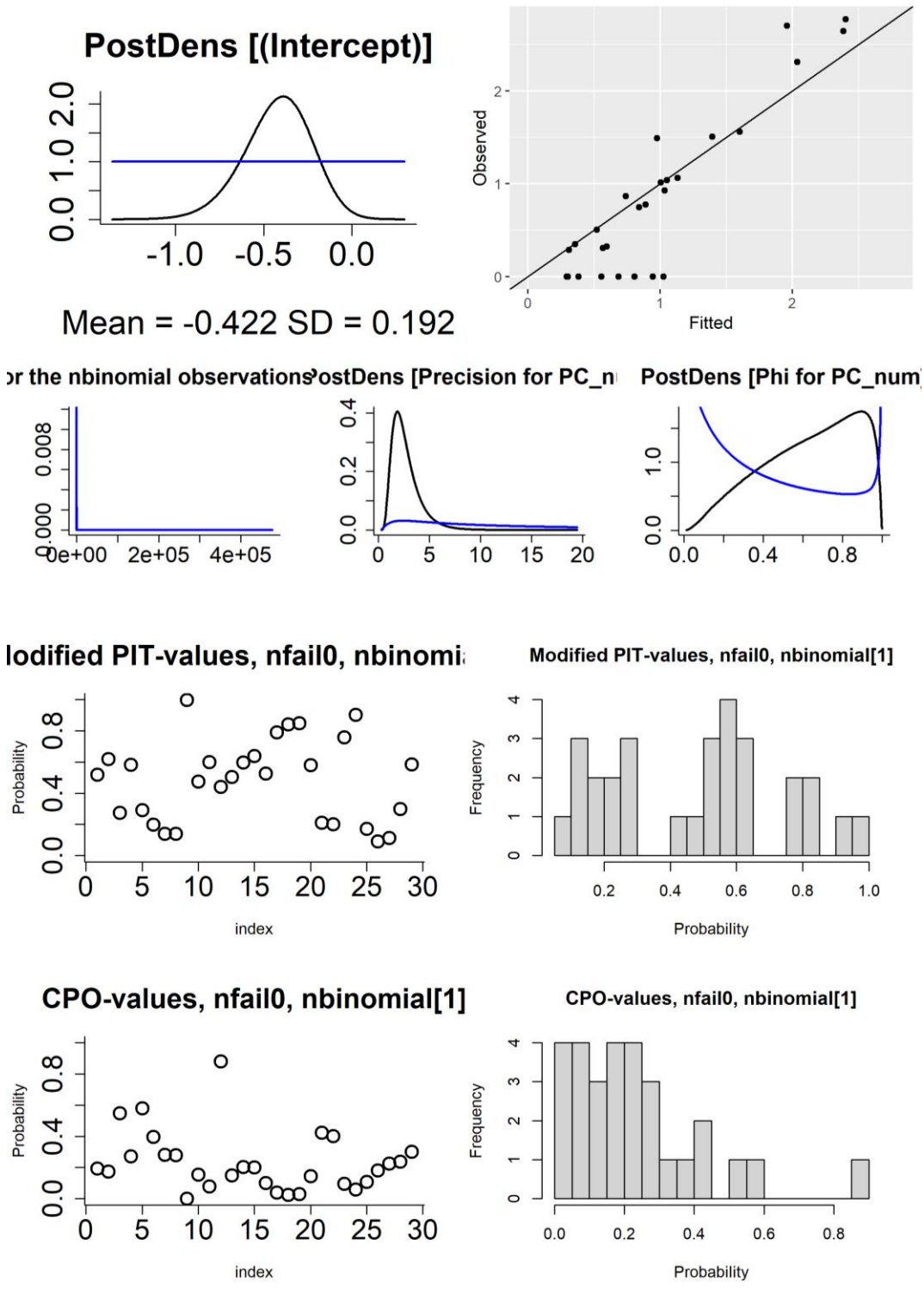
Figure S21: Figures used to assess model fit for the Lin52_B.1.177.10 disease mapping model, fit with default priors and other settings. First row: density of the posterior marginals of the intercept (including prior), observed vs fitted values. Second row: posterior density (and priors) of the hyperparameters (size for the negative binomial observations, and precision and phi for the BYM2 random effect). Third row: probability integral transforms (PIT) values (modified/adjusted version appropriate for count data) per postcode area, histogram of PIT values. Fourth row: conditional predictive ordinate (CPO) values per postcode area, histogram of CPO values.
