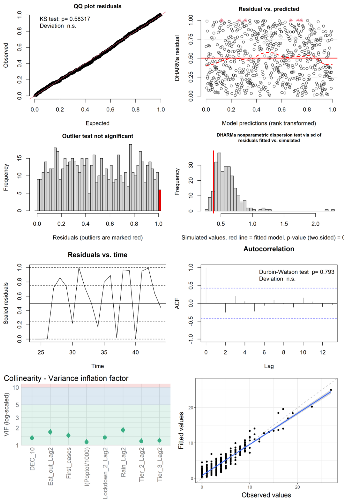
Figure S36: Figures used to assess model fit second-wave lineage cases GLMM with an AR1 term for week grouped by postcode. Temperature was dropped from this final model due to collinearity. First row: QQ plot, residuals vs predicted. Second row: outlier check, dispersion check. Third row: residuals vs time, ACF. Bottom row: VIF, observed values vs fitted values from the model.
