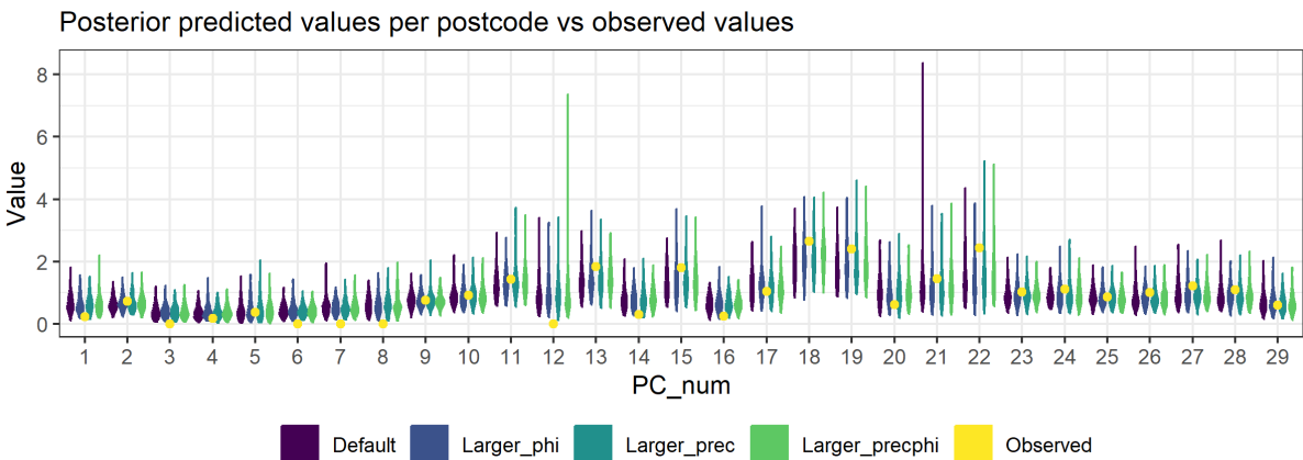
Figure S18: Figures used to assess model fit and sensitivity to hyperparameter values for the Lin45_B.1.1.7 disease mapping model, fit with the “laplace” approximation method. These plots compare the values for 4 models, each fit with different hyperparameter values (see section 2.2 above and model code in the analysis repository ( https://doi.org/10.25405/data.ncl.23815077 )). First row: density of the posterior marginals of the intercept and phi and precision hyperparameters. Second row: Mean and 97.5% quantiles for the intercept, comparison of the observed values to a sample generated from the posterior distribution. Third row: comparison of the observed values per postcode area to a sample generated from the posterior distribution (note that the numbers on the x axis do not correspond to the actual postcode numbers).
