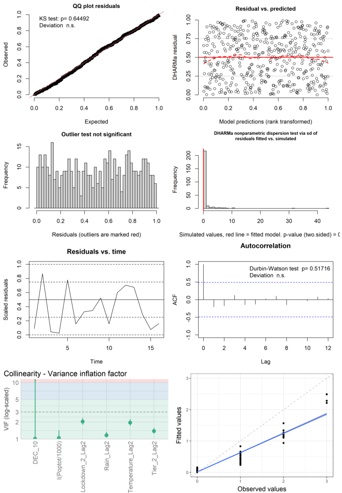
Figure S32: Figures used to assess model fit for the lineage B.1.1.37 GLMM with an AR1 term for week grouped by postcode. The eat-out subsidy was dropped from this final model due to collinearity. First row: QQ plot, residuals vs predicted. Second row: outlier check, dispersion check. Third row: residuals vs time, ACF. Bottom row: VIF, observed values vs fitted values from the model.
