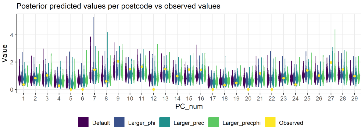
Figure S12: Figures used to assess model fit and sensitivity to hyperparameter values for the Lin35_B.1.1.309 disease mapping model, fit with the “laplace” approximation method. These plots compare the values for 4 models, each fit with different hyperparameter values (see section 2.2 above and model code in the analysis repository ( https://doi.org/10.25405/data.ncl.23815077 )). First row: density of the posterior marginals of the intercept and phi and precision hyperparameters. Second row: Mean and 97.5% quantiles for the intercept, comparison of the observed values to a sample generated from the posterior distribution. Third row: comparison of the observed values per postcode area to a sample generated from the posterior distribution (note that the numbers on the x axis do not correspond to the actual postcode numbers).
