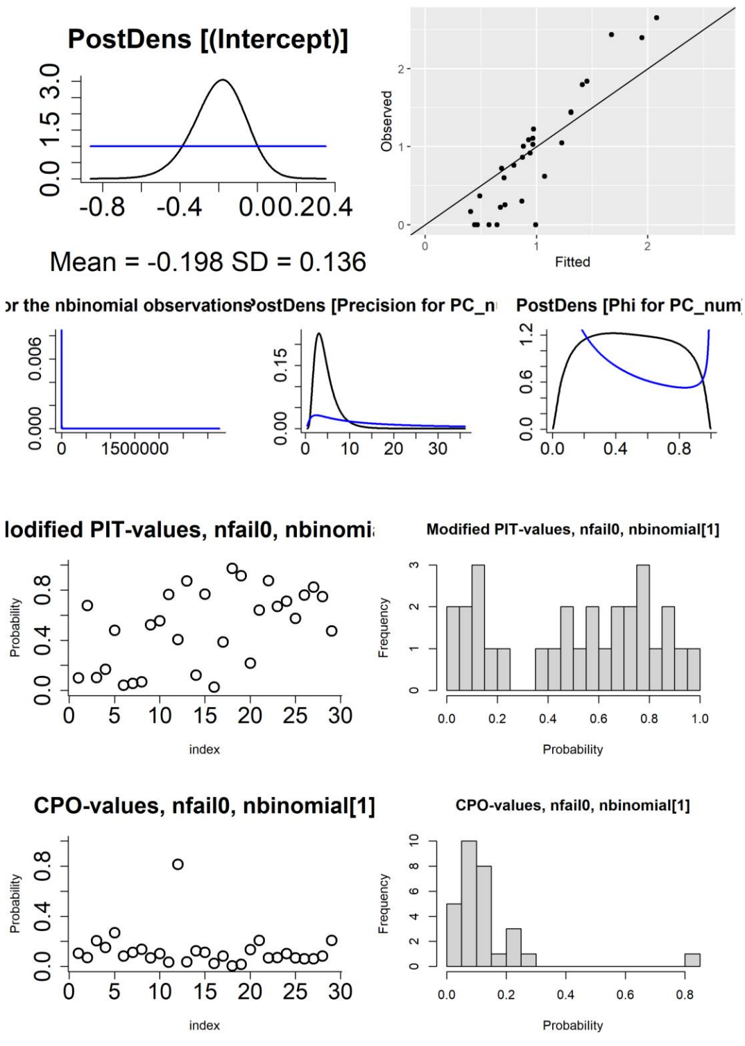
Figure S17: Figures used to assess model fit for the Lin45_B.1.1.7 disease mapping model, fit with default priors and other settings. First row: density of the posterior marginals of the intercept (including prior), observed vs fitted values. Second row: posterior density (and priors) of the hyperparameters (size for the negative binomial observations, and precision and phi for the BYM2 random effect). Third row: probability integral transforms (PIT) values (modified/adjusted version appropriate for count data) per postcode area, histogram of PIT values. Fourth row: conditional predictive ordinate (CPO) values per postcode area, histogram of CPO values.
