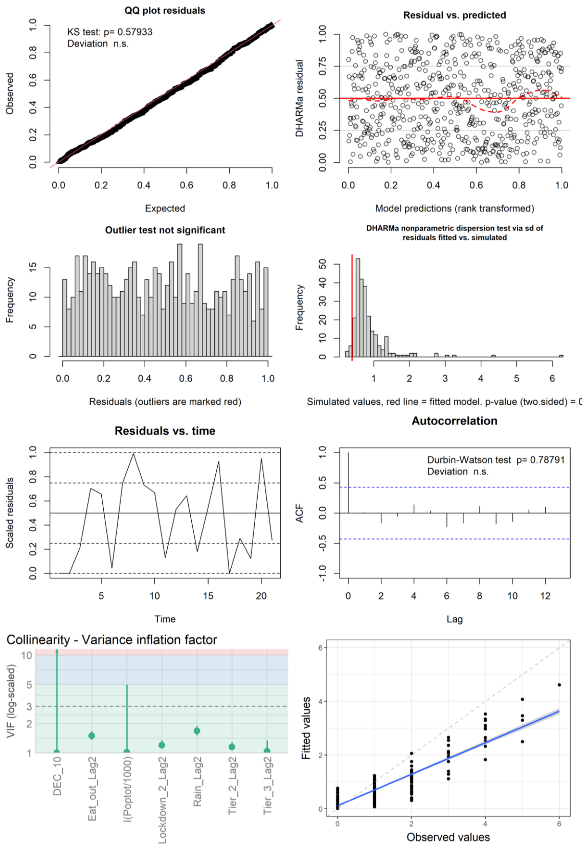
Figure S31: Figures used to assess model fit for the lineage B.1.1.315 GLMM with an AR1 term for week grouped by postcode. Temperature was dropped from this final model due to collinearity. First row: QQ plot, residuals vs predicted. Second row: outlier check, dispersion check. Third row: residuals vs time, ACF. Bottom row: VIF, observed values vs fitted values from the model.
