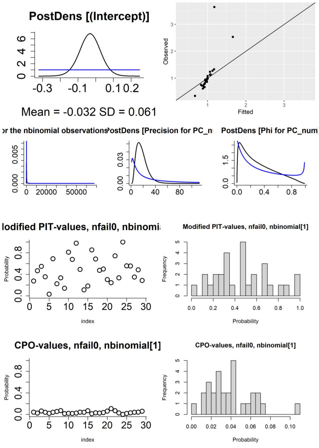
Figure S19: Figures used to assess model fit for the Lin51_B.1.177 disease mapping model, fit with default priors and other settings. First row: density of the posterior marginals of the intercept (including prior), observed vs fitted values. Second row: posterior density (and priors) of the hyperparameters (size for the negative binomial observations, and precision and phi for the BYM2 random effect). Third row: probability integral transforms (PIT) values (modified/adjusted version appropriate for count data) per postcode area, histogram of PIT values. Fourth row: conditional predictive ordinate (CPO) values per postcode area, histogram of CPO values.
