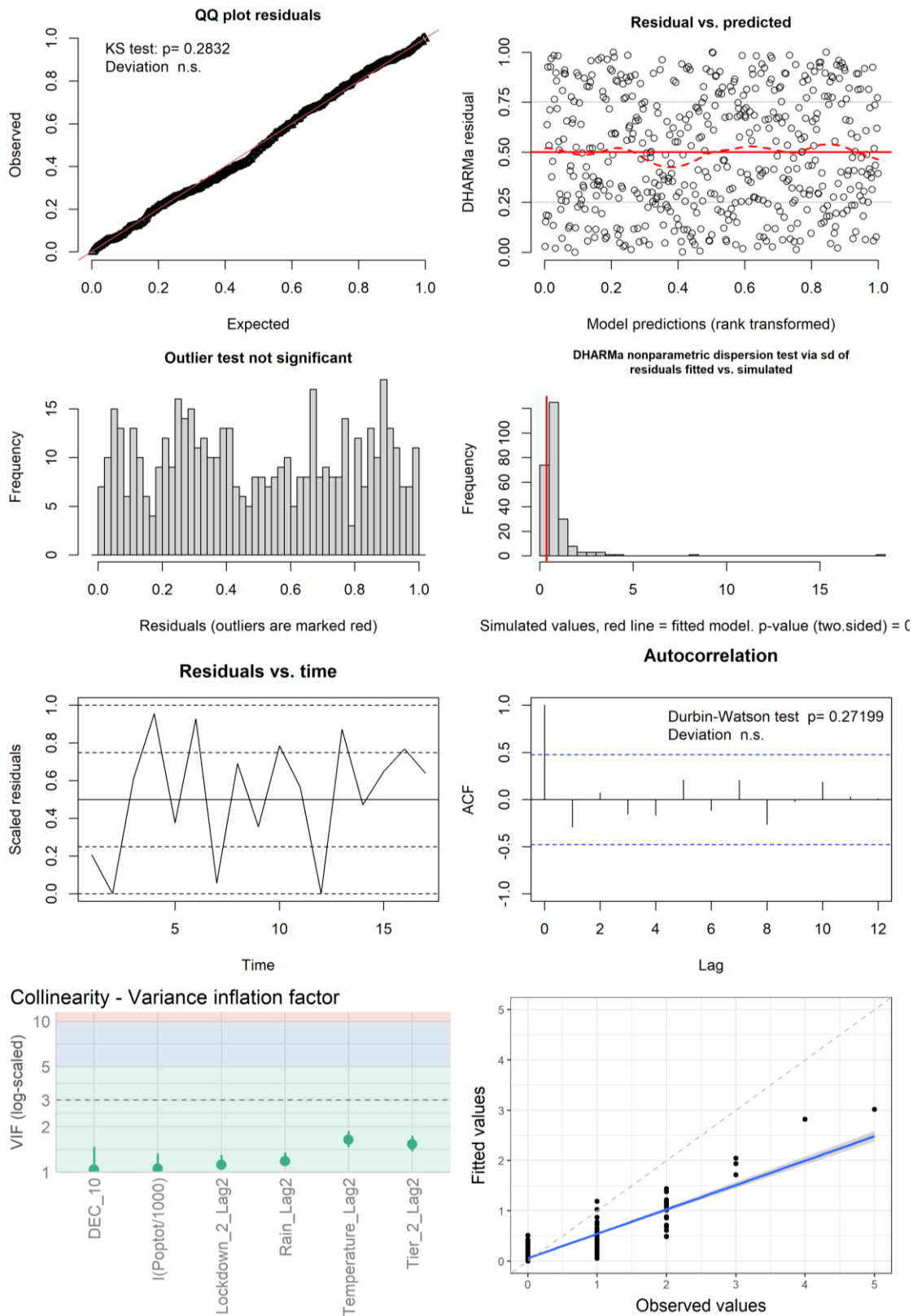
Figure S30: Figures used to assess model fit for the lineage B.1.1.309 GLMM with an AR1 term for week grouped by postcode. Eat-out subsidy was dropped from this final model due to collinearity. The random intercept for postcode was dropped due to poorer model fit. First row: QQ plot, residuals vs predicted. Second row: outlier check, dispersion check. Third row: residuals vs time, ACF. Bottom row: VIF, observed values vs fitted values from the model.
