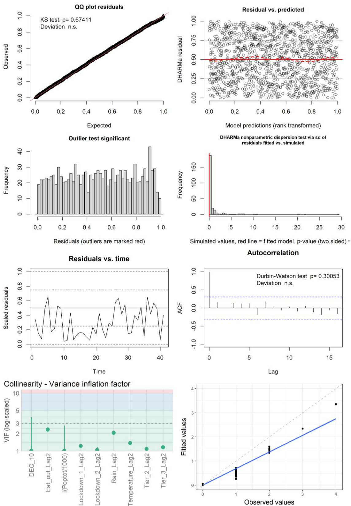
Figure S28: Figures used to assess model fit for the lineage B.1.1.1 GLMM with an AR1 term for week grouped by postcode. First row: QQ plot, residuals vs predicted. Second row: outlier check, dispersion check. Third row: residuals vs time, ACF. Bottom row: VIF, observed values vs fitted values from the model.
