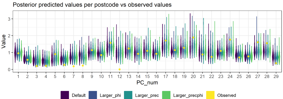
Figure S14: Figures used to assess model fit and sensitivity to hyperparameter values for the Lin37_B.1.1.315 disease mapping model, fit with the “laplace” approximation method. These plots compare the values for 4 models, each fit with different hyperparameter values (see section 2.2 above and model code in the analysis repository ( https://doi.org/10.25405/data.ncl.23815077 )). First row: density of the posterior marginals of the intercept and phi and precision hyperparameters. Second row: Mean and 97.5% quantiles for the intercept, comparison of the observed values to a sample generated from the posterior distribution. Third row: comparison of the observed values per postcode area to a sample generated from the posterior distribution (note that the numbers on the x axis do not correspond to the actual postcode numbers).
