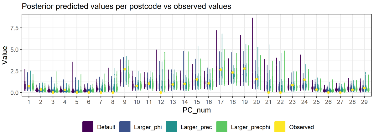
Figure S22: Figures used to assess model fit and sensitivity to hyperparameter values for the Lin52_B.1.177.10 disease mapping model, fit with the “laplace” approximation method. These plots compare the values for 4 models, each fit with different hyperparameter values (see section 2.2 above and model code in the analysis repository ( https://doi.org/10.25405/data.ncl.23815077 )). First row: density of the posterior marginals of the intercept and phi and precision hyperparameters. Second row: Mean and 97.5% quantiles for the intercept, comparison of the observed values to a sample generated from the posterior distribution. Third row: comparison of the observed values per postcode area to a sample generated from the posterior distribution (note that the numbers on the x axis do not correspond to the actual postcode numbers).
