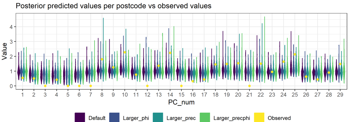
Figure S16: Figures used to assess model fit and sensitivity to hyperparameter values for the Lin39_B.1.1.37 disease mapping model, fit with the “laplace” approximation method. These plots compare the values for 4 models, each fit with different hyperparameter values (see section 2.2 above and model code in the analysis repository ( https://doi.org/10.25405/data.ncl.23815077 )). First row: density of the posterior marginals of the intercept and phi and precision hyperparameters. Second row: Mean and 97.5% quantiles for the intercept, comparison of the observed values to a sample generated from the posterior distribution. Third row: comparison of the observed values per postcode area to a sample generated from the posterior distribution (note that the numbers on the x axis do not correspond to the actual postcode numbers).
