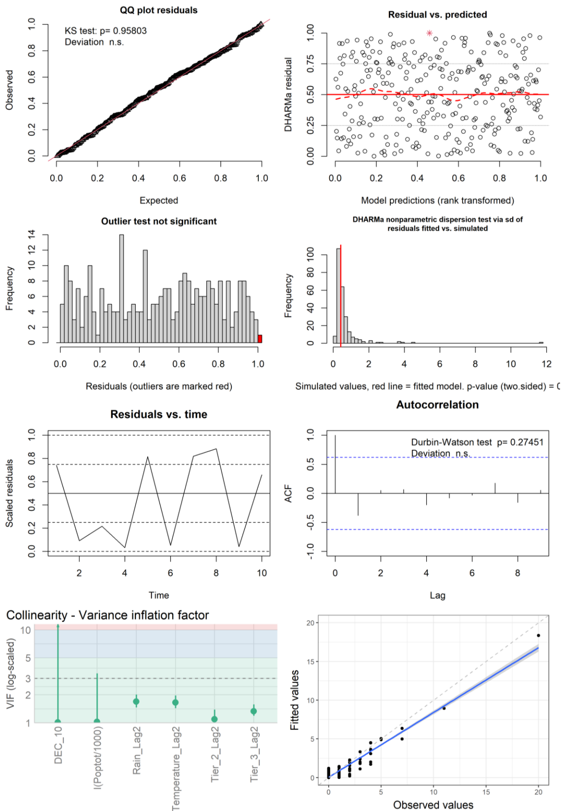
Figure S33: Figures used to assess model fit for the lineage B.1.1.7 GLMM with an AR1 term for week grouped by postcode. Lockdown 2 was dropped from this final model due to collinearity. First row: QQ plot, residuals vs predicted. Second row: outlier check, dispersion check. Third row: residuals vs time, ACF. Bottom row: VIF, observed values vs fitted values from the model.
