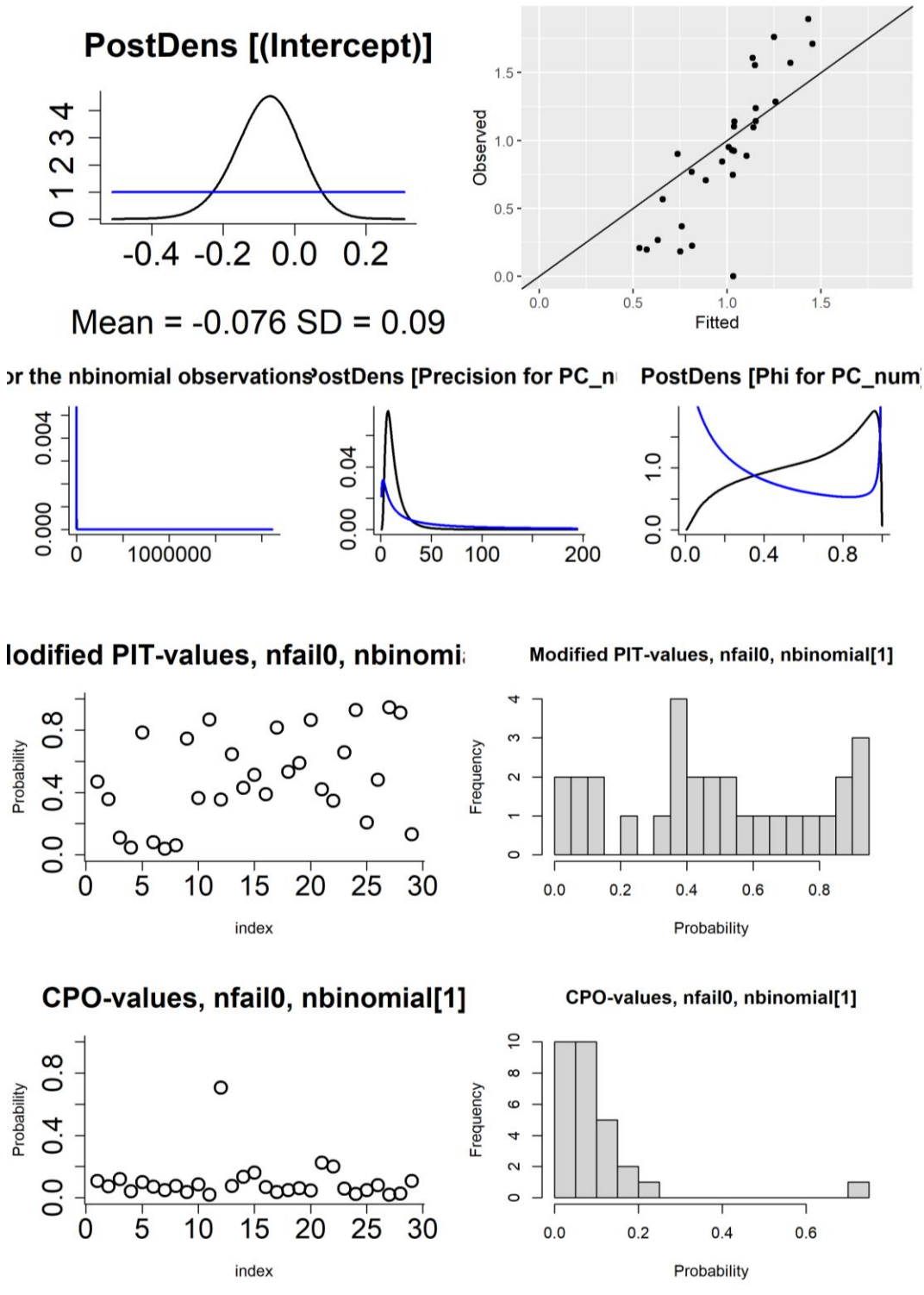
Figure S13: Figures used to assess model fit for the Lin37_B.1.1.315 disease mapping model, fit with default priors and other settings. First row: density of the posterior marginals of the intercept (including prior), observed vs fitted values. Second row: posterior density (and priors) of the hyperparameters (size for the negative binomial observations, and precision and phi for the BYM2 random effect). Third row: probability integral transforms (PIT) values (modified/adjusted version appropriate for count data) per postcode area, histogram of PIT values. Fourth row: conditional predictive ordinate (CPO) values per postcode area, histogram of CPO values.
