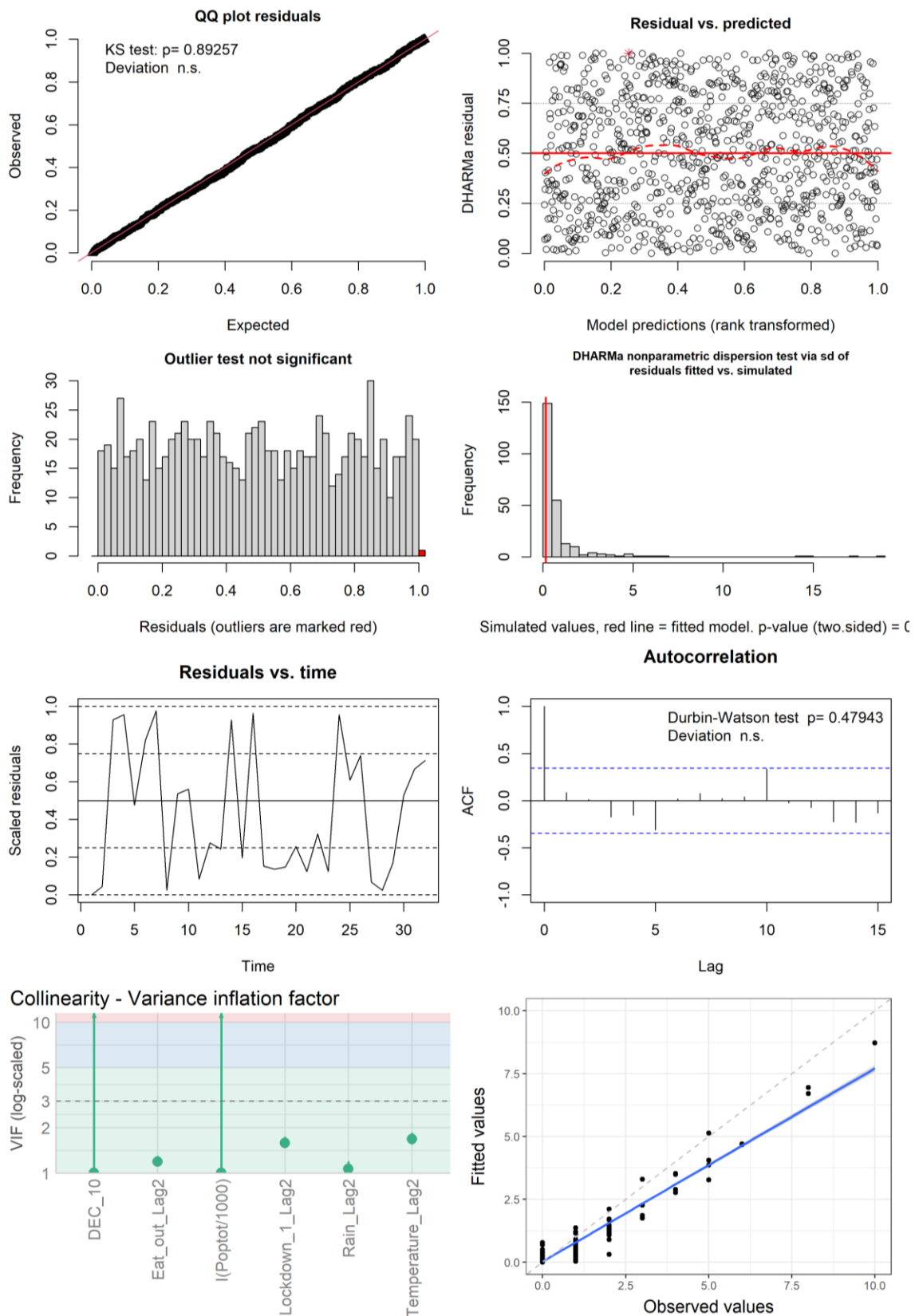
Figure S29: Figures used to assess model fit for the lineage B.1.1.119 GLMM with an AR1 term for week grouped by postcode. First row: QQ plot, residuals vs predicted. Second row: outlier check, dispersion check. Third row: residuals vs time, ACF. Bottom row: VIF, observed values vs fitted values from the model.
