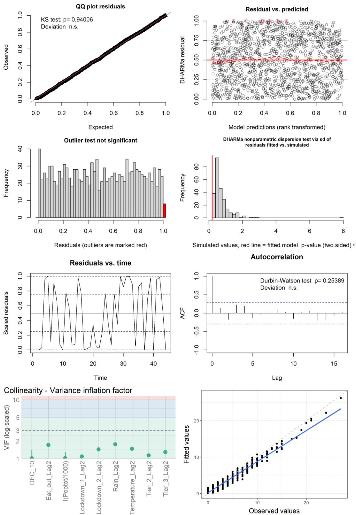
Figure S25: Figures used to assess model fit for the all-cases GLMM with an AR1 term for week grouped by postcode. First row: QQ plot, residuals vs predicted. Second row: outlier check, dispersion check. Third row: residuals vs time, ACF. Bottom row: VIF, observed values vs fitted values from the model.
