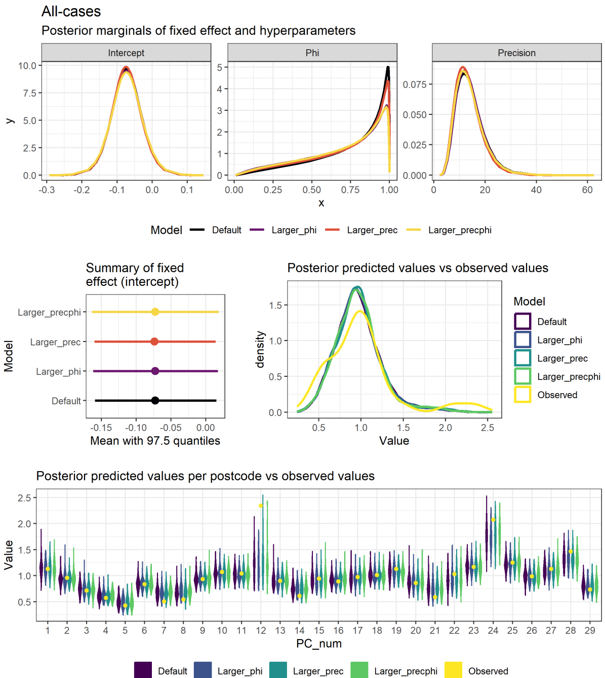
Figure S6: Figures used to assess model fit and sensitivity to hyperparameter values for the all-cases disease mapping model, fit with the “laplace” approximation method. These plots compare the values for 4 models, each fit with different hyperparameter values (see section 2.2 above and model code in the analysis repository ( https://doi.org/10.25405/data.ncl.23815077 )). First row: density of the posterior marginals of the intercept and phi and precision hyperparameters. Second row: Mean and 97.5% quantiles for the intercept, comparison of the observed values to a sample generated from the posterior distribution. Third row: comparison of the observed values per postcode area to a sample generated from the posterior distribution (note that the numbers on the x axis do not correspond to the actual postcode numbers).
