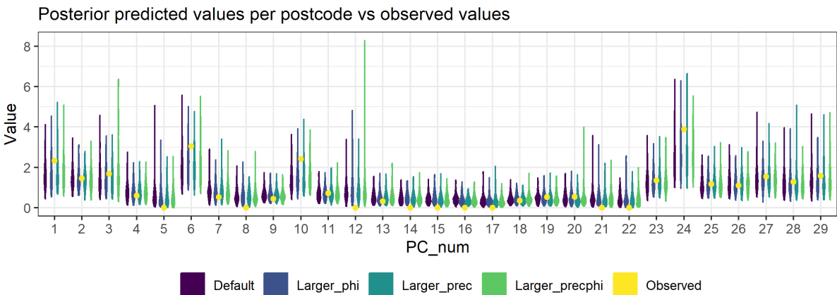
Figure S8: Figures used to assess model fit and sensitivity to hyperparameter values for the Lin6_B.1.1.1 disease mapping model, fit with the “laplace” approximation method. These plots compare the values for 4 models, each fit with different hyperparameter values (see section 2.2 above and model code in the analysis repository ( https://doi.org/10.25405/data.ncl.23815077 )). First row: density of the posterior marginals of the intercept and phi and precision hyperparameters. Second row: Mean and 97.5% quantiles for the intercept, comparison of the observed values to a sample generated from the posterior distribution. Third row: comparison of the observed values per postcode area to a sample generated from the posterior distribution (note that the numbers on the x axis do not correspond to the actual postcode numbers).
