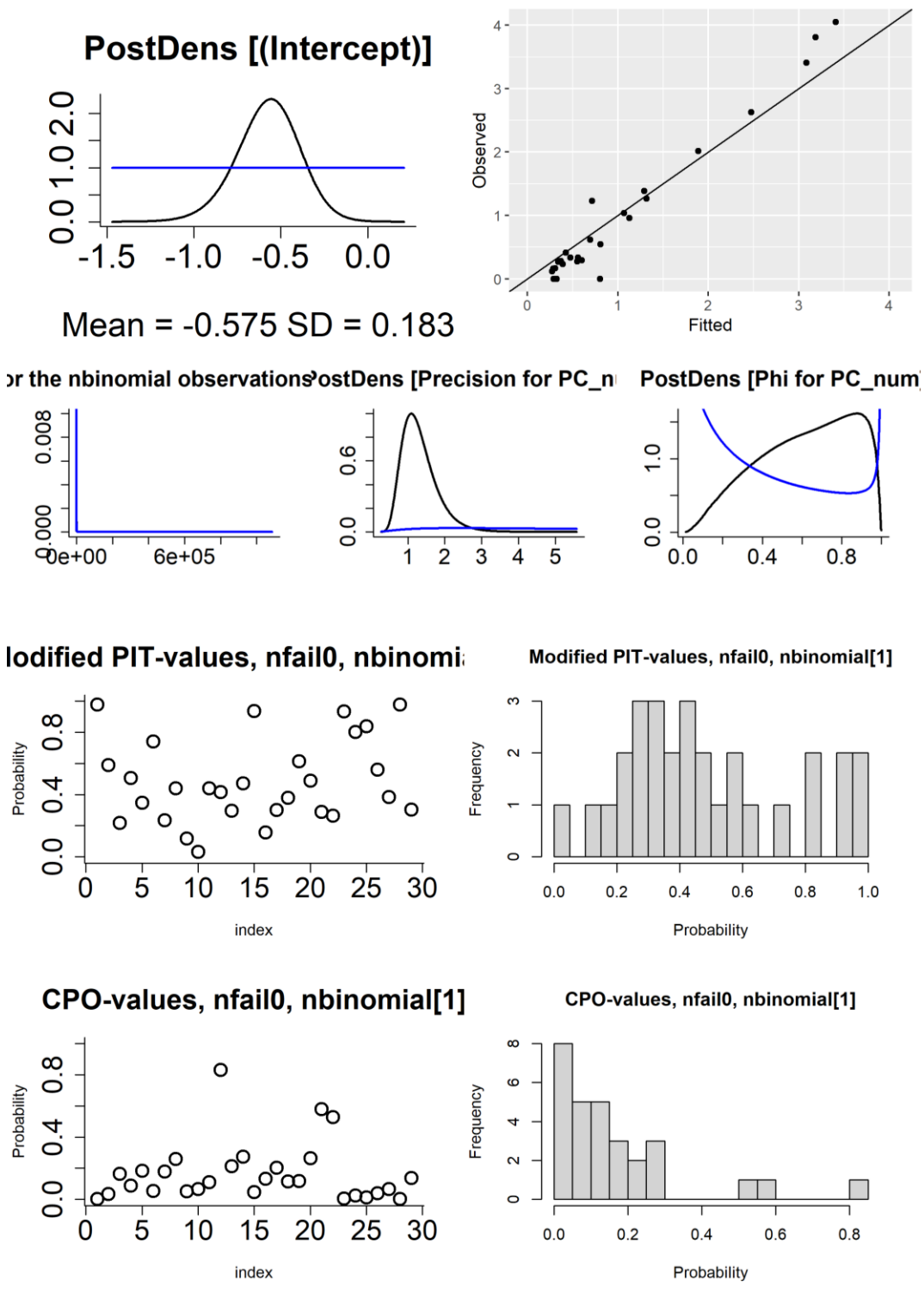
Figure S9: Figures used to assess model fit for the Lin10_B.1.1.119 disease mapping model, fit with default priors and other settings. First row: density of the posterior marginals of the intercept (including prior), observed vs fitted values. Second row: posterior density (and priors) of the hyperparameters (size for the negative binomial observations, and precision and phi for the BYM2 random effect). Third row: probability integral transforms (PIT) values (modified/adjusted version appropriate for count data) per postcode area, histogram of PIT values. Fourth row: conditional predictive ordinate (CPO) values per postcode area, histogram of CPO values.
