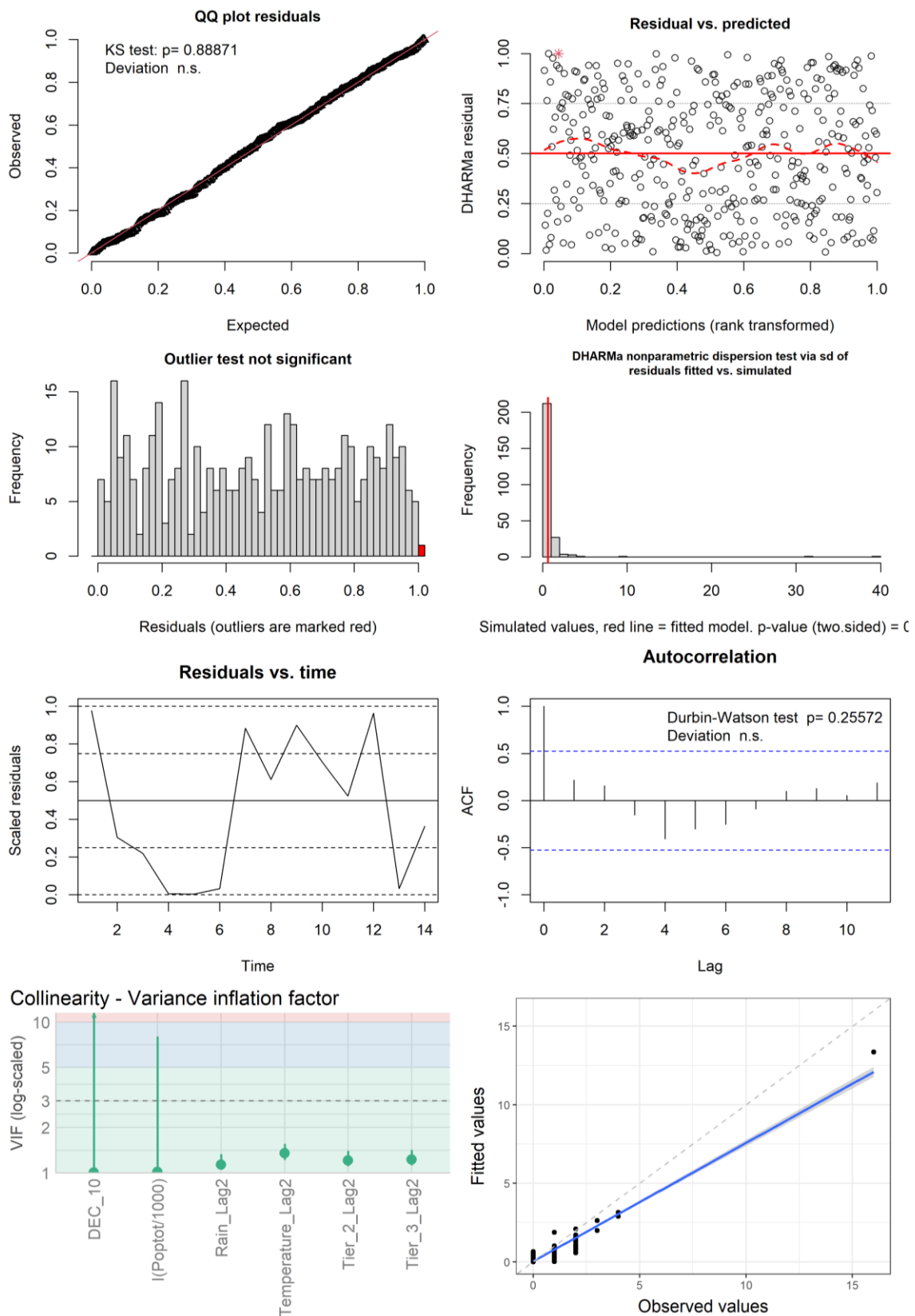
Figure S35: Figures used to assess model fit for the lineage B.1.177.10 GLMM with an AR1 term for week grouped by postcode. Lockdown 2 was dropped from this final model due to collinearity. First row: QQ plot, residuals vs predicted. Second row: outlier check, dispersion check. Third row: residuals vs time, ACF. Bottom row: VIF, observed values vs fitted values from the model.
