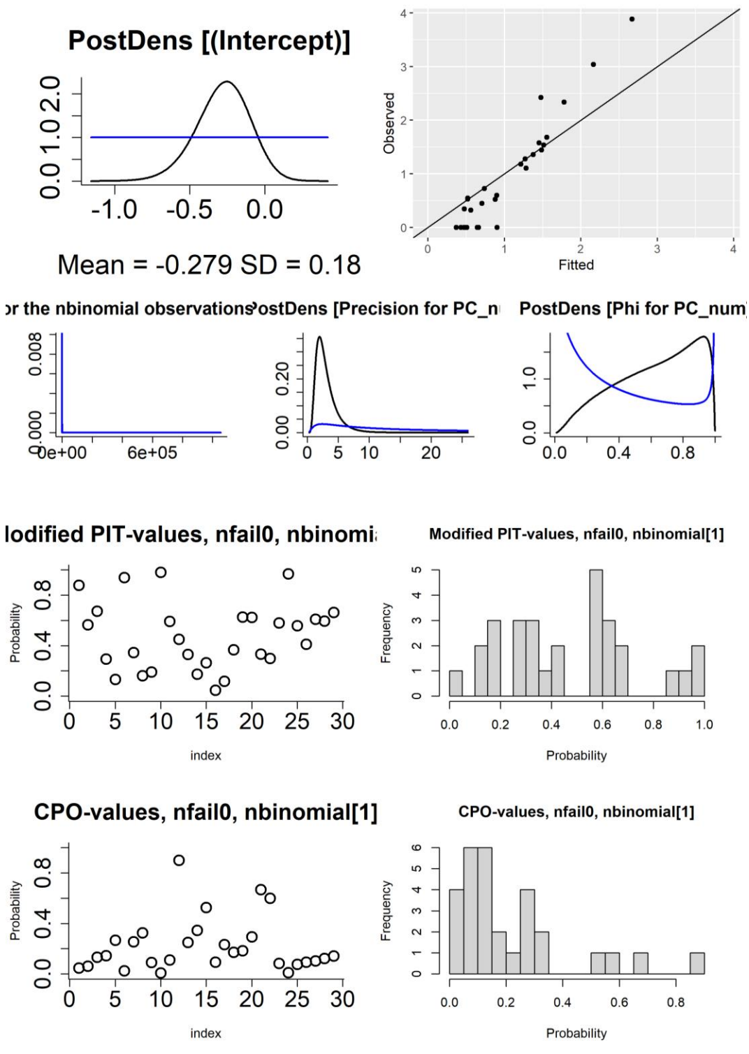
Figure S7: Figures used to assess model fit for the Lin6_B.1.1.1 disease mapping model, fit with default priors and other settings. First row: density of the posterior marginals of the intercept (including prior), observed vs fitted values. Second row: posterior density (and priors) of the hyperparameters (size for the negative binomial observations, and precision and phi for the BYM2 random effect). Third row: probability integral transforms (PIT) values (modified/adjusted version appropriate for count data) per postcode area, histogram of PIT values. Fourth row: conditional predictive ordinate (CPO) values per postcode area, histogram of CPO values.
