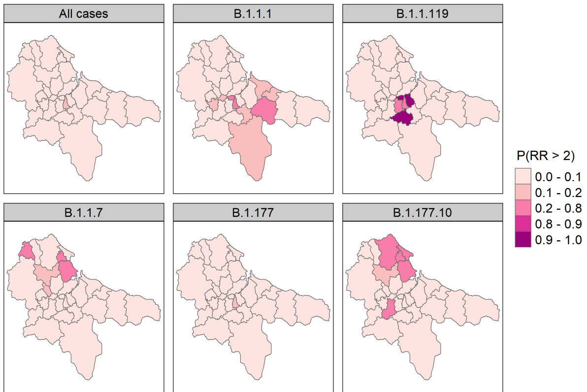
Figure S2: Map of the exceedance probabilities for relative risk threshold of 2. Relative risk is very likely to exceed 2 when probabilities are close to 1, and very unlikely when values are close to 0 (values around 0.5 have the highest uncertainty). Maps for 3 of the lineages are not shown due to poor model fit (B.1.1.309, B.1.1.315, and B.1.1.37).
