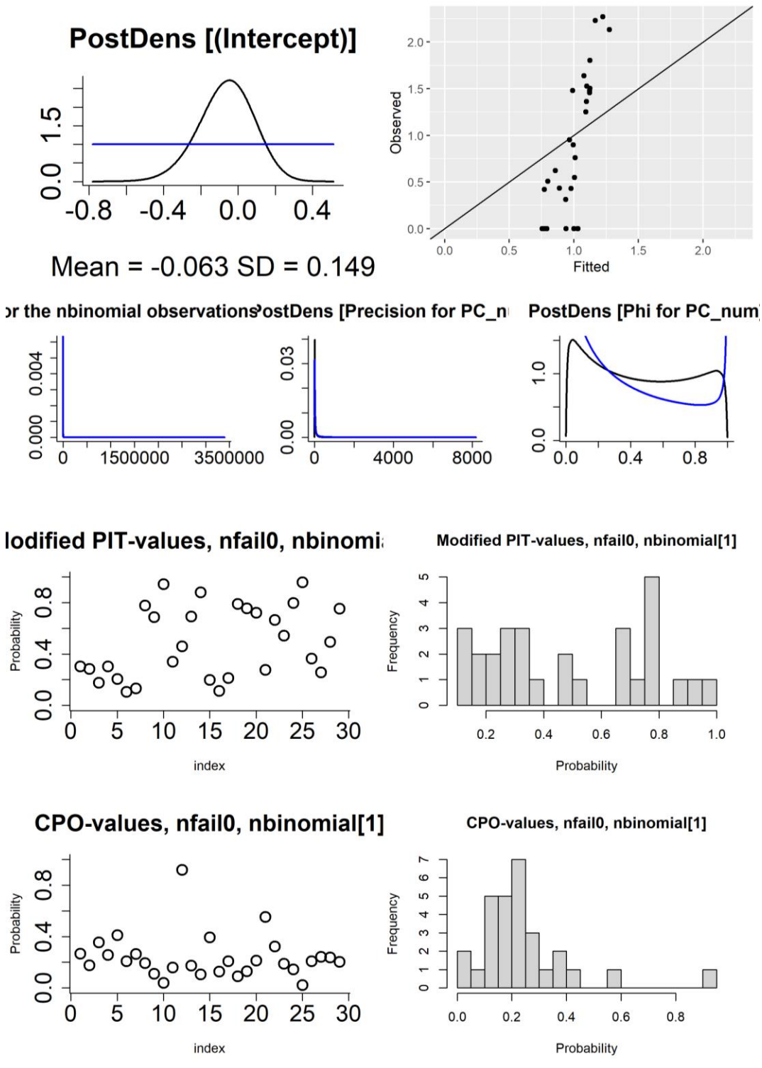
Figure S15: Figures used to assess model fit for the Lin39_B.1.1.37 disease mapping model, fit with default priors and other settings. First row: density of the posterior marginals of the intercept (including prior), observed vs fitted values. Second row: posterior density (and priors) of the hyperparameters (size for the negative binomial observations, and precision and phi for the BYM2 random effect). Third row: probability integral transforms (PIT) values (modified/adjusted version appropriate for count data) per postcode area, histogram of PIT values. Fourth row: conditional predictive ordinate (CPO) values per postcode area, histogram of CPO values.
