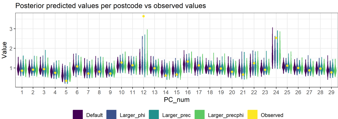
Figure S20: Figures used to assess model fit and sensitivity to hyperparameter values for the Lin51_B.1.177 disease mapping model, fit with the “laplace” approximation method. These plots compare the values for 4 models, each fit with different hyperparameter values (see section 2.2 above and model code in the analysis repository ( https://doi.org/10.25405/data.ncl.23815077 )). First row: density of the posterior marginals of the intercept and phi and precision hyperparameters. Second row: Mean and 97.5% quantiles for the intercept, comparison of the observed values to a sample generated from the posterior distribution. Third row: comparison of the observed values per postcode area to a sample generated from the posterior distribution (note that the numbers on the x axis do not correspond to the actual postcode numbers).
