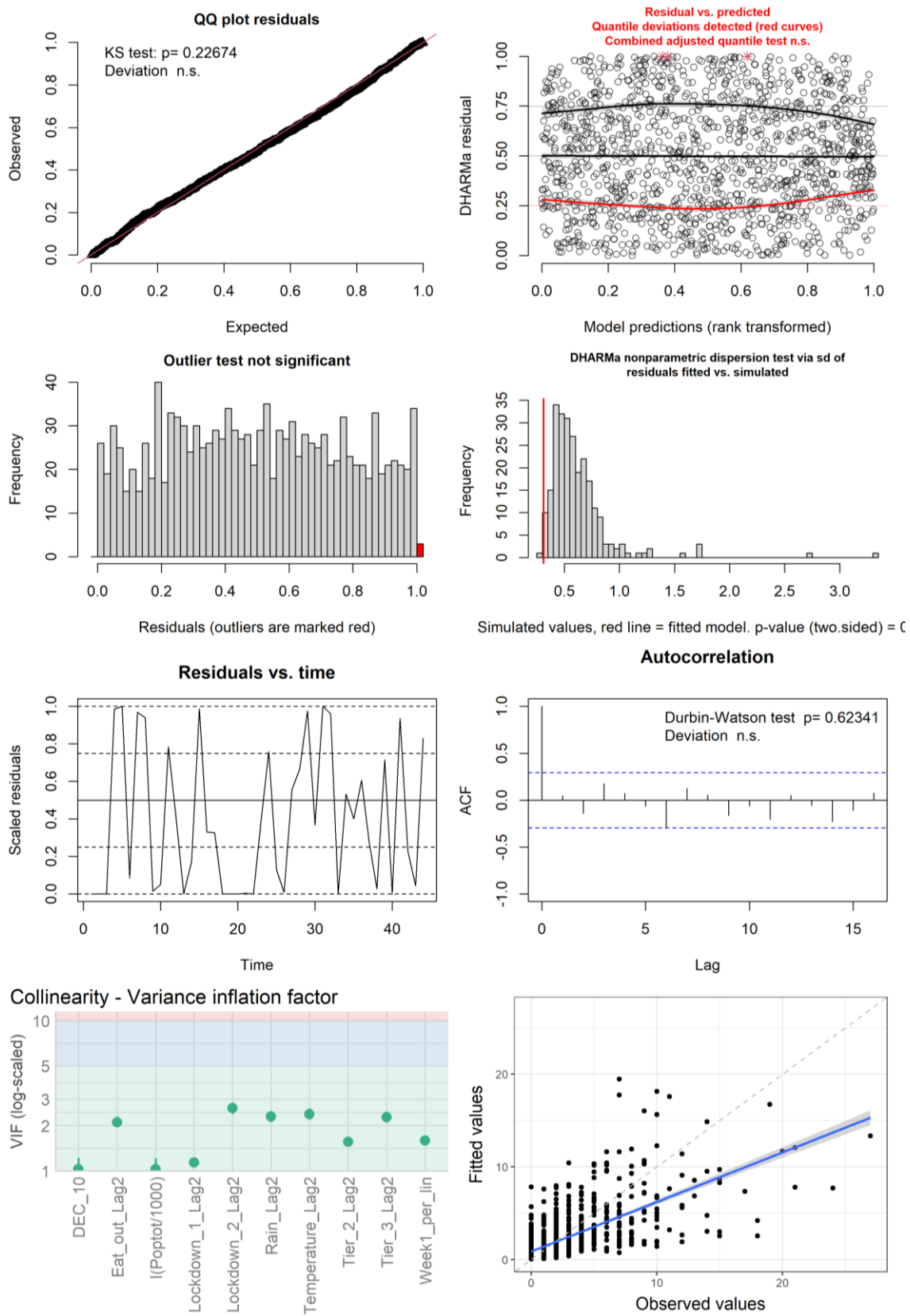
Figure S37: Figures used to assess model fit all-cases GLMM with a random gradient for week for each postcode. First row: QQ plot, residuals vs predicted. Second row: outlier check, dispersion check. Third row: residuals vs time, ACF. Bottom row: VIF, observed values vs fitted values from the model.
