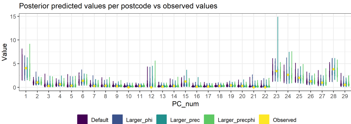
Figure S10: Figures used to assess model fit and sensitivity to hyperparameter values for the Lin10_B.1.1.119 disease mapping model, fit with the “laplace” approximation method. These plots compare the values for 4 models, each fit with different hyperparameter values (see section 2.2 above and model code in the analysis repository ( https://doi.org/10.25405/data.ncl.23815077 )). First row: density of the posterior marginals of the intercept and phi and precision hyperparameters. Second row: Mean and 97.5% quantiles for the intercept, comparison of the observed values to a sample generated from the posterior distribution. Third row: comparison of the observed values per postcode area to a sample generated from the posterior distribution (note that the numbers on the x axis do not correspond to the actual postcode numbers).
