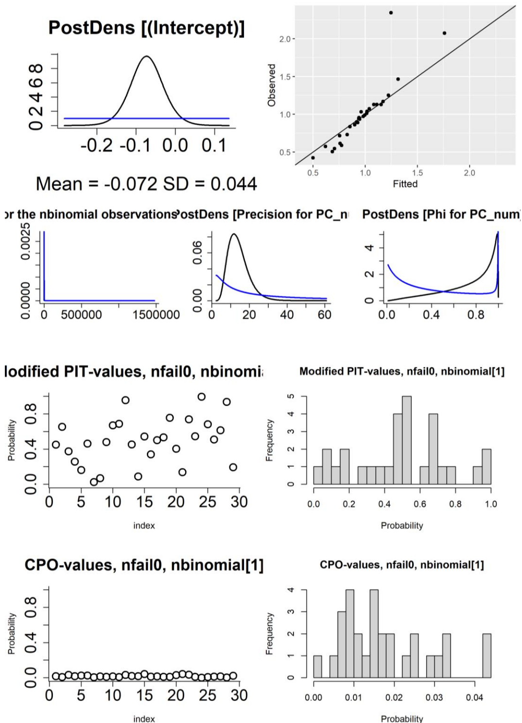
Figure S5: Figures used to assess model fit for the all-cases disease mapping model, fit with default priors and other settings. First row: density of the posterior marginals of the intercept (including prior), observed vs fitted values. Second row: posterior density (and priors) of the hyperparameters (size for the negative binomial observations, and precision and phi for the BYM2 random effect). Third row: probability integral transforms (PIT) values (modified/adjusted version appropriate for count data) per
