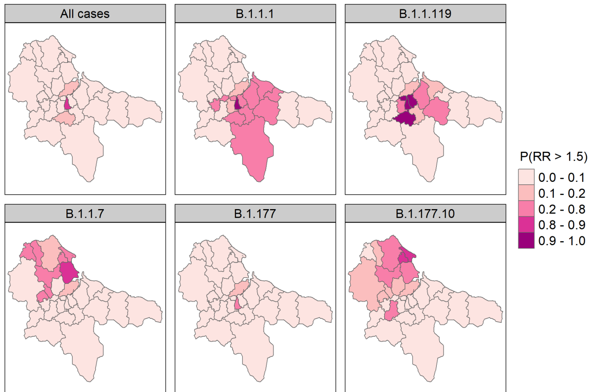
Figure S1: Map of the exceedance probabilities for relative risk threshold of 1.5. Relative risk is very likely to exceed 1.5 when probabilities are close to 1, and very unlikely when values are close to 0 (values around 0.5 have the highest uncertainty). Maps for 3 of the lineages are not shown due to poor model fit (B.1.1.309, B.1.1.315, and B.1.1.37).
