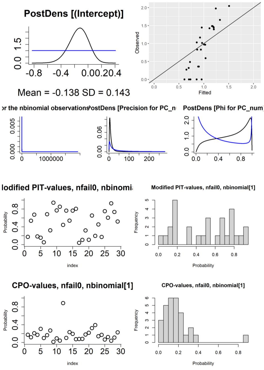
Figure S11: Figures used to assess model fit for the Lin35_B.1.1.309 disease mapping model, fit with default priors and other settings. First row: density of the posterior marginals of the intercept (including prior), observed vs fitted values. Second row: posterior density (and priors) of the hyperparameters (size for the negative binomial observations, and precision and phi for the BYM2 random effect). Third row: probability integral transforms (PIT) values (modified/adjusted version appropriate for count data) per postcode area, histogram of PIT values. Fourth row: conditional predictive ordinate (CPO) values per postcode area, histogram of CPO values.
