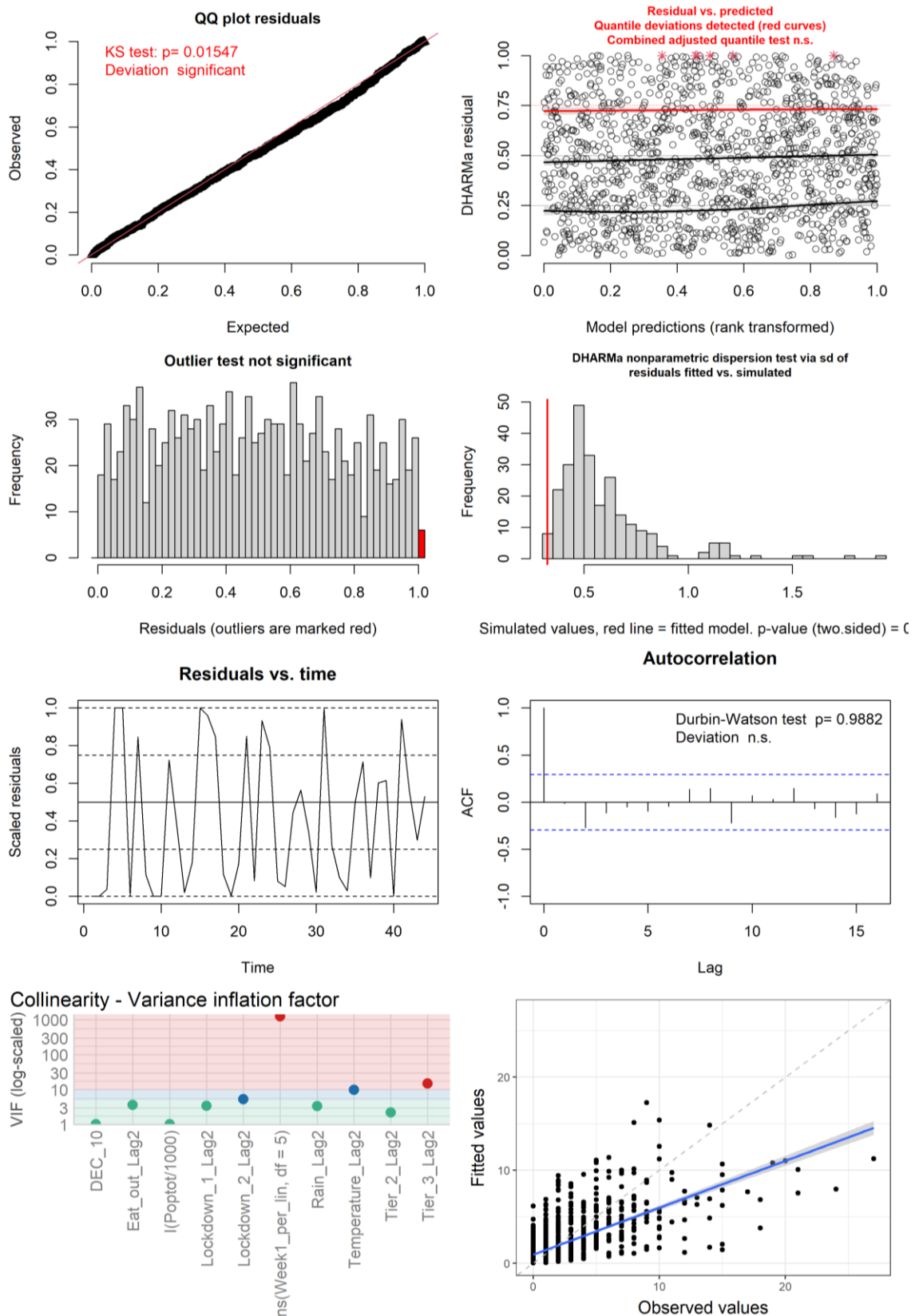
Figure S26: Figures used to assess model fit for the all-cases GLMM with a restricted cubic spline for week with 4 knots. First row: QQ plot, residuals vs predicted. Second row: outlier check, dispersion check. Third row: residuals vs time, ACF. Bottom row: VIF, observed values vs fitted values from the model.
