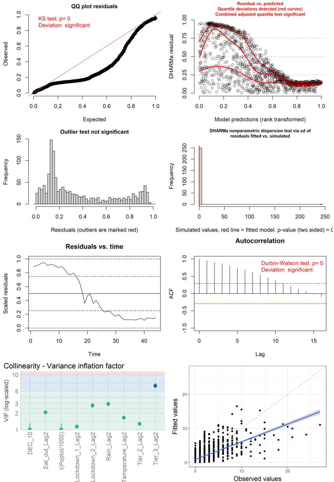
Figure S27: Figures used to assess model fit for the all-cases GLMM with a smooth spline for week. First row: QQ plot, residuals vs predicted. Second row: outlier check, dispersion check. Third row: residuals vs time, ACF. Bottom row: VIF, observed values vs fitted values from the model.
