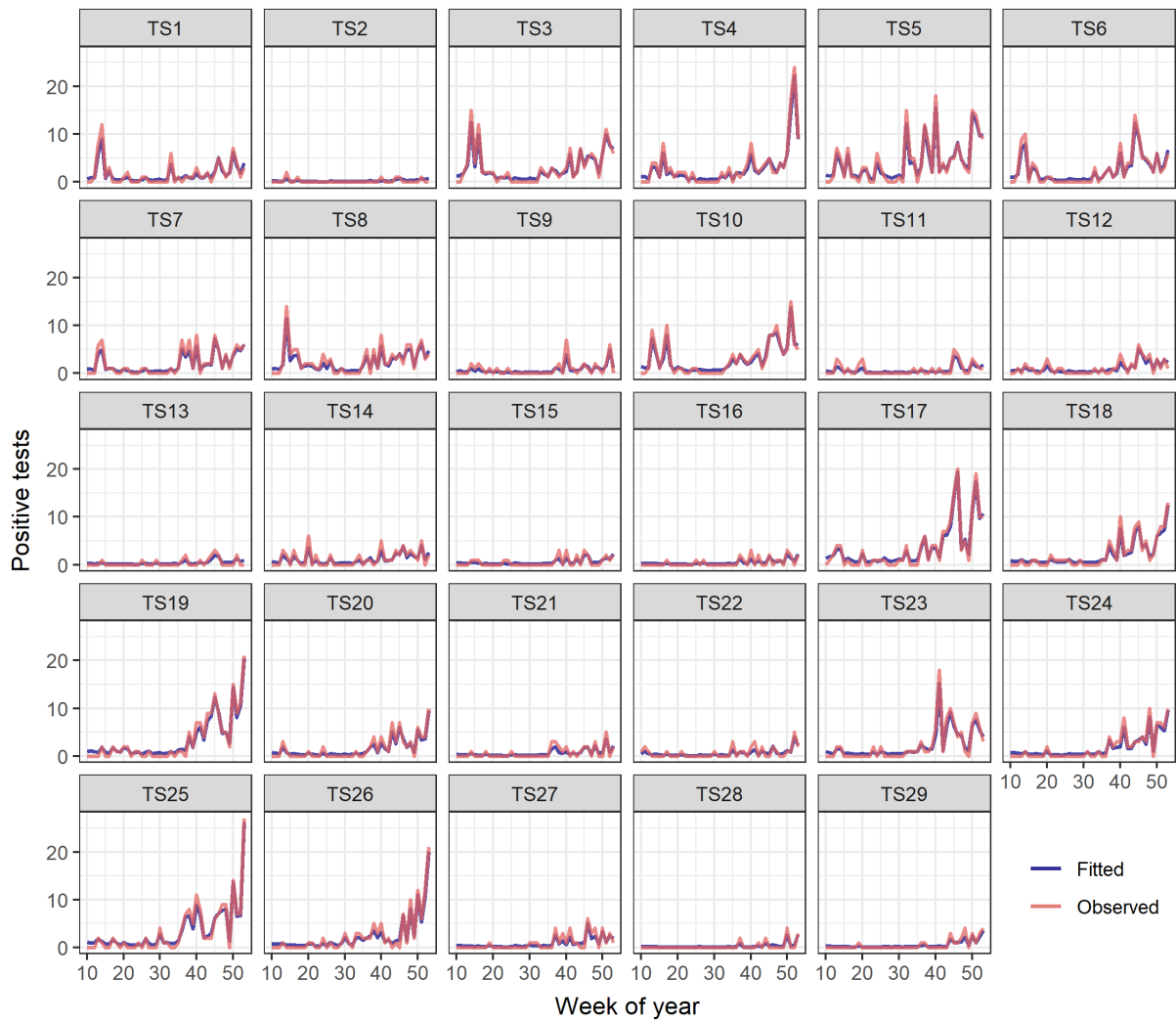
Figure S3: Predicted and observed total number of positive cases of COVID-19 (across all lineages) in Teesside during 2020. The predicted estimates (blue) are fitted values from the GLMM for all cases with an AR1 (autoregressive order 1) term for week for each postcode.
