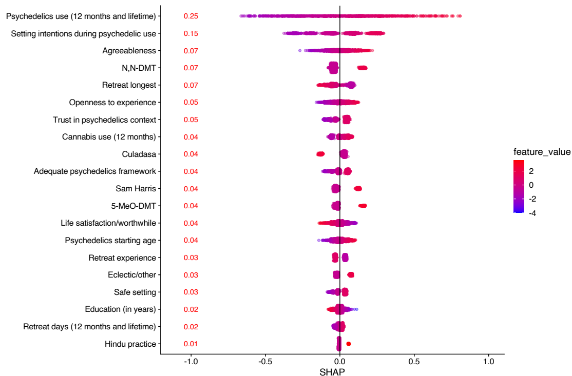
Most Important Variables in the Elastic Net Model organized by the SHAP Values
