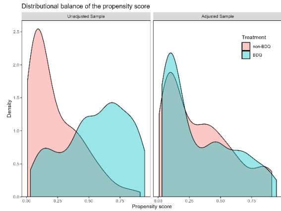
Figure 2B: Overlap plots for the complete case analysis. There is a good overlap of the propensities for being treated or not treated in both treatment groups Legend: Green hew is for patients treated with bedaquiline-containing regimens and red hew is for patients treated with non-bedaquiline-containing regimen
