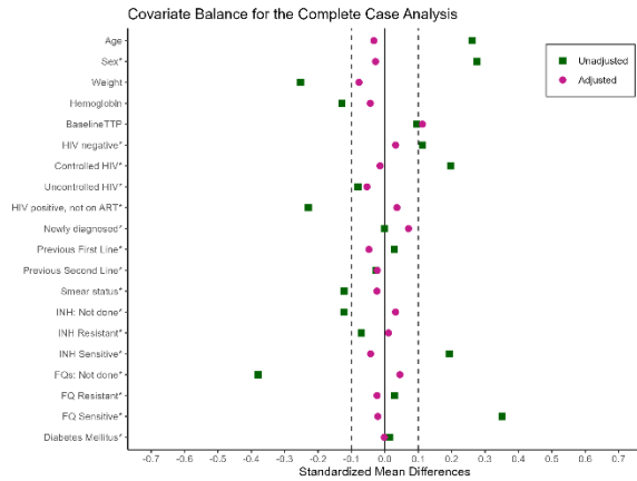
Figure 2A: Covariate balance for the complete case. This illustrates graphically that conditional exchangeability was achieved. Definition of Abbreviations: Baseline TTP = Baseline Time to culture positivity, HIV = Human Immunodeficiency Virus, ART = Antiretroviral Therapy, INH = Isoniazid, FQ = Fluoroquinolones.
