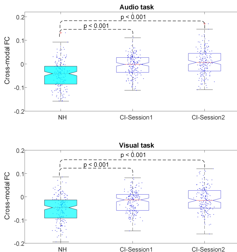
Figure 9: Comparison of the distribution of average task-induced CMFC across subjects for NH and CI groups. CI users exhibit significantly higher task-related CMFC values compared to the NH group (p-values represent the significance of the two-group comparison in each recording session). Dashed lines indicate two-group comparisons.
