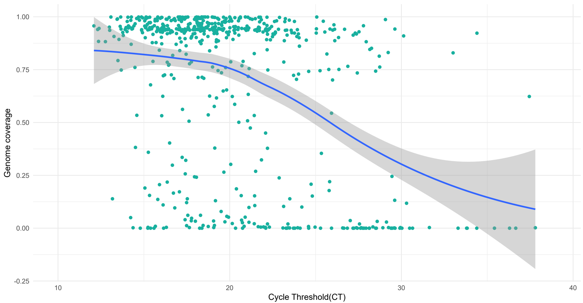
Figure S1 : Scatterplot of genome called coverage vs PCR Cycle threshold
