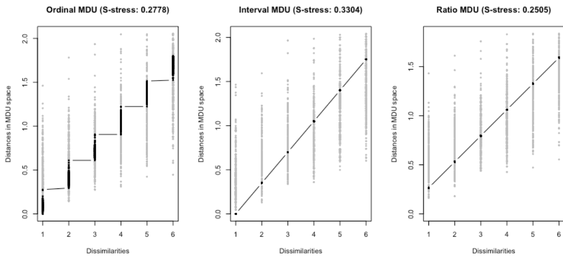
Figure S2. Shepard diagrams for ordinal MDU, interval MDU, and ratio MDU solutions
