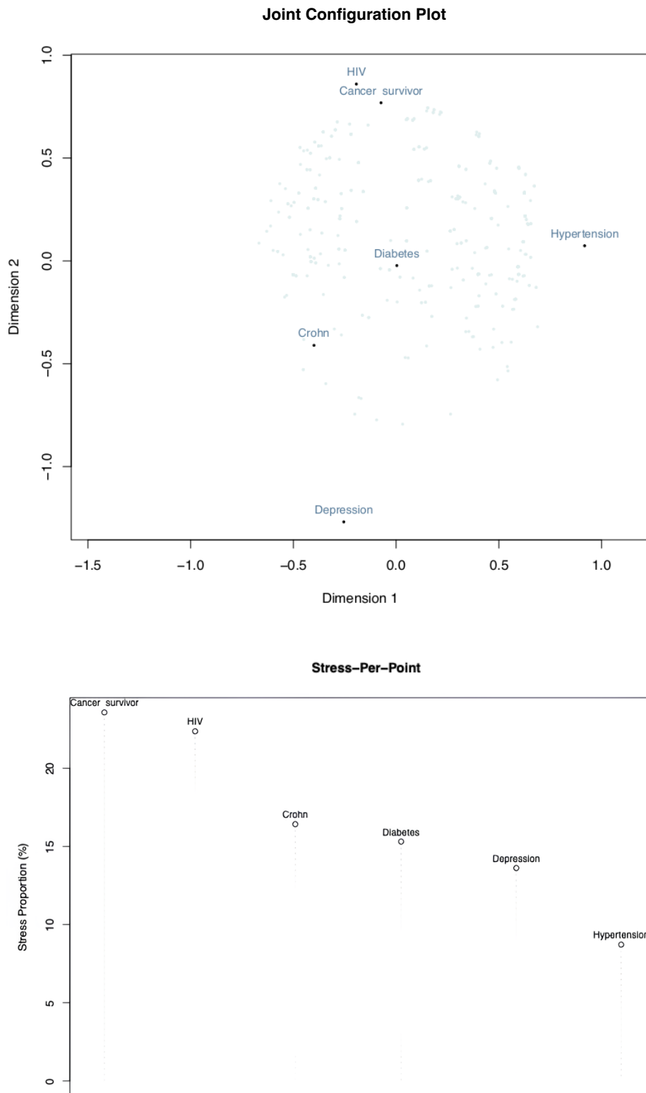
Figure S3. Top: Two-dimensional unfolding ordinal solution plot of individuals (light dots) and objects (dark dots). Bottom: Stress Per Point diagram illustrating the contribution of each object to the overall stress of the solution.
