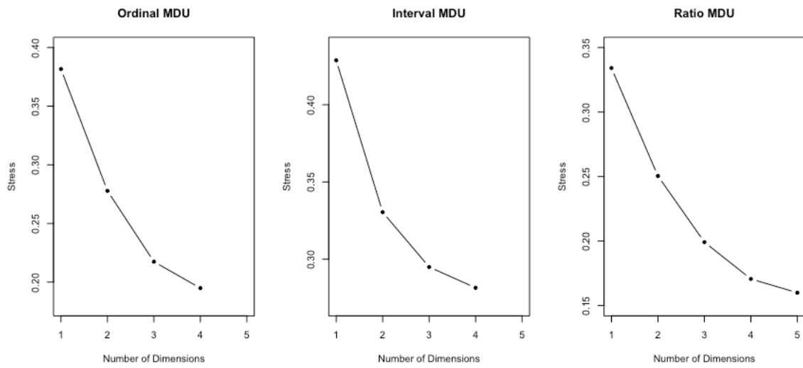
Figure S1. Scree plots for ordinal MDU, interval MDU, and ratio MDU solutions
