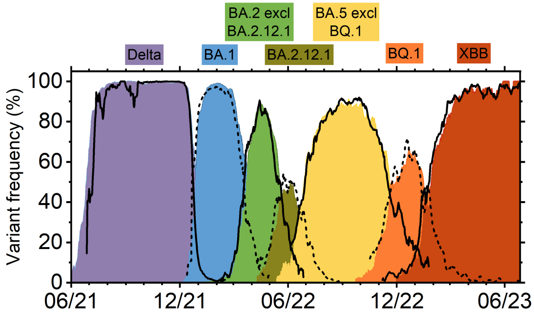
Figure S2. Variant frequency data with clinical data submitted by “Lab A” from March 21 to April 2, 2022, omitted. The 7-day simple moving average of the frequency of individual variants in clinical sequences collected in Minnesota is shown as consolidated colored bars, vs time. The 7-day simple moving average of the frequency of individual variants in Metro Plant influent is shown in solid or dashed black lines, vs time. Variants are labeled across the top.
