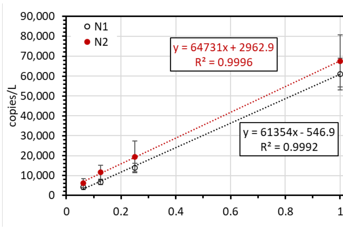
Figure S1. Dilution series results showing the average N1 and N2 concentrations (n=8) at each dilution level.
