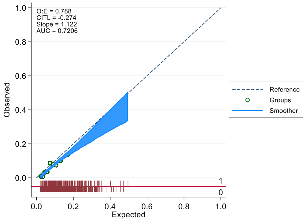
Figure S7: Calibration plot of the PREPARE hypoxemia clinical prediction model in the validation dataset when including wheezing as a candidate predictor
