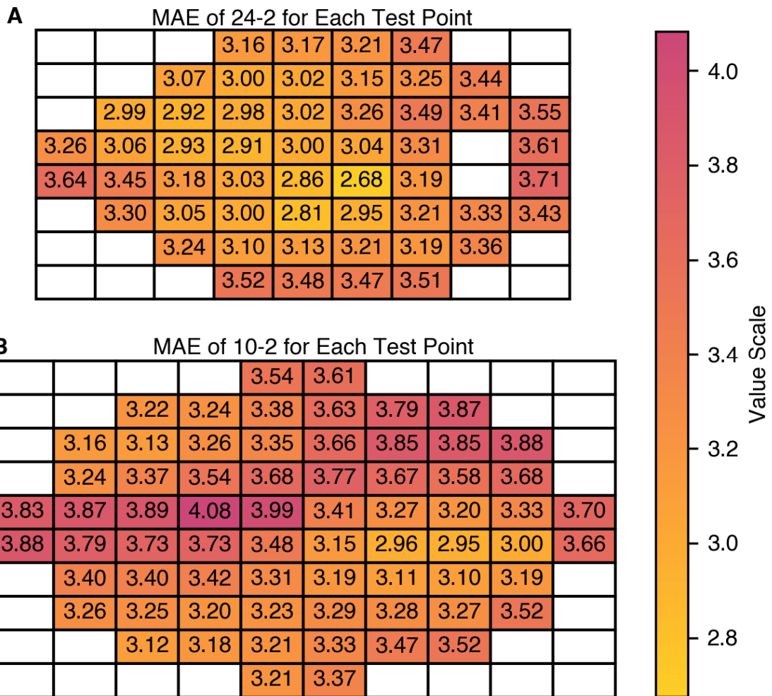
2 Figure S7. Heatmaps of the MAEs for each test point. (A) 24-2 test pattern, (B) 10-2 test pattern. The 3 color scale represents the magnitude of the MAE at each test point, revealing the spatial distribution 4 of estimation accuracy across the VF for both test patterns. We horizontally flipped the left eye data 5 and integrated them with the right eye data. For the 24-2 pattern, MAEs are generally consistent 6 across most VFs, with slight increases in peripheral areas beyond the OCT scan range and regions 7 surrounding the physiological blind spot. The 10-2 pattern shows a relatively stable distribution of 8 MAEs, with a modest increase in the central nasal area. 9 MAE = mean absolute error; VF = visual field; OCT = optical coherence tomography.
