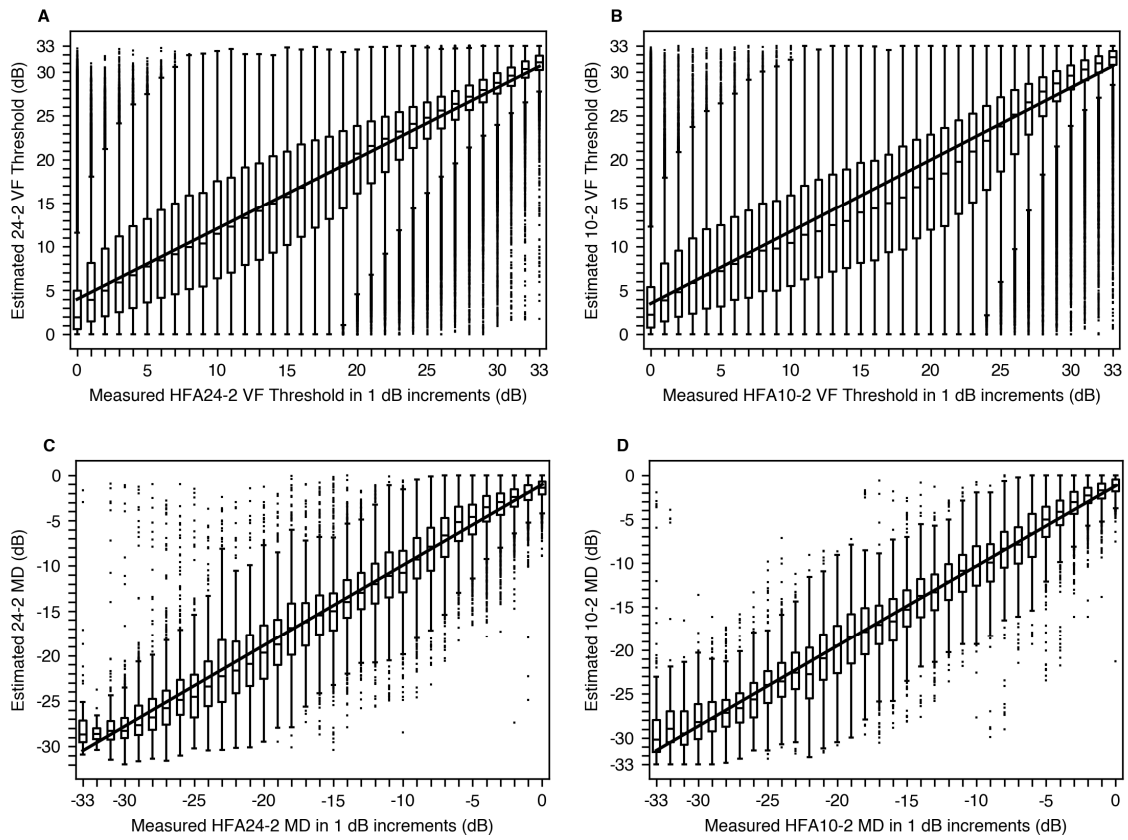
2 Figure S3. Correlations between measured and estimated VF parameters. (A) 24-2 VF threshold 3 (pointwise values, Pearson's r = 0.893 ), (B) 10-2 VF threshold (pointwise values, Pearson's r = 0.902 ), 4 (C) 24-2 MD (Pearson's r = 0.932 ), and (D) 10-2 MD (Pearson's r = 0.945 ). Each panel displays 5 boxplots of estimated values for each measured value increment and a regression line. All correlations 6 are significant at p < 0.001 . 7 VF = visual field; MD = mean deviation.
