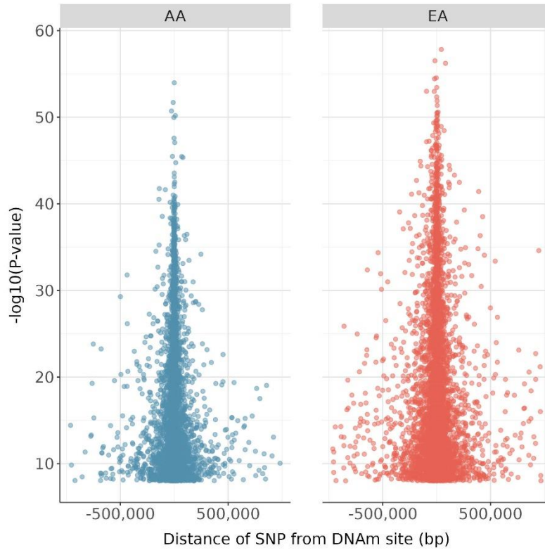
Supplementary Fig.1: Relationship between p-values and the distance from SNP to DNAm site in the AA and EA populations. The scatter plots depict the association between the distance from the SNP to the DNAm site (measured in base pairs, bp) and the corresponding -\log_{10}(\text{p-values}) for the detected meQTLs in the AA (left panel) and EA (right panel) populations. Higher values indicate more significant meQTL associations.
