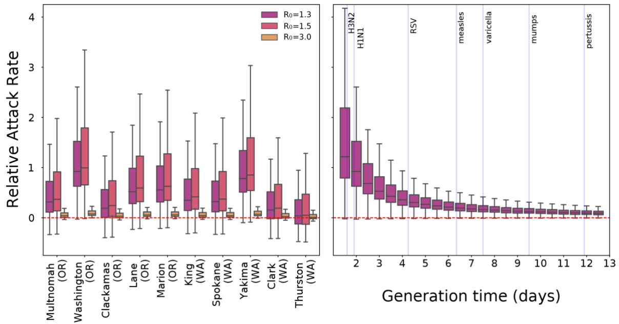
Figure S1: Left: Relative variation in attack for the selected affected counties under different infective scenarios: R_0 = 1.3 , R_0 = 1.5 , R_0 = 3.0 . Right: Exploration of the relative variation in attack rate (Washington county, OR) for different values of the generation time and a fixed R_0 = 1.3 . Blue vertical lines indicate the average generation time of different airborne respiratory diseases.
