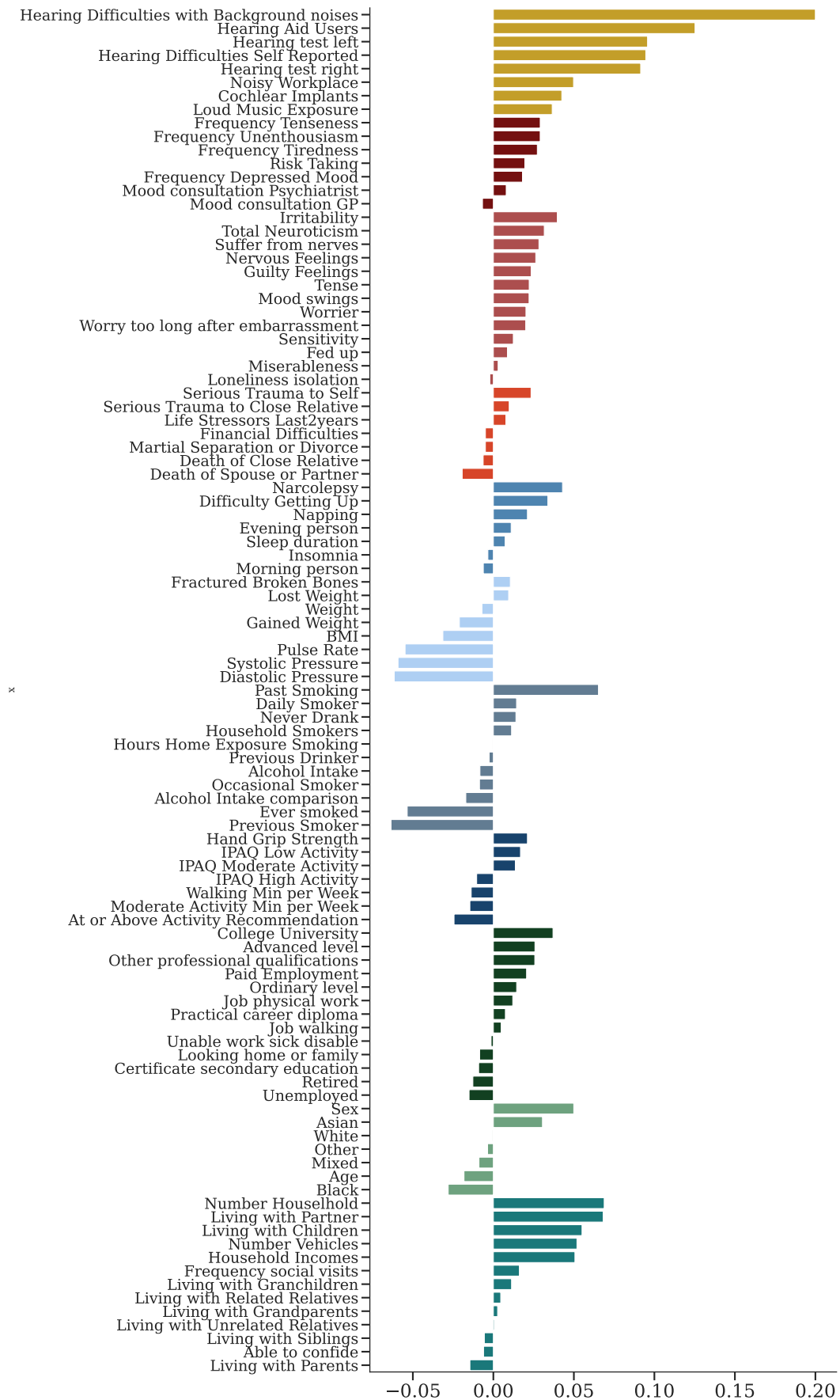
Figure A2: Features loads (Pearson's r correlation coefficient between features and the models' scores) of the Presence Risk Score model
