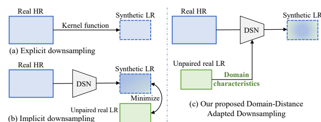
Fig. 1. Synthesizing downsampled LR images from the real HR and unpaired real LR datasets. (a) shows the explicit down-sampling. (b) shows the conventional implicit down-sampling, which proposes minimizing the distance between synthetic and real LR images. (c) shows our proposed domain-distance adapted down-sampling method, in which real LR domain characteristics were embedded into the down-sampling process to facilitate the domain translation.
