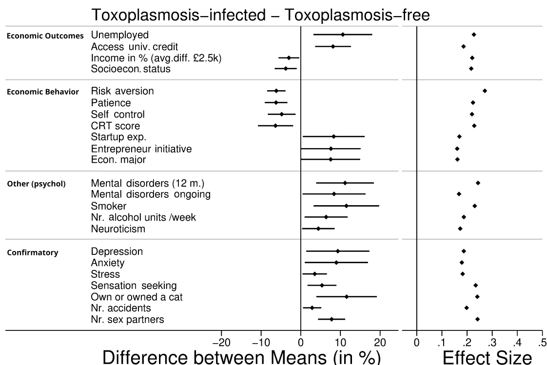
Figure 4: Differences between RhD-negative participants classified as infected and non-infected by the RT-method in a representative UK survey ( N = 2,020 ). We report differences between the means of the two groups (with 95% confidence intervals) and effect sizes. The upper-most part of the figure presents results on economic outcomes. The second block reports results on economic behavior. The third presents new results on mental health and addiction. As an additional validation of the method, the lower part confirms previously-reported effects of Toxoplasmosis while using our imputed classification.
