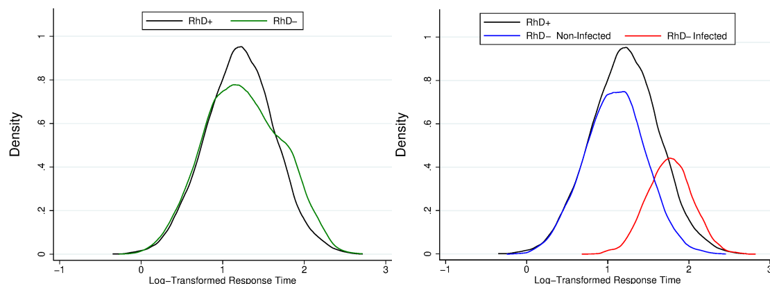
Figure 3: Left: Empirical distribution of log-transformed response times for the survey study ( N = 2,020 ) depending on blood type. Right: Applying a finite-mixture method, we recover the distributions for (imputed) infected and non-infected within the RhD-negative population, and estimate the extent of the infection at 18.32%.
