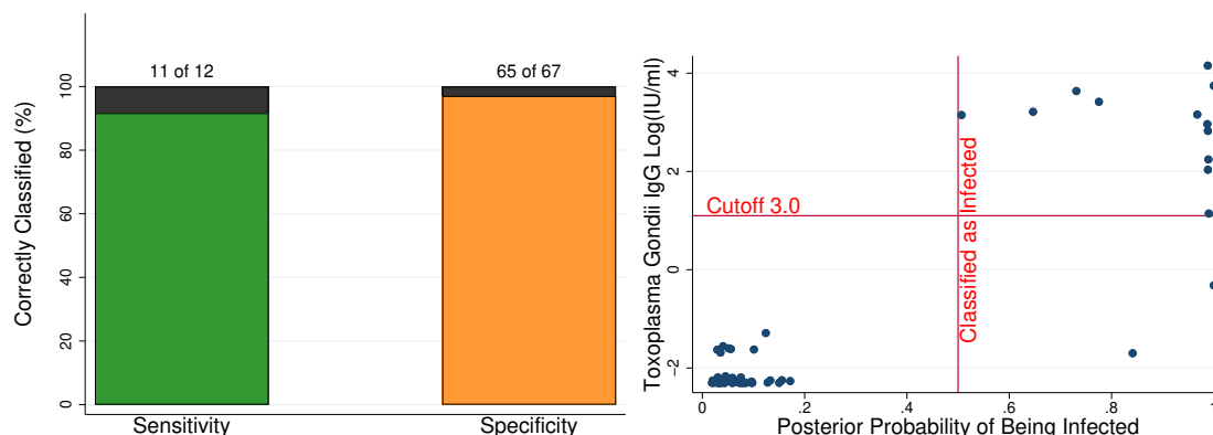
Figure 2: Left-hand panel: The proposed method, which uses only response times and is cheaper and easier to deploy at large scale than antibodies tests, presents high sensitivity (91.66%) and specificity (97.01%). Right-hand panel: The posterior probability of each participant being classified as infected by the proposed method is highly correlated with the individual proportion of Toxoplasma gondii IgG antibodies (log-transformed for ease of representation, Pearson’s \rho = 0.7125, p < 0.0001 ).
