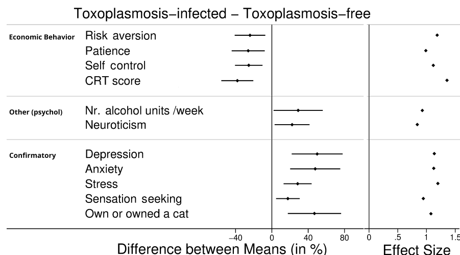
Figure 5: Differences between Toxoplasmosis-infected and Toxoplasmosis-free subjects in the clinical study ( N = 79 ), where infection status is based on Toxoplasma IgG seroprevalence. We report differences between the means of the two groups (with 95% confidence intervals) and effect sizes (means difference divided by standard deviations). The upper part of the figure presents results on economic behavior. The middle part reports new results on mental health and addiction. The lower part confirms previously-reported effects of Toxoplasmosis.
