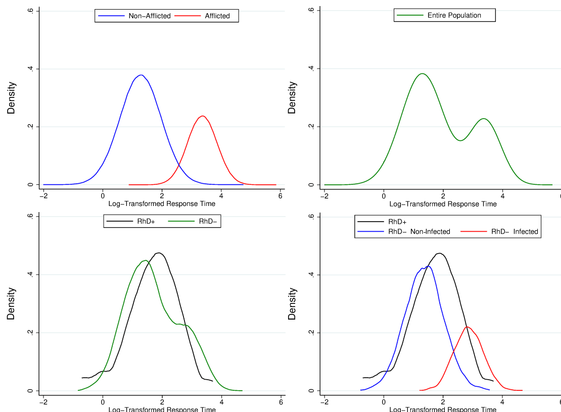
Figure 1: If afflicted individuals in a population show a systematic reaction slow-down, the distribution of their log-transformed response times is shifted compared to the non-afflicted (top-left panel). The distribution for the entire population is then a mixture showing a bimodal pattern (top-right panel). Consistent with the expected effects of Toxoplasmosis infection, we find this pattern in our clinical study for RhD-negative individuals, but not for RhD-positives (bottom-left panel). Applying finite-mixture models to the data, we recover the subgroup distributions and their relative sizes (bottom-right panel). This delivers an estimate of the extent of the infection in the population and also individual-level infection probabilities.
