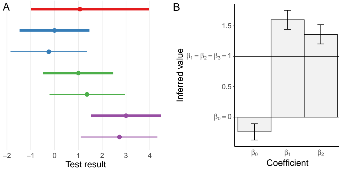
Figure S3: Inferences of a linear model of test results from 100 simulated observations when an interaction term is unaccounted for. There are two binary features, x_1 and x_2 , both with 50% prevalence. The model is y = \beta_0 + \beta_1 x_1 + \beta_2 x_2 + \epsilon but there is in truth an additional interaction term \beta_3 x_1 x_2 . The true coefficients are \beta_0 = 0 and \beta_1 = \beta_2 = \beta_3 = 1 , and the error is \epsilon \sim \text{Normal}(0, 3/4) . (A) 95% central intervals of true (bold lines) and posterior predictive distributions (thin lines) of results in the population (red) as features are conditioned on: x_1 = x_2 = 0 (blue), x_1 = 1 and x_2 = 0 (green), and x_1 = x_2 = 1 (purple). Points represent medians. (B) Mean posterior coefficient estimates with standard errors.
