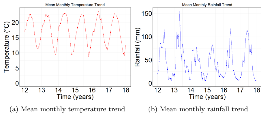
Fig. A1: Mean monthly temperature and rainfall trends used to simulate the models for a period of 6 years from year 12 to 18.
