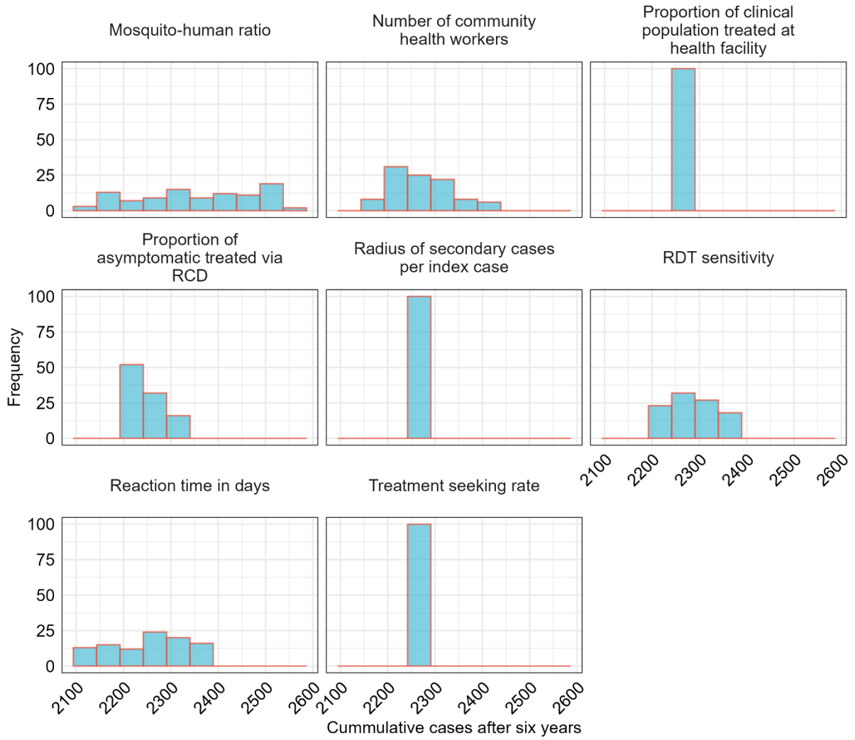
Figure 2: Cumulative malaria cases observed after varying intervention related parameters. The parameter ranges considered are highlighted in manuscript 1.
