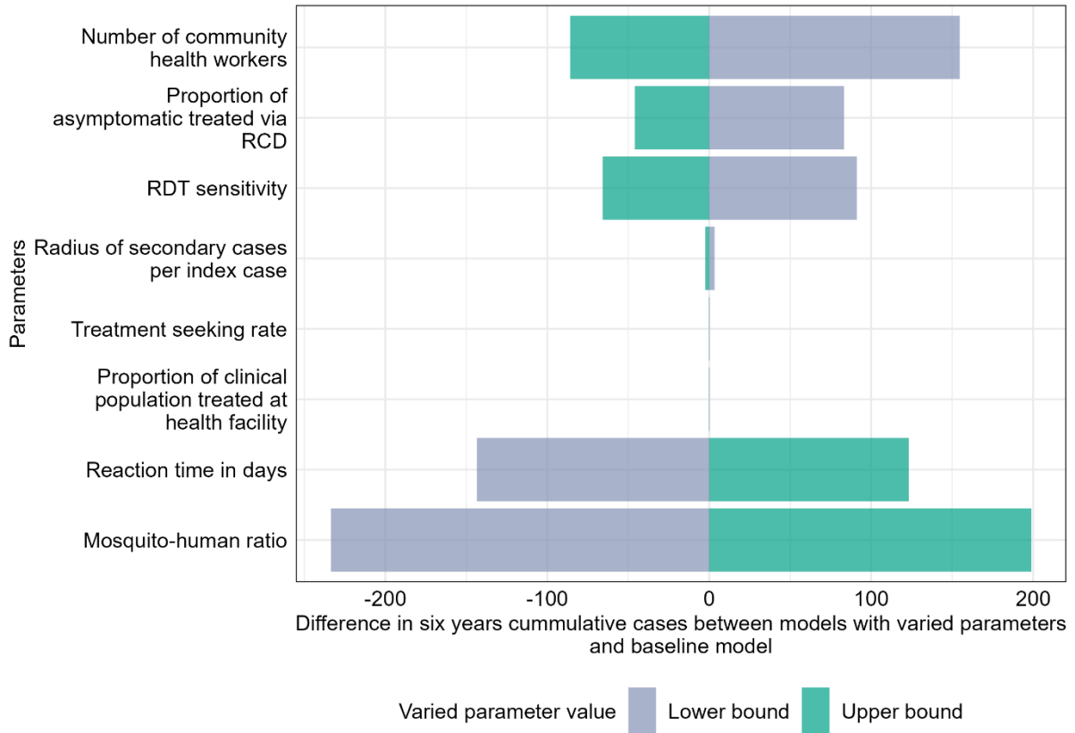
Figure 6: Difference in cumulative cases after six years between the model with baseline (central)
