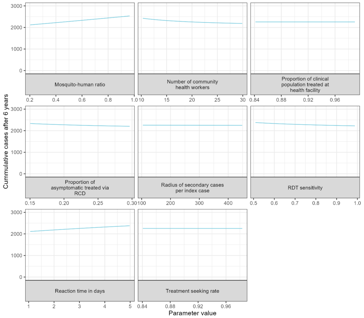
Figure 4: Relationship between cumulative malaria cases observed after varying intervention related parameters and random values between their ranges. The parameter ranges considered are highlighted in manuscript 1.
