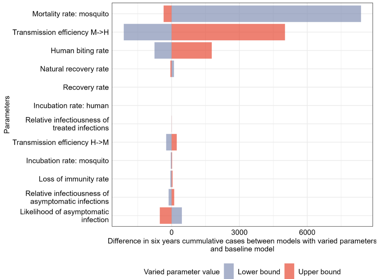
Figure 5: The difference in cumulative cases after six years between the model with baseline (central)
