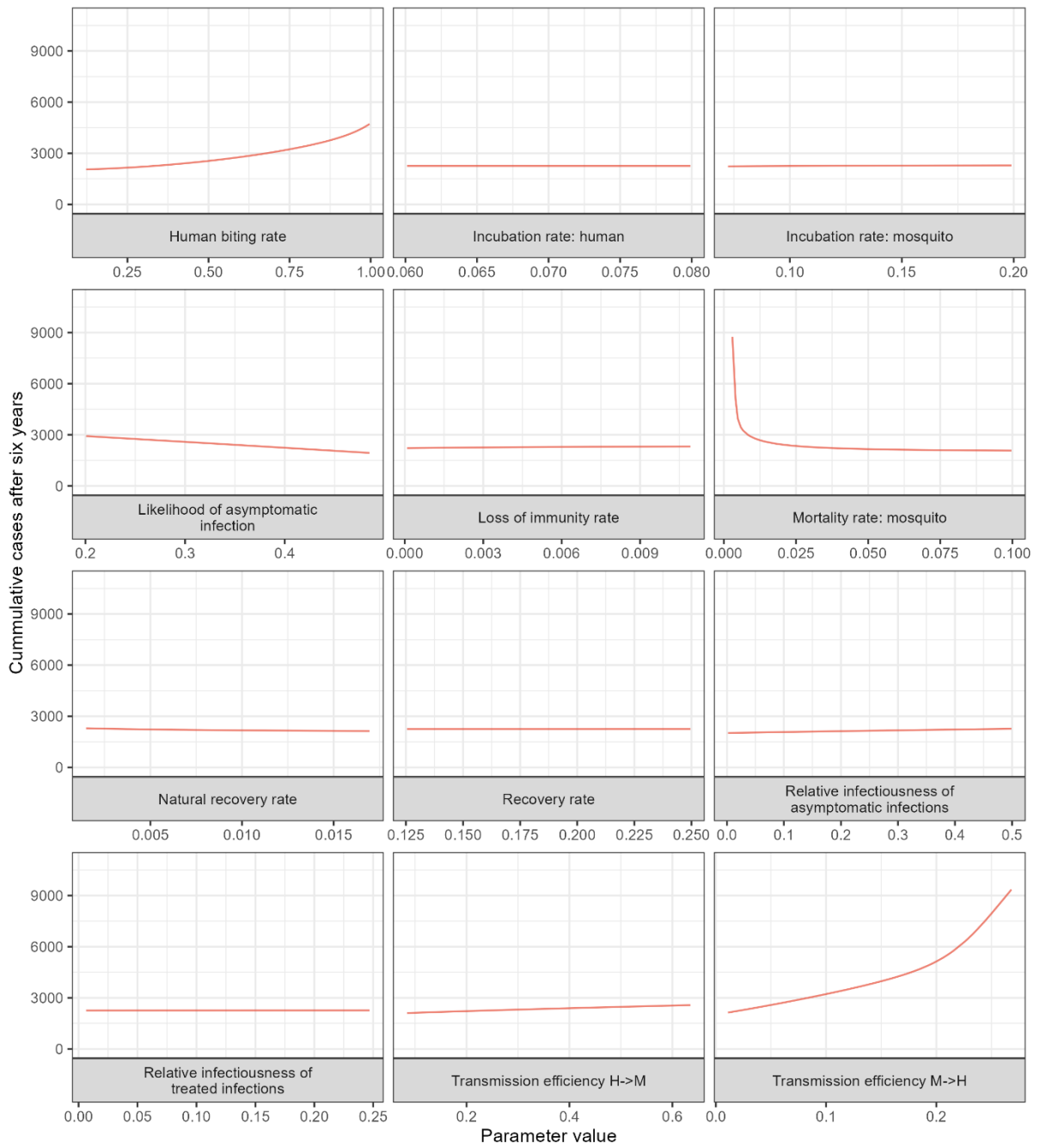
Figure 3: Relationship between cumulative malaria cases observed after varying non-intervention related parameters and random values between their ranges. The parameter ranges considered are highlighted in manuscript 1.
