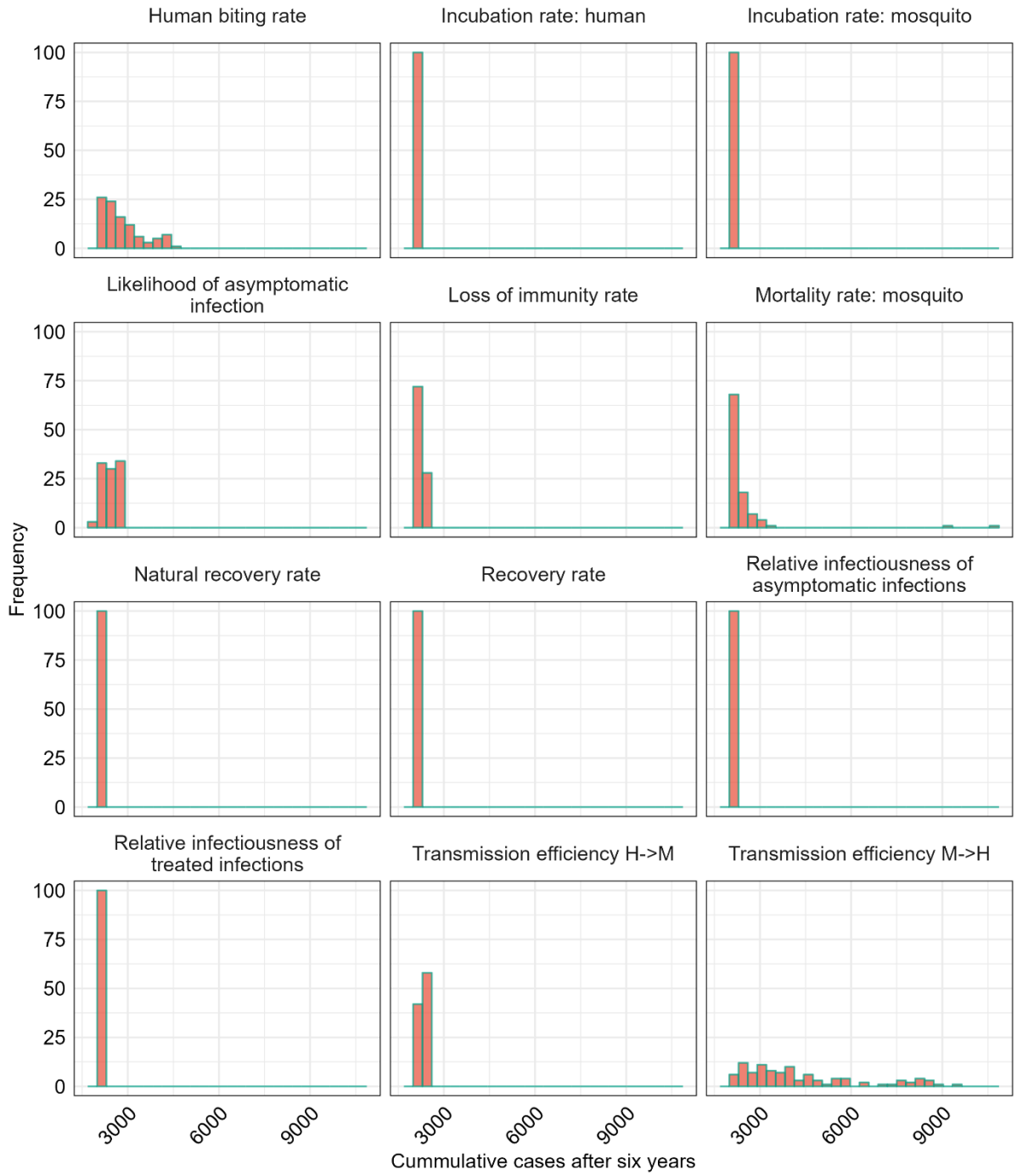
Figure 1: Cumulative malaria cases observed after varying non-intervention related parameters. The parameter ranges considered are highlighted in manuscript Table 1.
