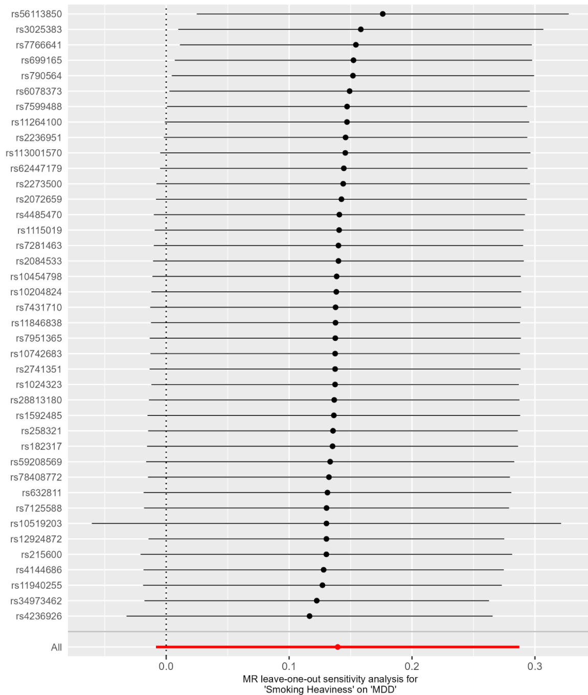
Supplementary Figure S12. Leave-one-out IVW regression analyses of liability to smoking heaviness on MDD risk.
