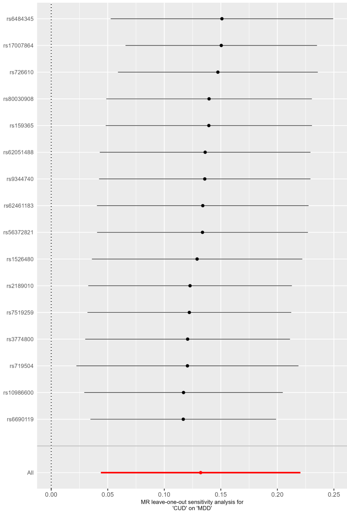
Supplementary Figure S14. Leave-one-out IVW regression analyses of liability to CUD on MDD risk.
