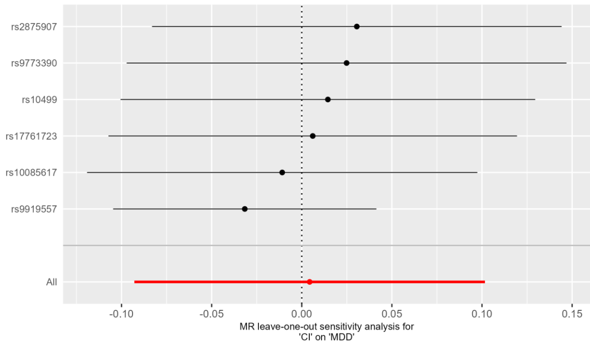
Supplementary Figure S13. Leave-one-out IVW regression analyses of liability to cannabis initiation on MDD risk.
